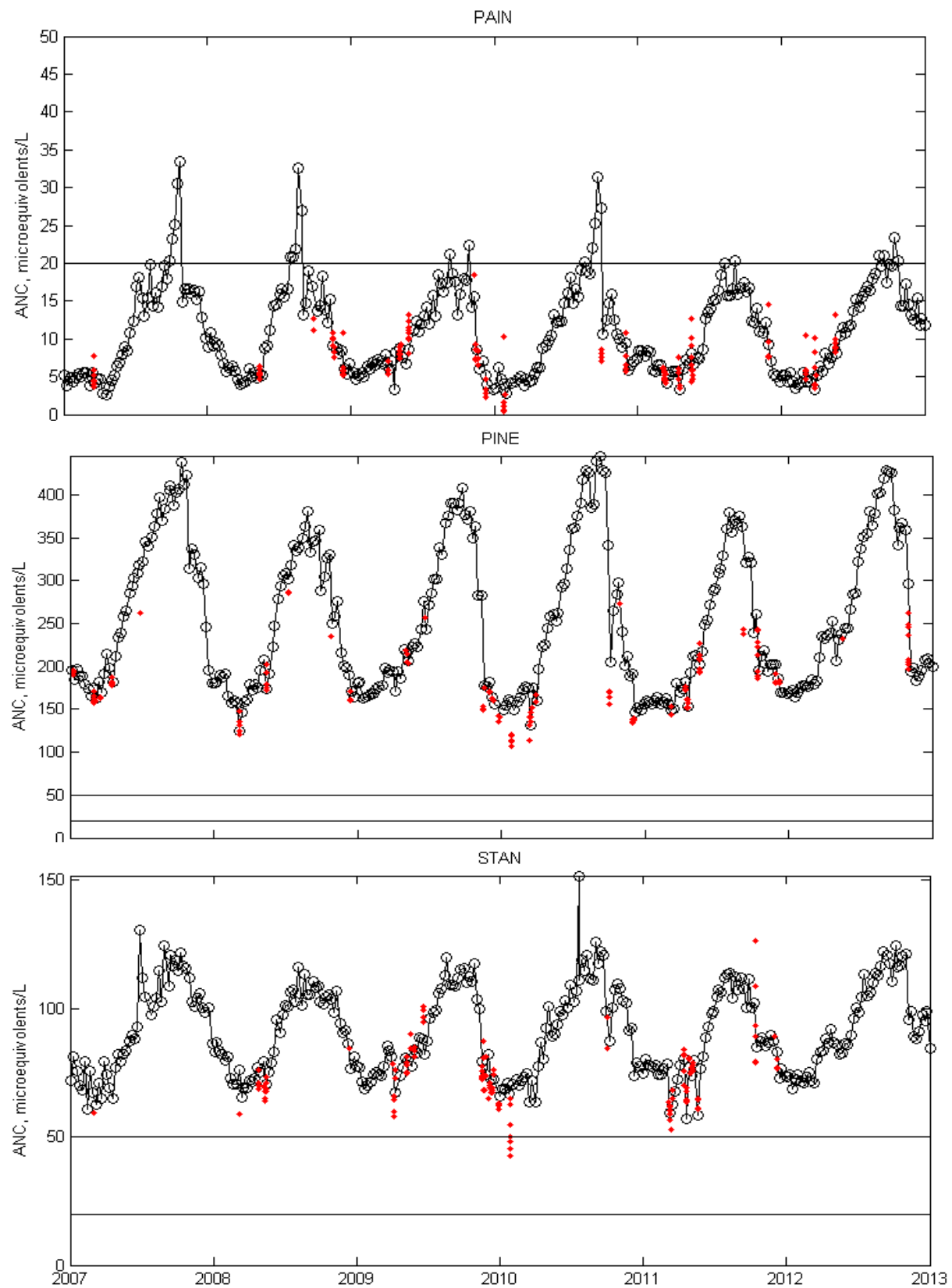
Figure 2. ANC values for grab (black) and automated episodic (red) samples in 2006-2012.
