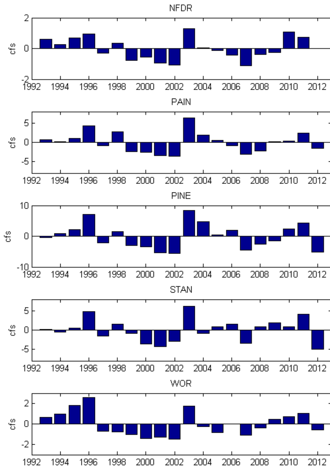
Figure 4. Inter-annual variation in discharge around the long-term mean (1993-2012) discharge for gauged streams in SHEN. NFDR gauge was discontinued in 2011.
