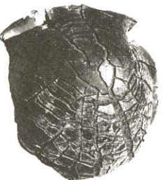
"Bombs," or ejected lava blobs.
