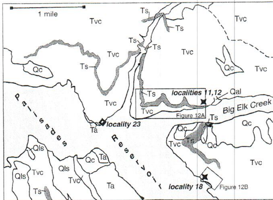
Figure 11. Modified geologic map showing relationship of detachment slide blocks (Ts) with Tertiary volcaniclastic sediments (Tvc) at Palisades Reservoir (see Fig. 1; from Oriel and Moore, 1985). The slide blocks are limestone of the Mississippian Mission Canyon Formation that slid from the Snake Range into a basin accumulating Miocene volcaniclastic sediments. Isotopic ages from ashes bounding the slide blocks provide precise limits for the age of deformation as described in the text. Other symbols on map include Quaternary colluvium (Qc), Quaternary alluvium (Qal), Quaternary landslide deposits (Qls), and Tertiary andesite (Ta). Locality 14 is ~2 km southeast of locality 18. Locations of Figures 12A and 12B are also shown. Sample location sites from Table 1 are shown.
