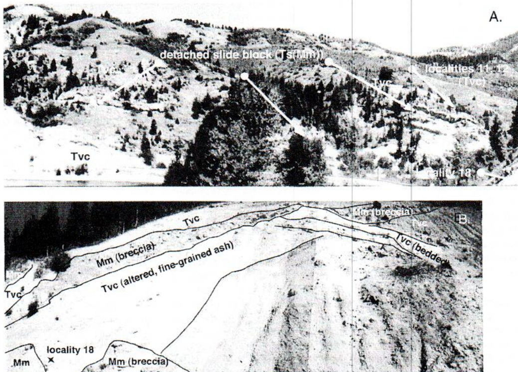
Figure 12. (A) Photo of slide block (Ts) bounded by Miocene volcaniclastic sediments along east side of Palisades Reservoir. Localities 11, 12, and 18 are also shown. Locality 14 is ~2 km southeast of locality 18. See Figure 11 for location of photo. (B) Photo of chaotic breccia. Symbols include Tertiary volcaniclastic sediments (Tvc), Tertiary slide blocks (Ts), and Mississippian Mission Canyon Formation (Mm).
