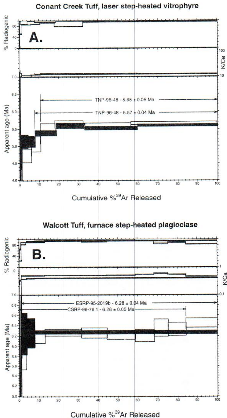
Figure 6. Age spectra for step-heated bulk samples. (A) Results from step-heated vitrophyre from the Conant Creek Tuff. (B) Results from furnace step-heated plagioclase from the Walcott Tuff.
