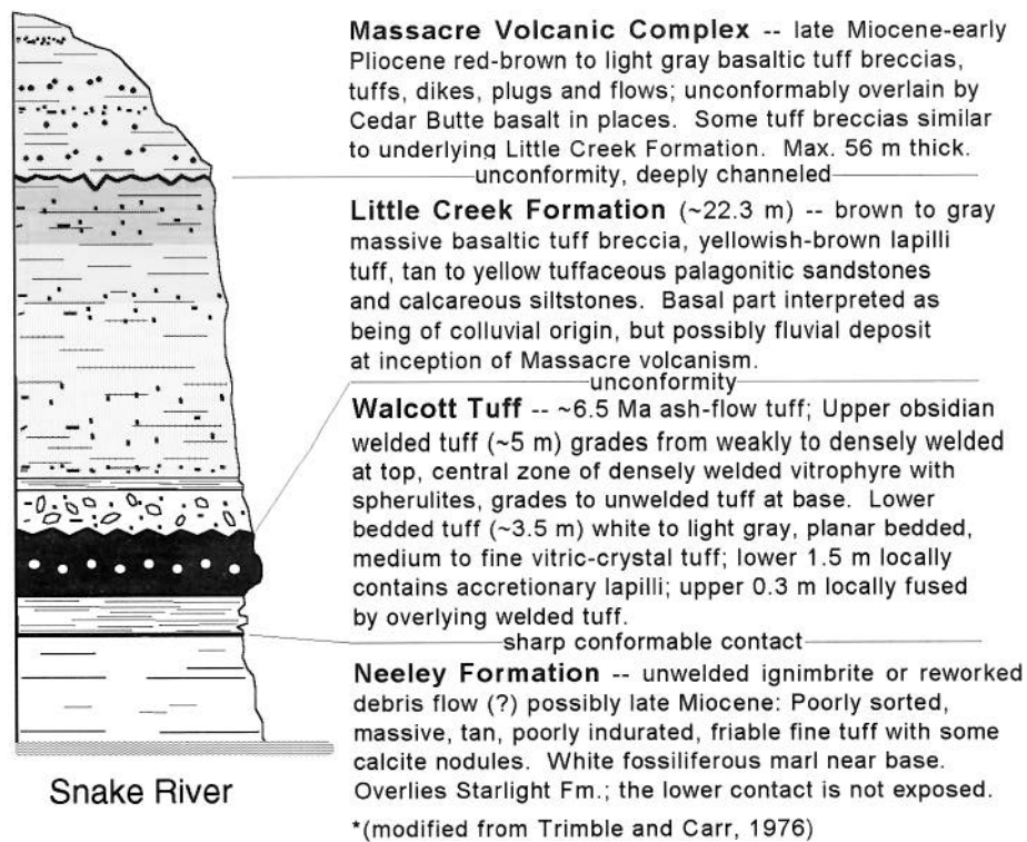
Figure 30. Geologic section at Stop 12C (access from interstate highway rest area near Massacre Rocks) illustrating sequence observed along the Snake River. Refer to Figure 29 for location of this and other stops in the Massacre Volcanic Complex. Adapted from Trimble and Carr (1976).
