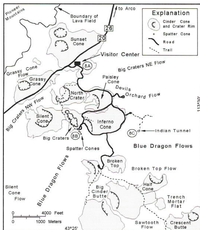
Figure 20. Index map of the Craters of the Moon National Monument area (adapted from Kuntz, 1989) showing tephra cones and general locations of major lava flows. Field trip Stops 8A-8C are only a few of the numerous places in the monument where fresh volcanic features can be observed.
