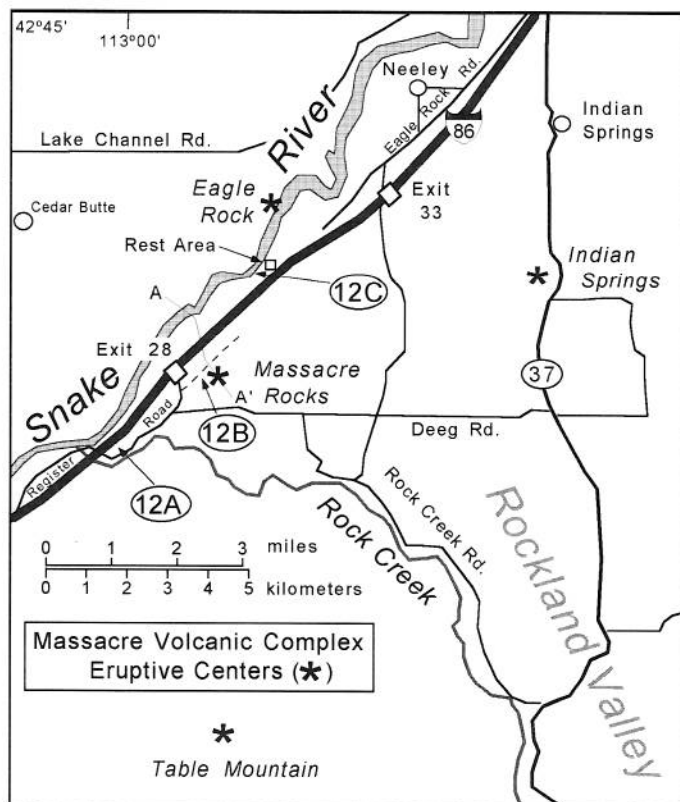
Figure 29. Map of the Massacre Rocks area with eruptive centers of the Massacre Volcanic Complex. Phreatomagmatic units of the Massacre Complex were overlain by Quaternary basalts that flowed north from eruptive centers in Rockland Valley. Field trip stops (12A - 12C) are circled.
