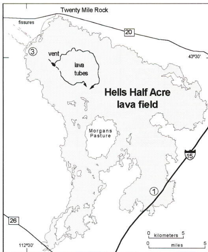
Figure 11. Map of the Hells Half Acre basaltic lava field with Stops 1 and 3 shown in circled numbers. The lava field exemplifies monogenetic Holocene shield eruptions and inflationary lava flow emplacement on the eastern Snake River Plain. Arrows denote path of lava tube feeders.
