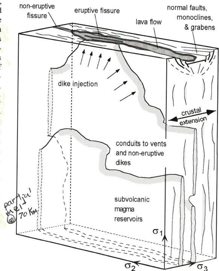
Figure 7. Schematic model of dike emplacement on the eastern Snake River Plain and the relation to surface deformational features. Propagation is possible when the fracture toughness of the country rock is exceeded by magma pressure. Orientation of dikes and vertical reservoirs are controlled by the regional stress field. Adapted from Rubin and Pollard, 1987; Kuntz, 1992; and Hackett and Smith, 1992.
