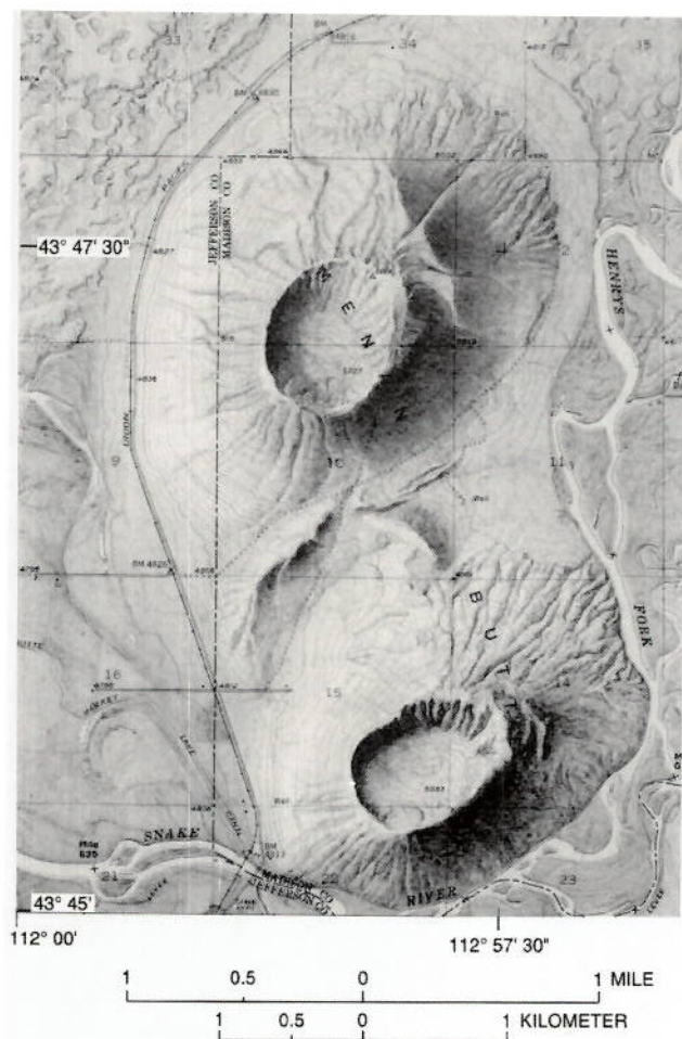
Figure 9. Portion of the Menan Buttes, Idaho shaded relief map (U.S. Geological Survey, 1951, 1:24,000 scale shaded topographic map) with large tuff cones. Phreatomagmatic eruptions occurred near the confluence of the Henrys Fork and the South Fork of the Snake River.
