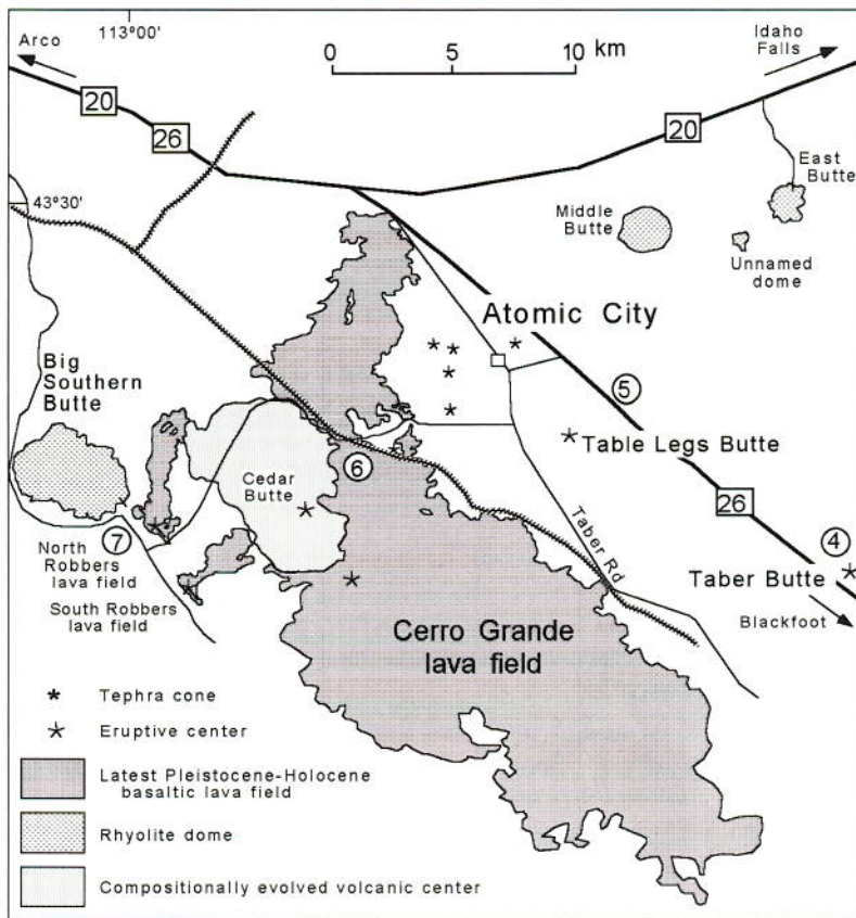
Figure 14. Detailed index map of the Cerro Grande lava field, North and South Robbers lava fields, and other features along the axial volcanic zone, adapted from Kuntz et al. (1992), aerial photographs and field investigations. Field trip stops are shown in circled numbers. See text for explanation and road guide to Stops 4-7.
