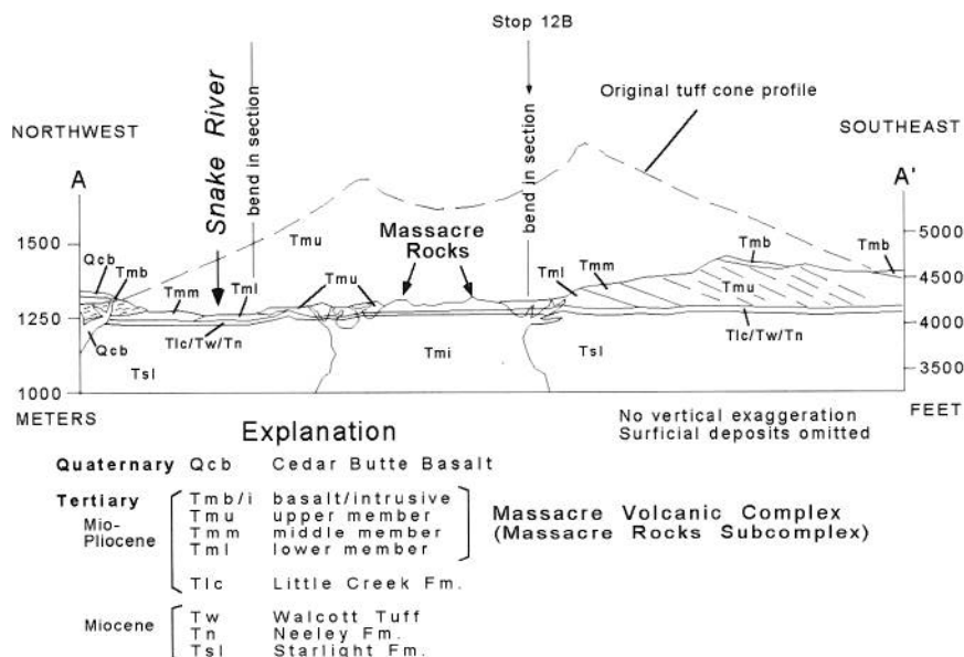
Figure 31. Geologic cross-section of the Massacre Volcanic Complex (after Luessen, 1987) through the Massacre Rocks eruptive center. Refer to Figure 29 for the location of the A-A' cross-section line.
