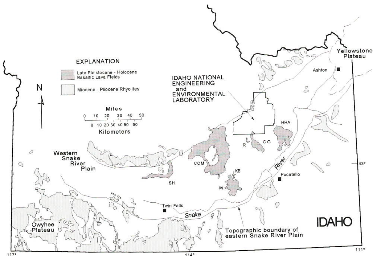
Figure 2. Map of southern Idaho with the locations of Owyhee Plateau, Yellowstone Plateau, Idaho National Engineering and Environmental Laboratory (INEEL), latest Pleistocene-Holocene basaltic lava fields (dark shading), and major outcrops of Miocene-Pliocene rhyolites. Abbreviations for lava fields are: SH = Shoshone, COM = Craters of the Moon, W = Wapi, KB = Kings Bowl, R = North and South Robbers, CG = Cerro Grande, and HHA = Hells Half Acre.
