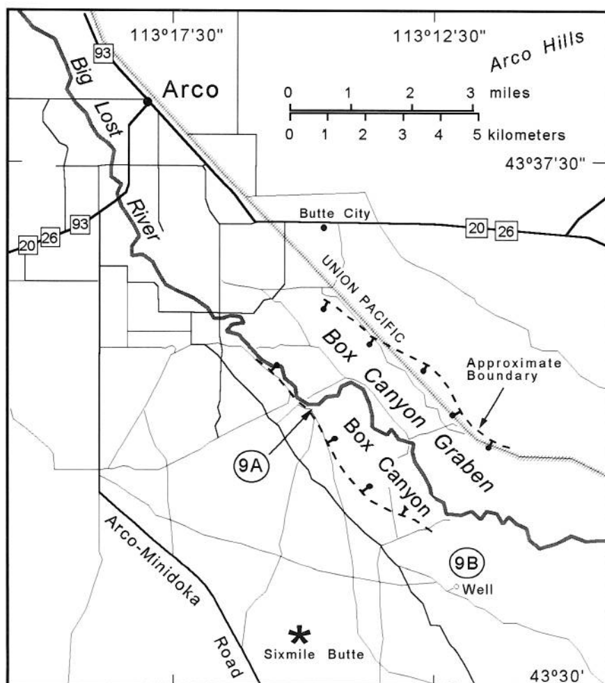
Figure 21. Map of unimproved roads (thin solid lines) south of Arco, Idaho illustrating access to Box Canyon graben. The Big Lost River flows southeast in a direction structurally controlled by the Arco volcanic rift zone (see Fig. 10). Stop 9A allows observation of Box Canyon graben, which follows the same structural trend. Geomorphic features related to catastrophic glacial flooding are observed at Stop 9B.
