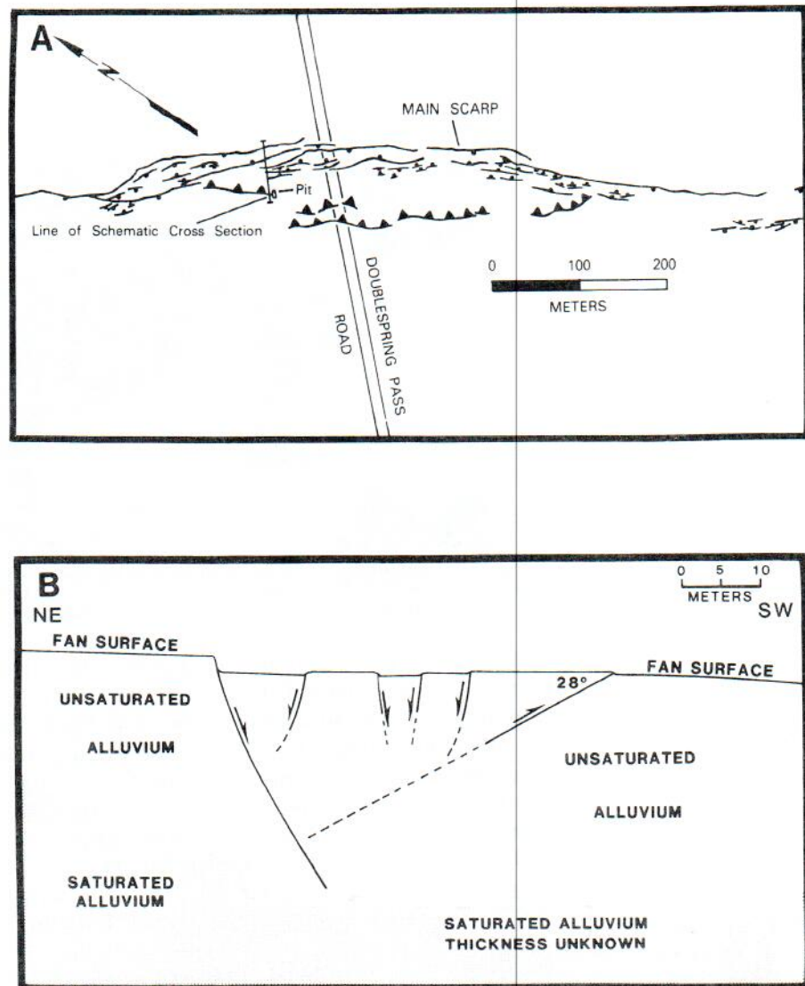
FIG. 10. Detailed map of fault scarps (A) and schematic diagram (B) of thrust faults near Double-spring Pass Road (see Plate 1). (A) Normal faults have ball on downthrown side; thrust faults have barbs on upper plate. Thrust fault exposed in pit dips 28° to the northeast. Note arcuate form of main scarp. (B) Schematic diagram showing geologic relations associated with the thrust faults. Maximum height of thrust faults is about 15 cm. Depth to top of saturated alluvium from Pelton et al. (1985).
