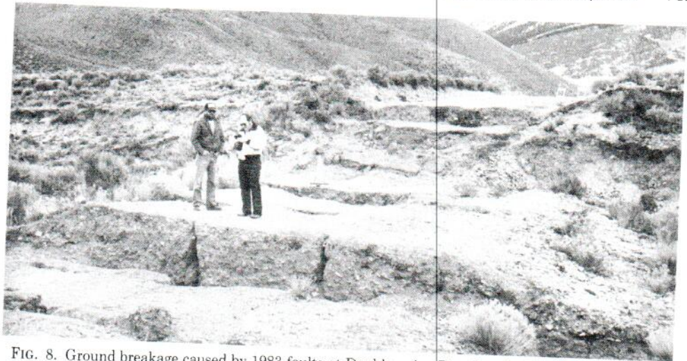
FIG. 8. Ground breakage caused by 1983 faults at Doublespring Pass Road. Zone of faults is 20 to 30 m wide with ground surface broken into numerous blocks. View is to the northeast. Photograph by M. N. Machette (U.S. Geological Survey Archive No. 40), 9 November 1983.
