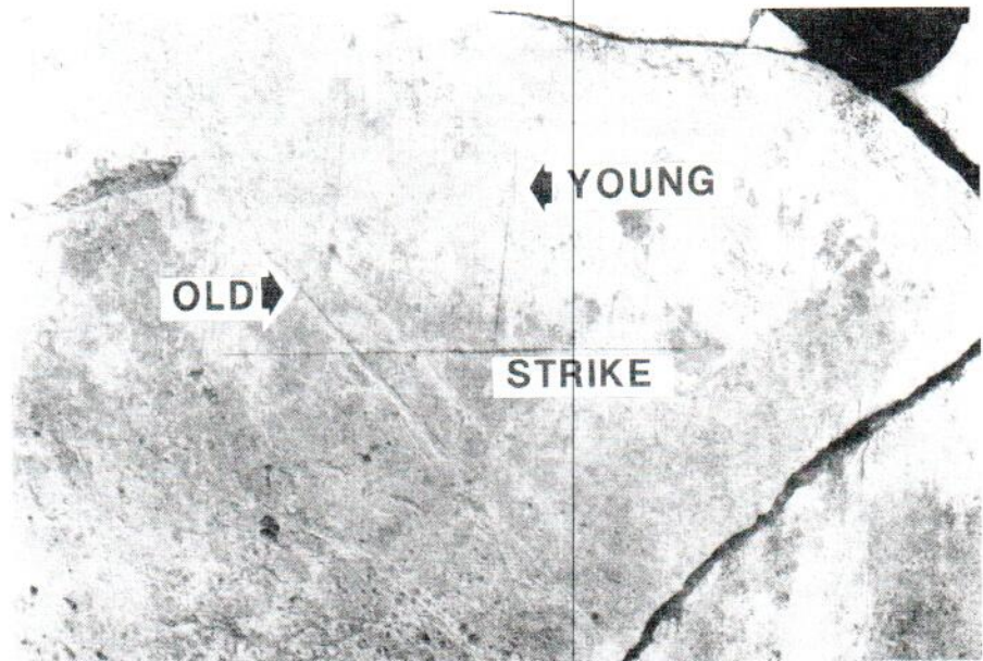
FIG. 15. Shale bedrock exposed in footwall of the 1983 scarp on northwest flank of Dickey Peak showing two sets of pre-1983 striae (see L on Plate 2). Fault plane strikes N12°W and dips 53°W. Older set of striae shows more sinistral slip than dip slip; younger set shows mostly dip slip with minor dextral slip. Camera lens cover in upper right is 5.5 cm in diameter. Photograph by A. J. Crone, 27 August 1984.
