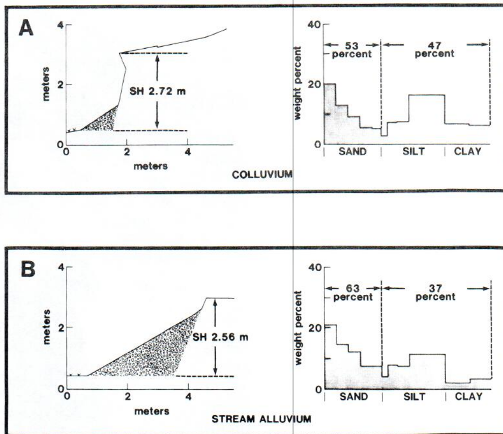
FIG. 18. Slope profile and particle-size distribution of matrix ( <2 mm) from scarp formed on colluvium (A) and stream alluvium (B) near Rock Creek (Figure 17). Colluvium and stream alluvium both contain about 85 per cent gravel and 15 per cent matrix, but matrix of the colluvium contains 10 per cent more silt and clay. SH is scarp height in meters.
