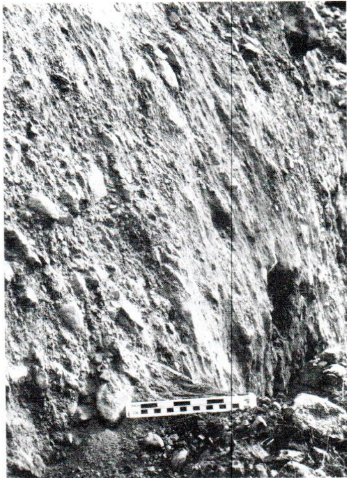
FIG. 5. Corrugations and grooves near the base of the large scarp shown in Figure 3. Grooves were formed by clasts dragged along the fault plane. Bars on scale show inches (above) and centimeters (below). Photograph by A. J. Crone, 3 November 1983.
