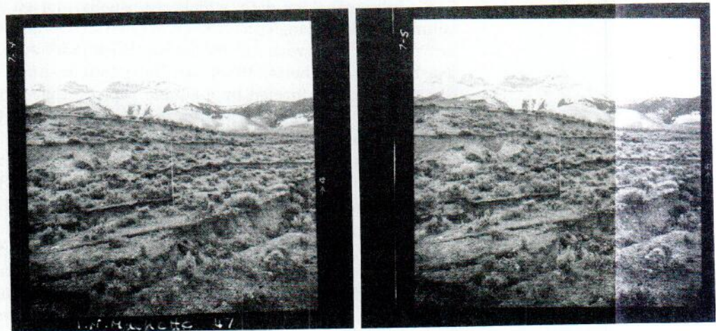
FIG. 16. Stereo pair of stair-step fault scarps about 300 m north of Doublespring Pass road (see Plate 1). View is to the southeast. Stadia rod is 2.5 m long. Photographs by M. N. Machette (U.S. Geological Survey Archive No. 47), 8 November 1983.
