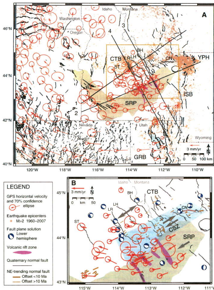
Figure 1. Maps show horizontal GPS velocities in North American reference frame, Quaternary faults, distribution of seismicity, and fault-plane solutions. Abbreviations: CTB—Centennial tectonic belt, CSZ—Centennial shear zone, GRB—Great Basin, ISB—Intermountain seismic belt, SRP—Snake River Plain, and YPH—Yellowstone hotspot. Normal faults: CN—Centennial, BH—Beaverhead, LH—Lemhi, LR—Lost River, and ST—Sawtooth. (A) Cross-section locations are shown for profiles in Figure 2. Brown box shows location of map shown in B. (B) Global positioning system (GPS) velocities indicate that the Centennial tectonic belt extends (double-ended black arrow) at a higher rate than in the Snake River Plain (black arrow), which is an order of magnitude lower (see Figs. 2A and 2B). Right-lateral shear of 0.9 \pm 0.3 – 1.7 \pm 0.2 mm/yr (opposing black arrows) in the Centennial shear zone (blue shaded region labeled CSZ) is required to accommodate the different strain rates. Quaternary faults: U.S. Geological Survey (2007); NE-trending normal faults: modified from Zentner (1989); seismicity: Advanced National Seismic System (2007); and focal mechanisms: Zollweg and Richins (1985), Richins et al. (1987), Doser and Smith (1989), Jackson et al. (1993), Stickney (1997), and Saint Louis University (2007).
