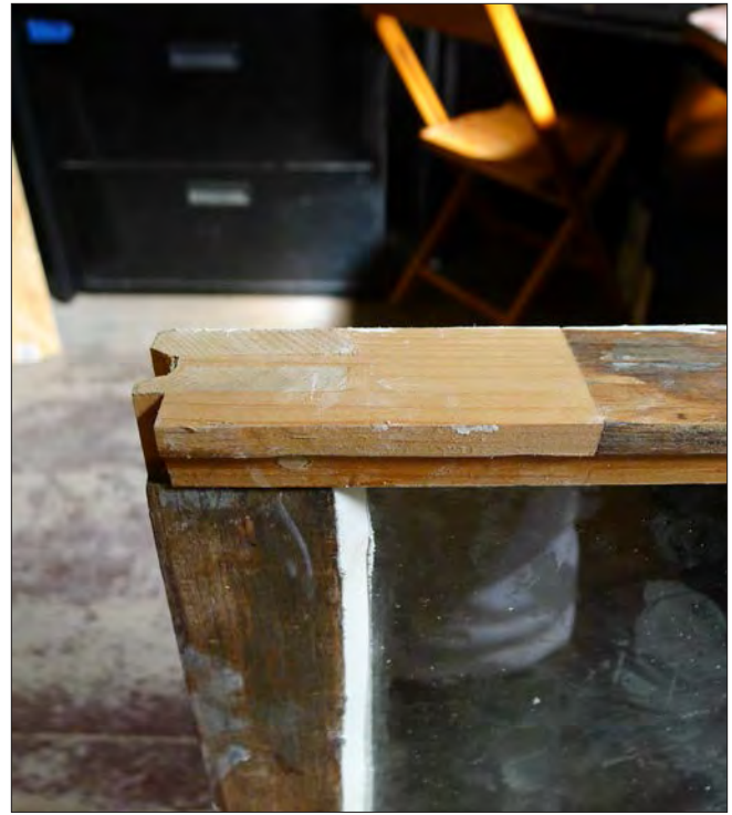
One of the advantages of historic wood windows over modern prefabricated units is repairability. This photo demonstrates a dutchman repair at the corner of a historic wood window. Also note the new glazing putty.
