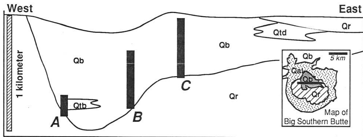
Figure 11. Schematic cross section of the uplifted slab of mafic-to-intermediate volcanic rocks exposed on the north flank of Big Southern Butte (data from Fishel, 1992). Locations of measured stratigraphic sections used in the compilation are shown as A, B, C; units dip about 45 degrees north. All deposits are of Quaternary age: Qal = alluvial-fan deposits; Qr = rhyolite of Big Southern Butte; Qb = Snake River Plain basalt lava flows; Qtb = lower trachybasalts; Qtd = upper trachydacites. See Fig. 12 for composition and nomenclature of selected rock units.
