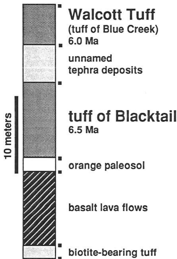
Figure 15. Simplified, composite-stratigraphic section of volcanic rocks exposed at Howe Point, Stop 7 (adapted from Hackett and Morgan, 1988).
