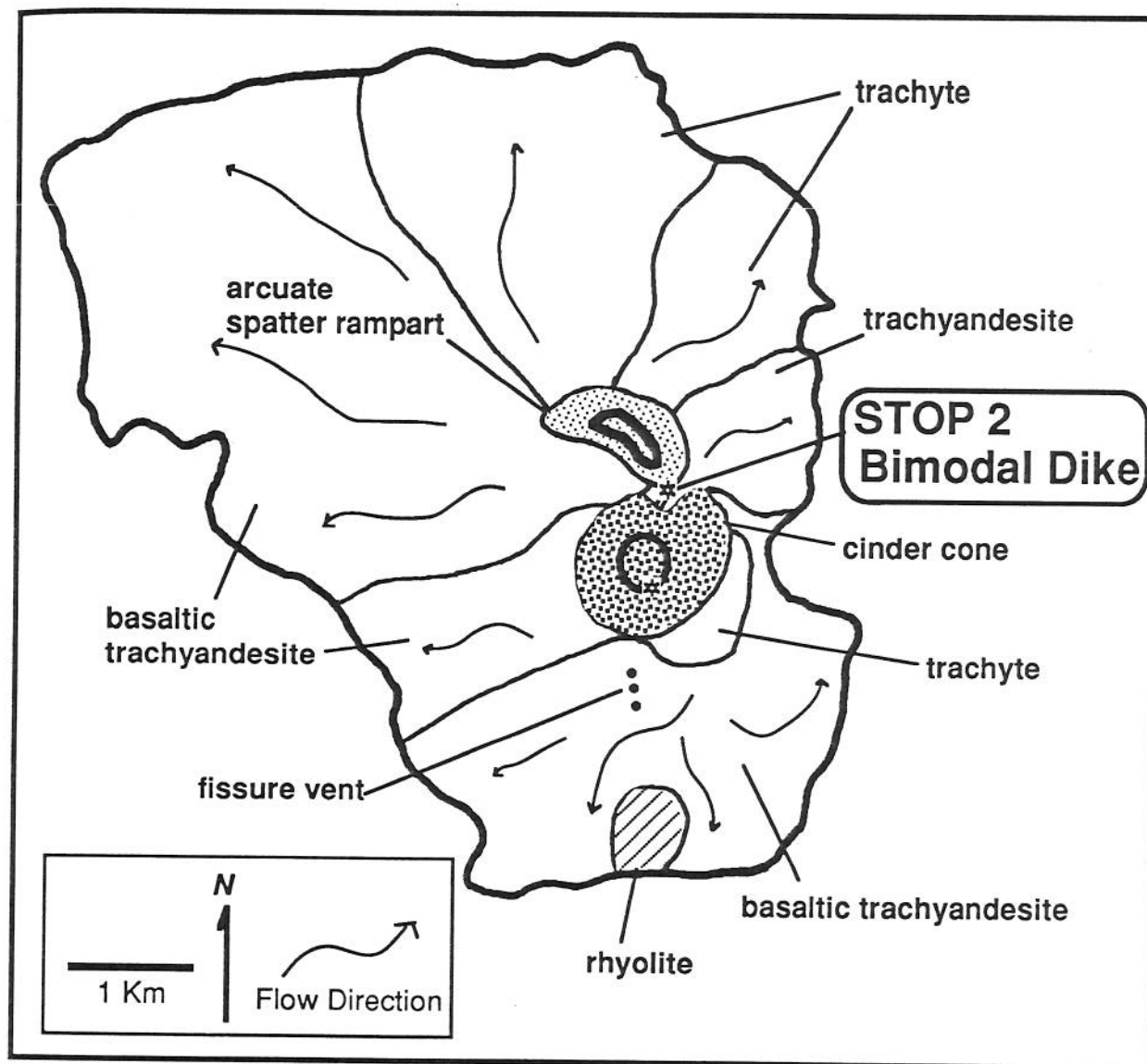
Figure 10. Generalized geologic map of the Cedar Butte eruptive center (data from Hayden, 1992), showing major map units, vent areas and position of Stop 2. All rock units are Quaternary in age, and the nomenclature of rock units is based on the geochemical data of Figure 12.
