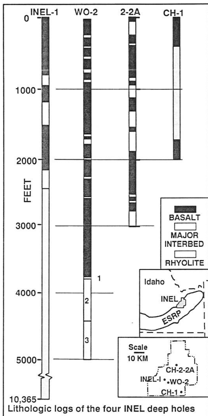
Figure 3. Simplified lithologic logs from deep drillholes in the INEL area. Only INEL-1 and WO-2 intersect Tertiary rhyolite, beneath basalts and sediments of the Snake River Group. Lithologic data are from Doherty and others (1979) for INEL-1; Doherty (1979a) for hole CH-1; and Doherty (1979b) for corehole 2-2A.
