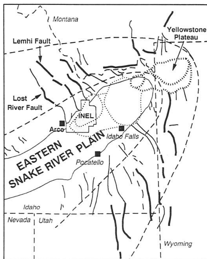
Figure 4. Map showing the generalized locations of Neogene silicic calderas (dotted ellipses) that are inferred to be buried beneath the ESRP (Morgan and others, 1984; Morgan, 1988), the exposed Quaternary calderas of the Yellowstone Plateau volcanic field (Christiansen, 1984), the parabolic region of historical seismicity centered on the Yellowstone plateau (enclosed by dashed curves; Anders and others, 1989), and major normal faults around the ESRP (bold lines indicate fault segments with Holocene displacement).
