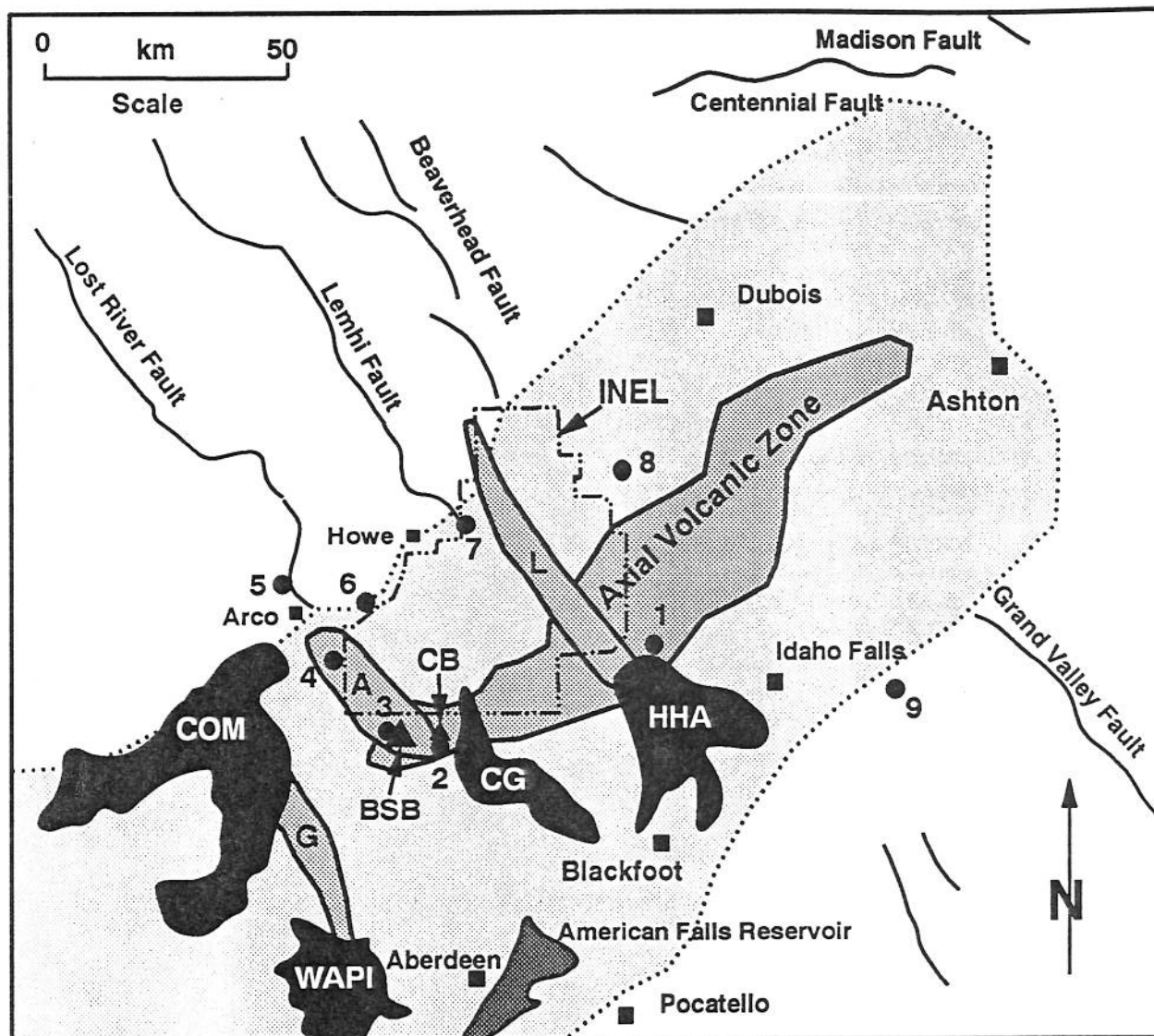
Figure 6. Map showing the major volcanic and tectonic elements of the INEL area, including northwest-trending normal faults of the Basin and Range tectonic province, northwest-trending volcanic rift zones on the ESRP, and the northeast-trending axial volcanic zone (a central, constructional region of volcanic vents). Holocene lava fields near the INEL are Hell's Half-Acre (HHA), Cerro Grande (CG), Wapi, and Craters of the Moon (COM). Locations of stops 1-9 are indicated.
