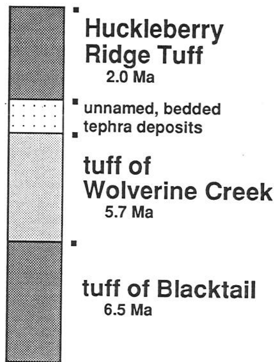
Figure 16. Generalized stratigraphy of Quaternary and Neogene rhyolitic tuffs exposed at the Blacktail Recreation area along the southern margin of the ESRP, Stop 9 (data from Morgan, 1988; Hackett and Morgan, 1988). The total section is about 300 m thick; relative thickness of the tuffs is not drawn to scale.
