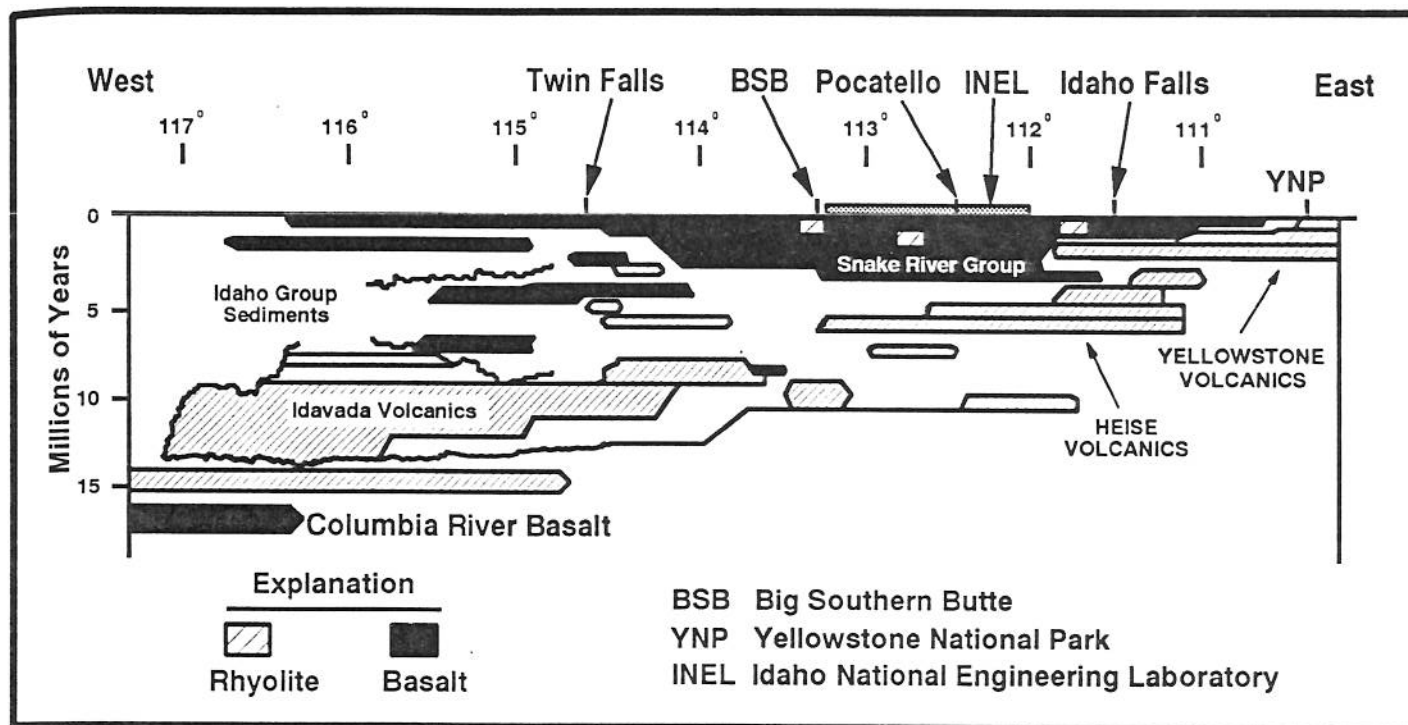
Figure 2. Age-distance plot of late Cenozoic, bimodal volcanism in the Snake River Plain-Yellowstone province (adapted from Armstrong and others, 1975; Hackett and Morgan, 1988; Rodgers and others, 1990). Two features are emphasized: the onset of voluminous rhyolitic volcanism becomes progressively younger toward the northeast, and the Tertiary eruptive complexes have been subsequently covered by Quaternary basalts and sediments of the Snake River Group.
