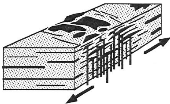
Figure 8. Schematic block diagrams showing the different modes of extension in the INEL region. On the Eastern Snake River Plain, the lithosphere apparently extends by mafic-dike intrusion. In the surrounding Basin and Range province, the lithosphere extends by normal faulting.
