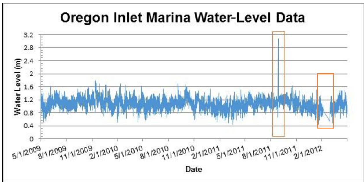
Figure 6. Plot of water level data from Oregon Inlet Marina, NC (Station ID 8652587) from the time the imagery was taken (May 2009) to the time ground truthing was performed (April 2012). The red boxes represent two events in the water level data, which includes Hurricane Irene (28 August 2011) and a winter storm (5–28 February 2012).
