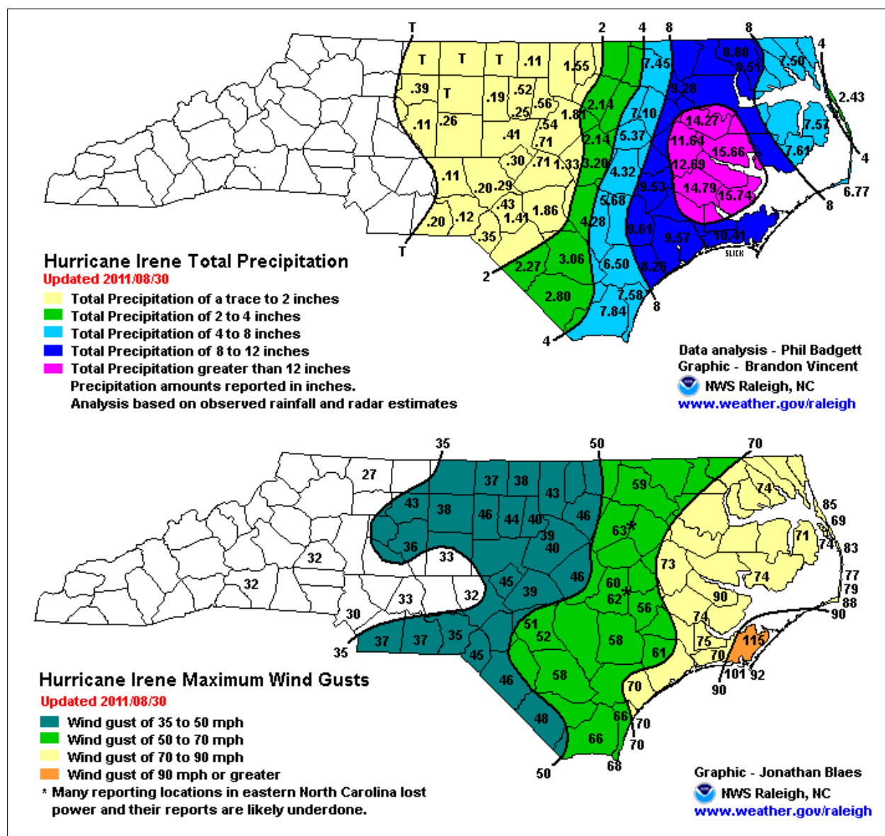
Figure 7. Total precipitation and maximum wind gusts during Hurricane Irene (NWS Raleigh, NC 2014).
