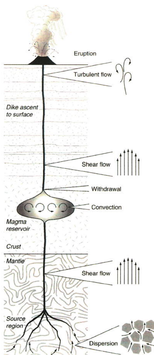
Fig. 7. Diagram illustrating fluid dynamic processes that might affect original source-related compositional variations in the melt, at different steps in the ascent of basaltic magmas.
