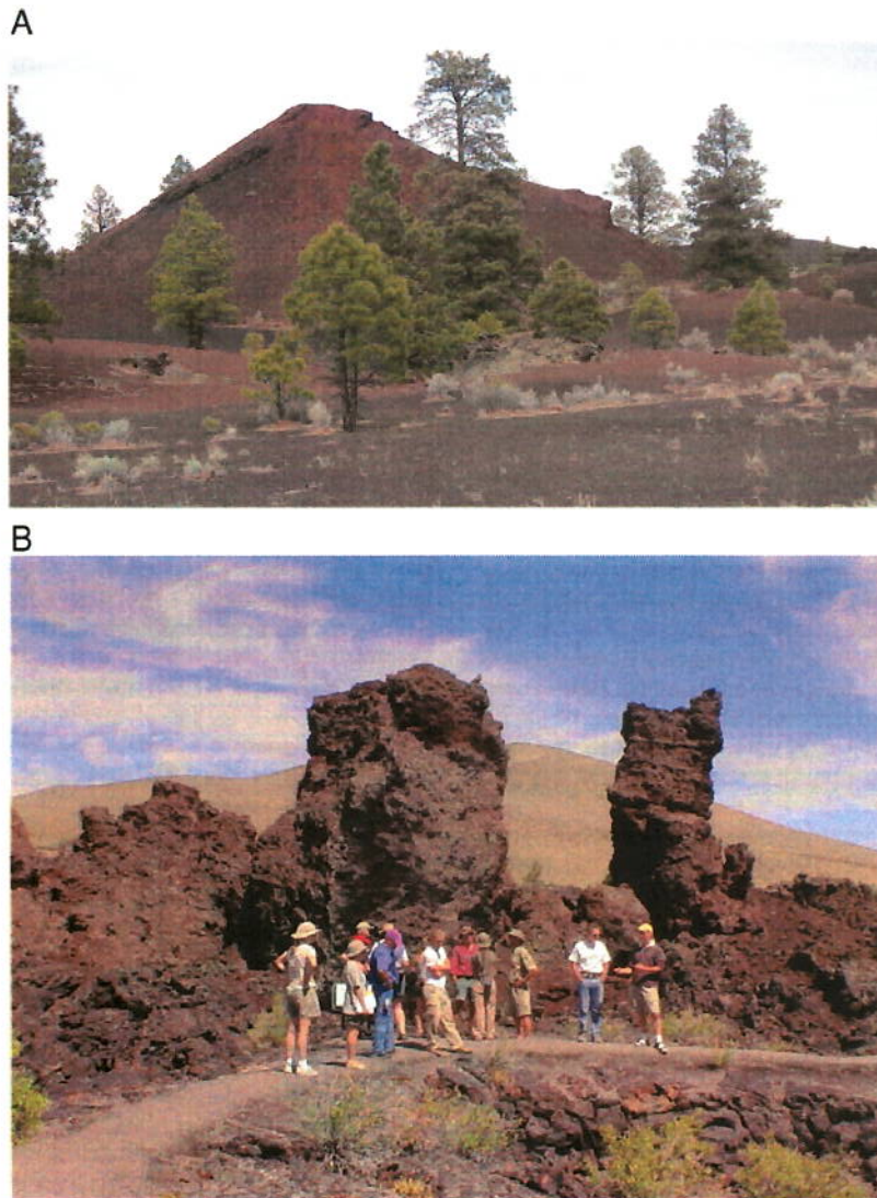
Fig. 4. (A) Raft of cone material on top of the Bonito flow at the ~ 1 ka Sunset Crater volcano (Arizona, USA), an example of the type of raft illustrated in Fig. 3A. Original bedding of variably welded cone deposits dip to the left and are locally visible through the scree that has formed due to raft degradation (see Valentine et al., 2006) as well as fallout scoria that blanketed the lava flow and raft surfaces. Raft is ~ 15 m high. (B) Rafted cone material at Craters of the Moon National Monument (Idaho, USA), illustrating the breaking up of cone agglutinate into blocks as the raft was carried atop a lava flow. This raft corresponds to the type illustrated in Fig. 3B.
