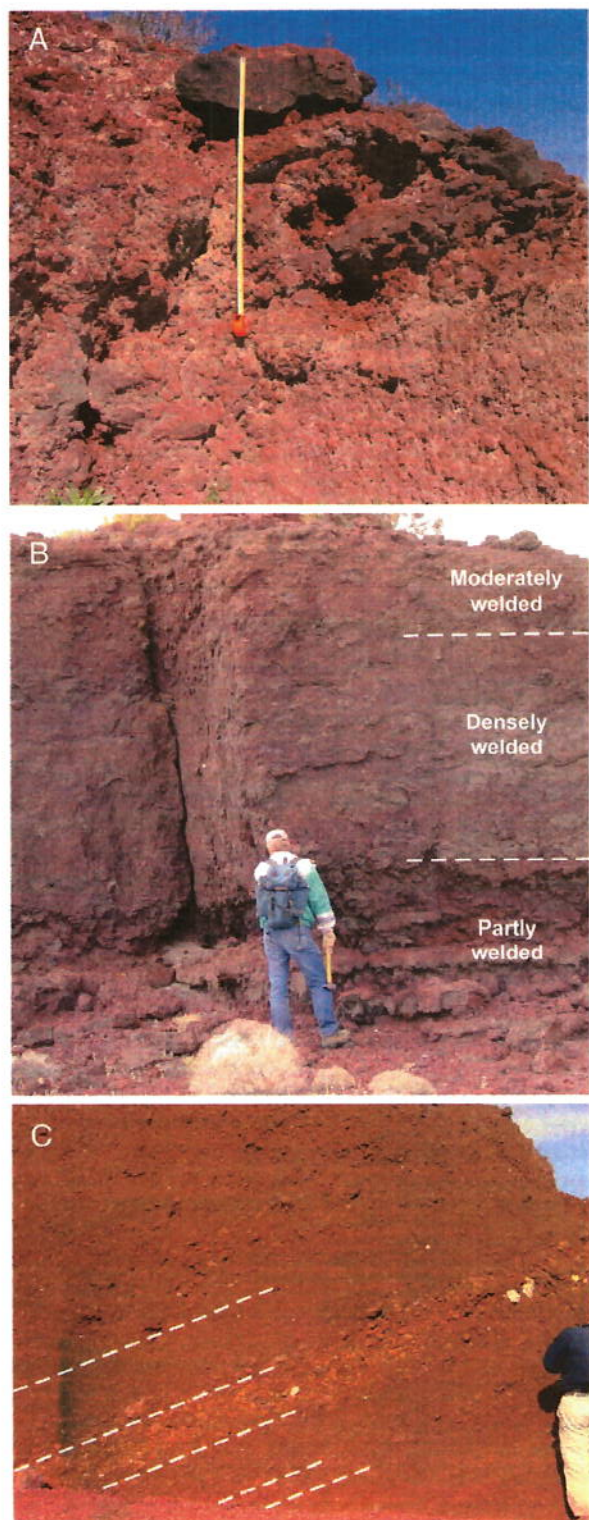
Fig. 1. Examples of proximal pyroclastic facies from three types of explosive basaltic eruption styles (all three examples are within ~100 m of vent). (A) Proximal Strombolian facies exposed at Black Cone, Nevada (~1 Ma; Valentine et al., 2006). Note abundance of coarse lapilli, which commonly occur in lenticular beds produced by grain avalanching. Local accumulations of coarser bombs (ranging from fluidal, flattened shapes to spheroidal) also define crude bedding. Measuring tape is 1 m long. Deposits are slightly welded, and dip toward the vent. (B) Proximal Hawaiian facies. These deposits are from an early phase of a Miocene-age fissure eruption at East Basalt Ridge, Nevada (Keating et al., 2008), deposited on flat ground about 50 m from the vent. Note partly welded basal deposits consisting of coarse lapilli and flattened bombs, grading upward into densely welded deposits (above person). Proximal (cone) facies of Hawaiian eruptions often have vertically alternating zones of moderate and dense welding, reflecting pulses in eruptive fountains. Person is ~1.8 m tall. (C) Proximal facies produced by violent Strombolian activity. Deposits consist almost entirely of medium to coarse lapilli and some blocks, in massive, planar-parallel beds (dipping toward vent, indicated by dashed lines) that are characteristic of deposition by fallout rather than avalanching (lighter colored, lithic-enriched bed is a good example of the bedding style). Deposits are non-welded, and fluidal or flattened bombs are rare. Person is ~1.8 m tall.
