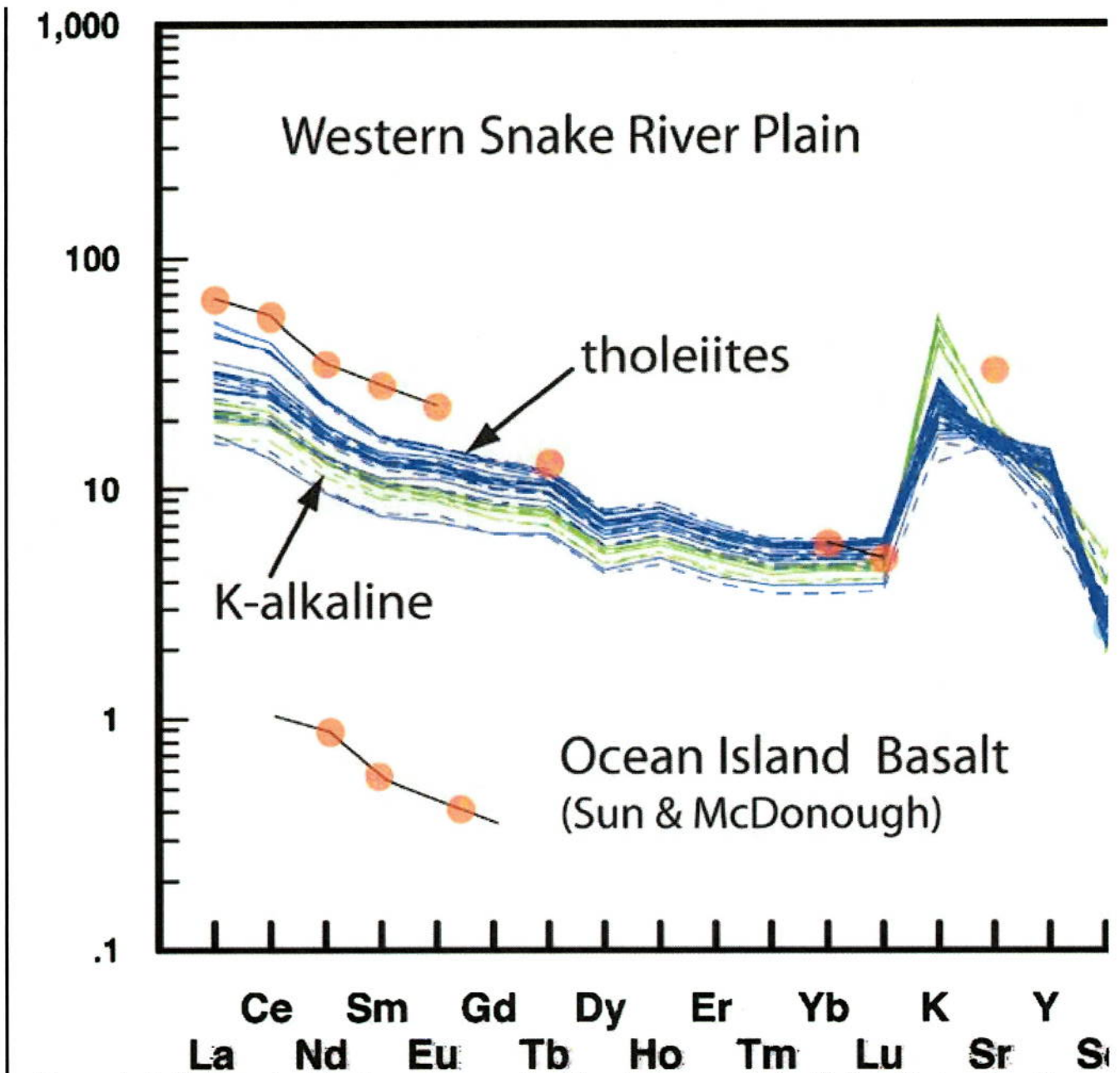
Figure 4: Multi-element spider diagrams normalized to primitive mantle for (A) tholeiitic basalts of the ce. basalts and high-K transitional alkaline basalts of western SRP, normalized to primitive mantle of Taylor and al (1992), White et al (2002), Shervais et al (2002, 2006), and Hughes et al (2002).
