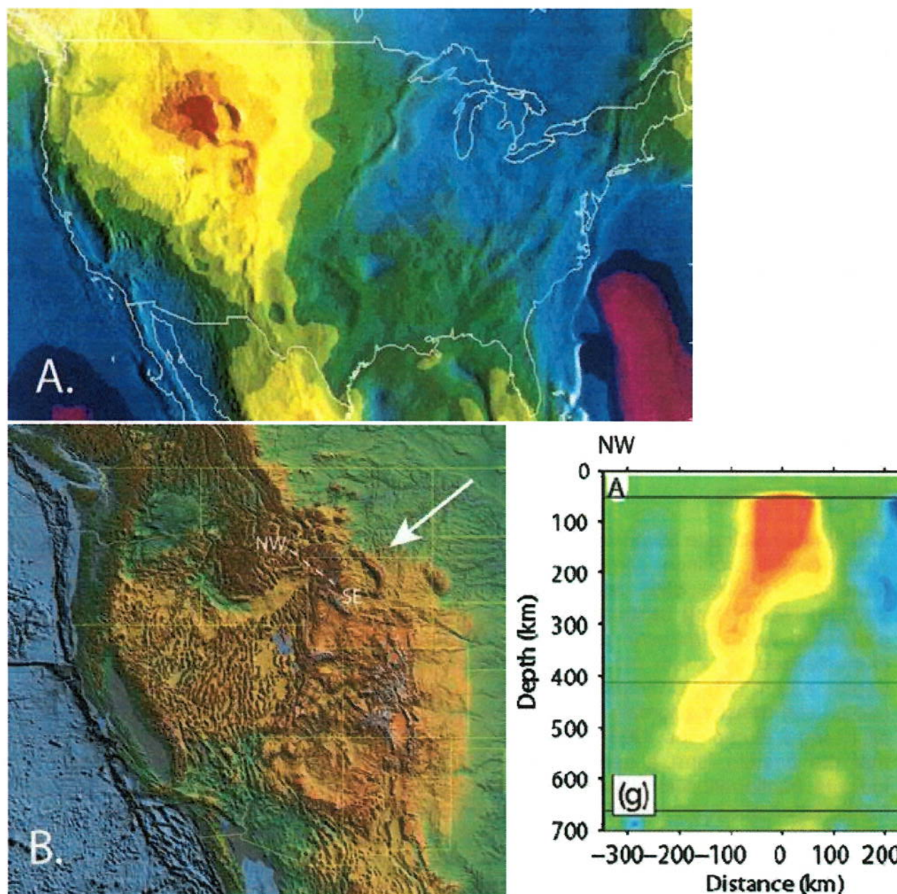
Figure 1: Impact of the Snake River-Yellowstone plume on North America. (A) Geoid map of North America showing a geoid anomaly of +15 m centered on current location of Snake River-Yellowstone hotspot. (B) digital topographic map of the Snake River-Yellowstone region showing the plume tail on topography, cutting across the regional Basin & Range trend to form a broad depression several hundred km long. White arrow shows direction of North American plate motion, dashed white line shows seismic tomograph section in figure 1C. (C) Seismic tomograph of Yellowstone thermal anomaly; anomaly (plane of section). Note the high velocity (cold) lithospheric root of Wyoming craton, which extends to at least 600 km depth. Tomograph from Yuan and Dueker, 2005.
