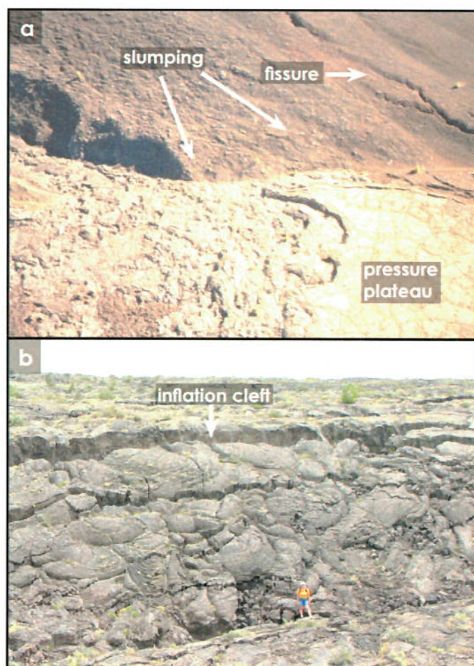
Figure 17: a) Pressure Plateau on the south side of Broken Top. Also note slumping and open fissures on side of cone. b) Side view of a pressure plateau
