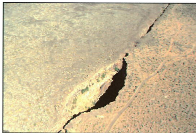
Figure 3: View of Kings Bowl and the Great Rift.
