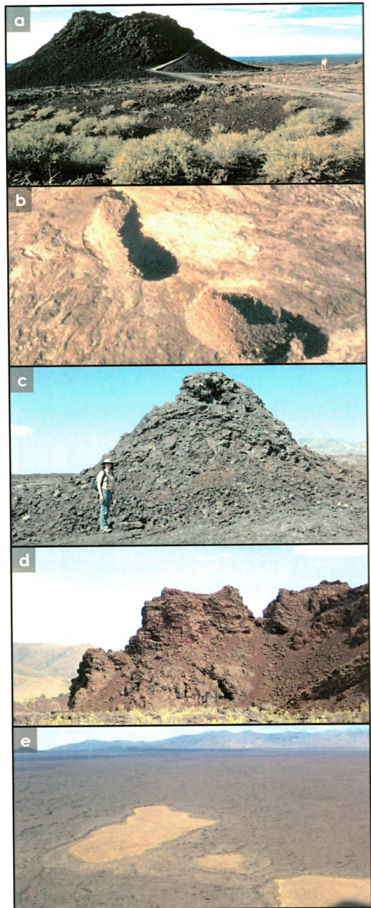
Figure 19: a) Spatter cone b) Pit craters c) Hornito d) Rafted blocks at Devil's Orchard e) Kipukas—older areas that are often higher and much more vegetated than the surrounding darker young lava
