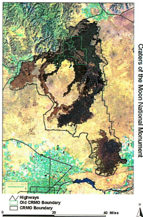
Figure 2: Craters of the Moon (CRMO). The park almost spans the width of the eastern Snake River Plain.
