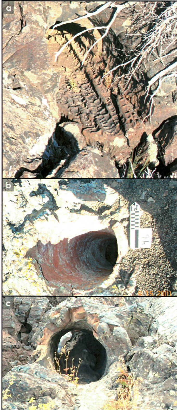
Figure 24: a) Tree mold of charred wood b) Vertical tree mold c) Horizontal tree mold
