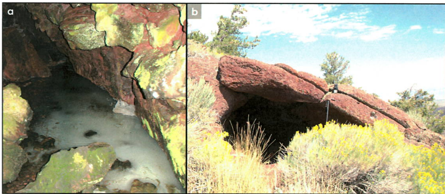
Figure 20: a) Bearsden Waterhole b) Differential watering cave
