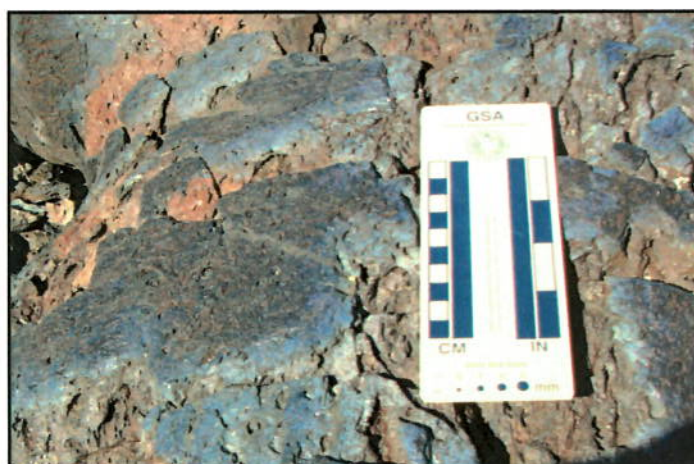
Figure 23: Blue Dragon lava flow
