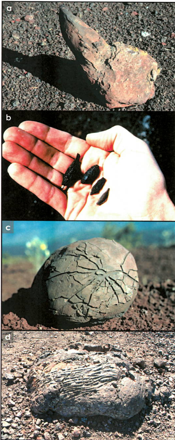
Figure 10: Volcanic bombs found at Craters of the Moon. a) Spindle bomb b) Ribbon bomb c) Breadcrust Bomb and d) Cow pie bomb
