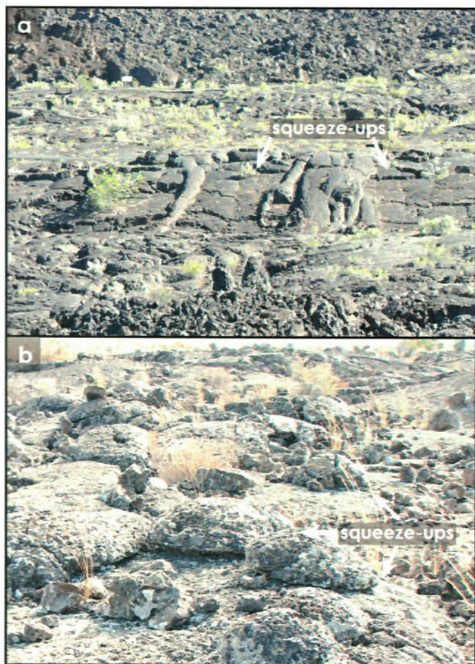
Figure 16: a) Squeeze-up that came from the tension fracture in the top of a flow/pressure ridge b) Squeeze-ups that look like mushrooms or candy kisses that oozed up through a crack in the crust of a lava pond
