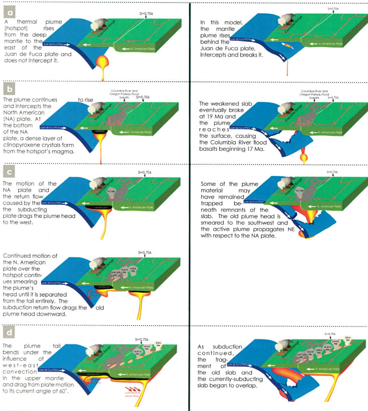
Figure 6: Sketch showing differing interpretations ( left: modified from: Smith, et al, 2009; right: modified from: Obrebski, et al, 2010) of the interaction between the mantle plume and the Juan de Fuca plate. a) The mantle plume rises from below b) The plume reaches the surface, triggering the Columbia River flood basalts beginning 17 Ma. c) The formation of extensive magma chambers and crustal melting leads to rhyolitic caldera-forming volcanism. Caldera volcanism continues as the N. American plate continues to move over the hotspot. d) The N. American plate continues moving over the plume to its current position below Yellowstone National Park.
