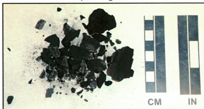
Figure 21: Charcoal from COM tree mold
