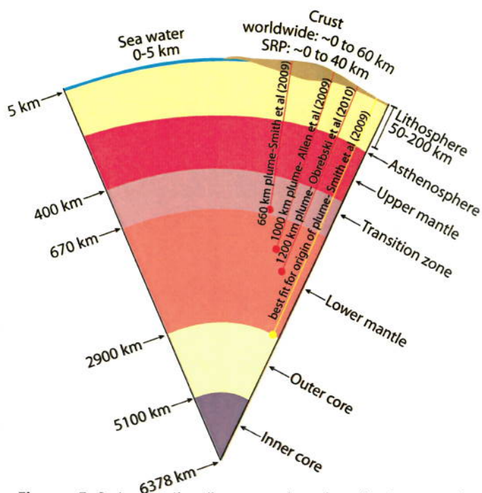
Figure 5: Schematic diagram showing the layers of the earth and the depths to which the mantle plume has been imaged by various authors. Not to scale. Adapted from AGI Datasheets 4 th edition.
