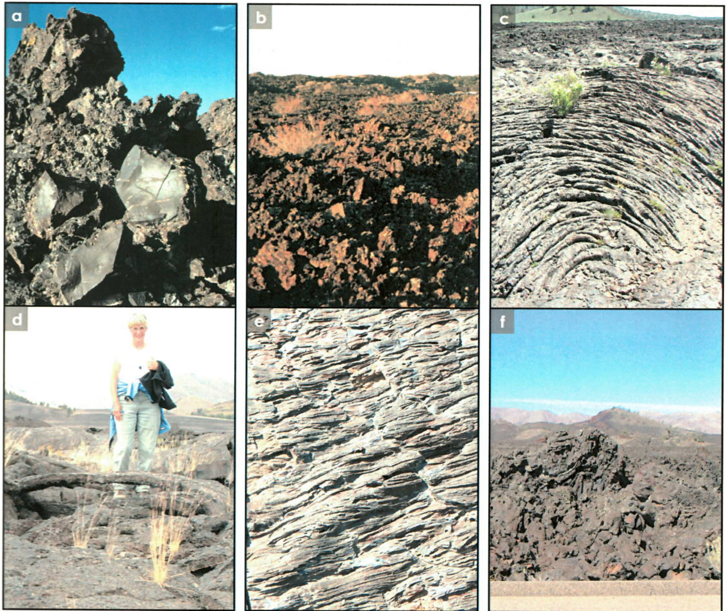
Figure 12: Types of lava flows at Craters of the Moon a) Block lava b) 'A'ā c) Pahoehoe d) Shelly pahoehoe e) Spiny pahoehoe f) Slabby pahoehoe
