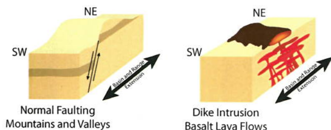
Figure 8: Sketch showing the crustal response to tensional forces in the a) Basin and Range and b) Snake River Plain.
