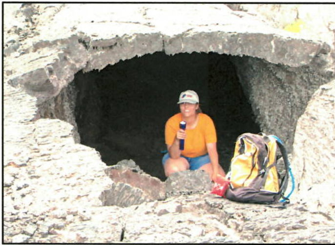
Figure 13: Small lava tube in Broken Top flow
