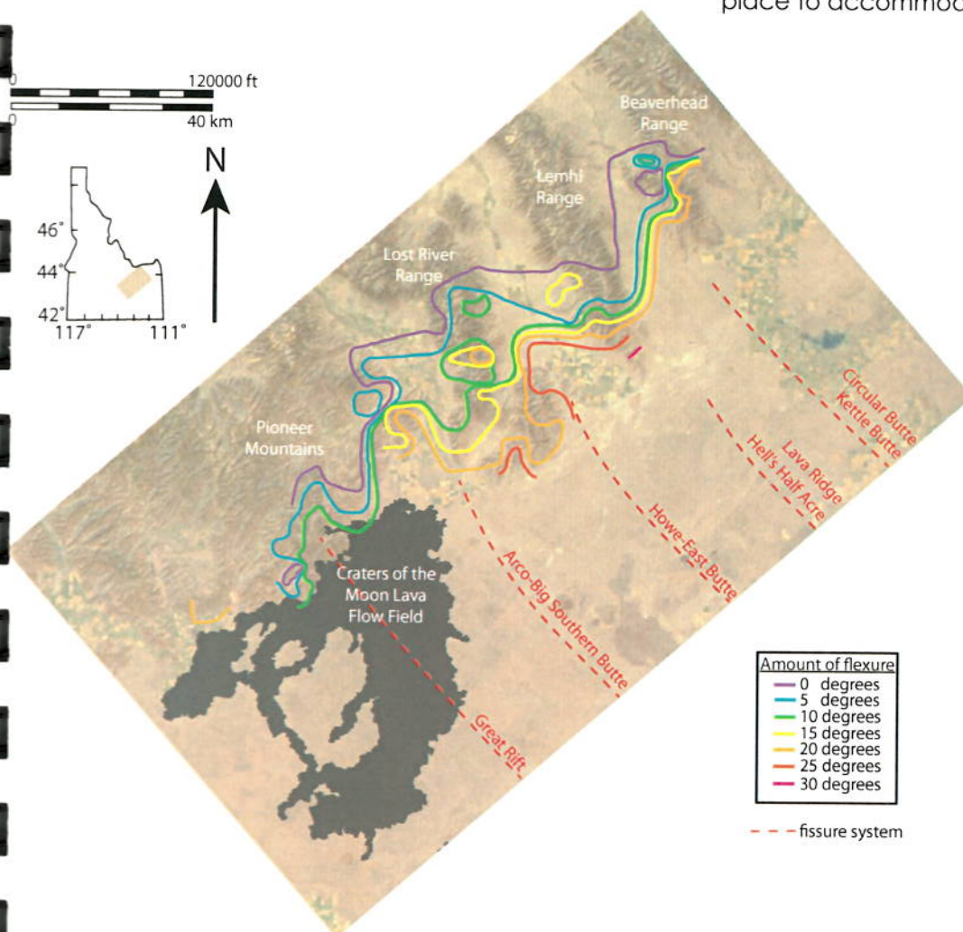
Figure 4: Amount of crustal flexure at the northwestern edge of the Snake River Plain in the CRMO vicinity. Adapted from Rodgers, et al (2002).
