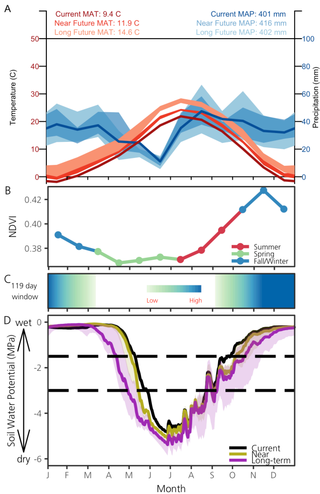
Figure 3. Panel A. Average seasonal patterns of climate in the shallow loamy mesa-top pinyon-juniper woodlands ecosystem in Mesa Verde NP. Climate diagram (Walter and Leith 1967) shows mean monthly temperature (°C) and precipitation (mm) in dark red and blue lines, respectively, in the current period (1970–2010). Shaded red and blue areas indicate the range of potential values in the near (darker area; 2020–2059) and long-term (lighter area; 2060–2099) future periods. Mean annual temperature (MAT) and mean annual precipitation (MAP) are derived from the mean monthly values. Panel B. Monthly mean for normalized difference vegetation index (NDVI, 2001–2014). Panel C. Seasonal periods when soil moisture is related to fluctuations in vegetation productivity, depicted by correlations between NDVI and soil water potential (SWP) 2001–2014. Colors indicate the sum of significant correlations ( p < 0.1 ) that overlap with each day of the year based upon window length (119 days identified as the most significant interval length). Darker blue indicates periods of greater cumulative correlation between NDVI and SWP. Panel D. Average daily SWP for the current period (1970–2010; black), near future (2020–2059; yellow), and long-term future (2060–2099; purple). For future time periods, thick lines represent the median value among climate models, while shaded areas represent the range of values across different climate models.
