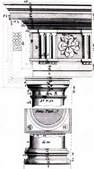
Doric Entablature with 6 Base & Capital
