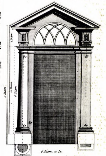
Doric Frontispiece Page 59
