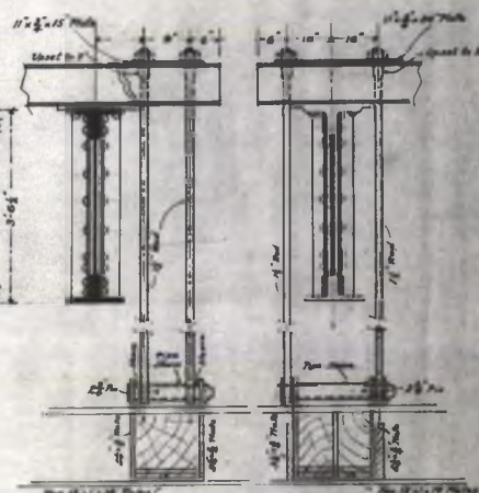
GIRDER "B" GIRDER "C" SECTIONS SHOWING SUSPENSION RODS IN RELATION TO GIRDER
