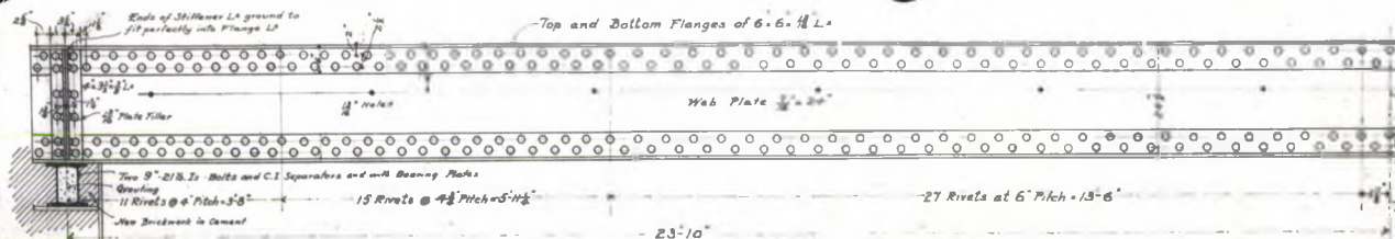
HALF ELEVATION OF GIRDER "A" SUPPORTING FLOOR OF SENATE CHAMBER
