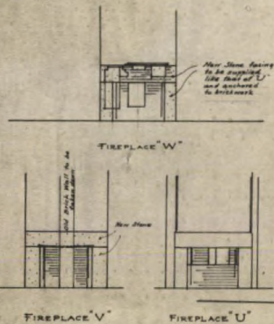
ELEVATIONS OF FIRST STOREY FIREPLACES
