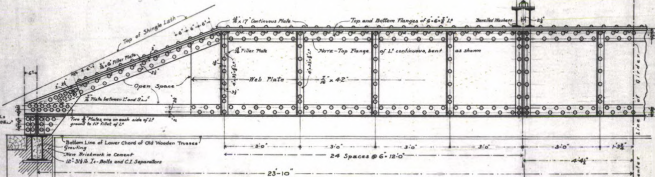
HALF ELEVATION OF PLATE GIRDER "B"
