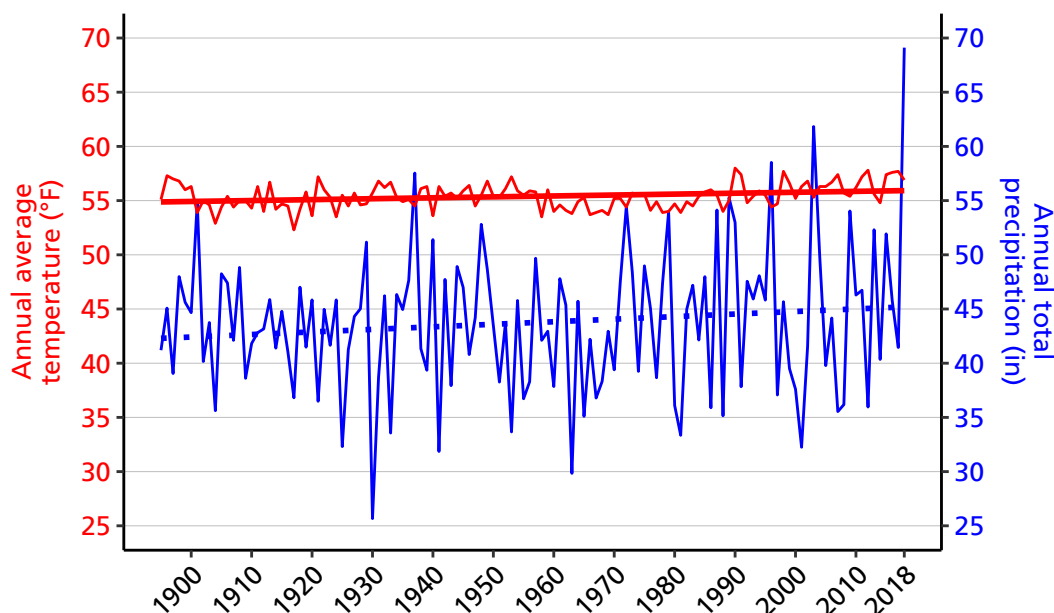
Figure 3. Annual average temperature ( ^{\circ}\text{F} ) and annual total precipitation (in.) for Franklin County, VA from 1895–2018. Solid lines represent statistically significant trends ( p < 0.05 ). Data are available at https://www.ncdc.noaa.gov/cag/county/time-series .
