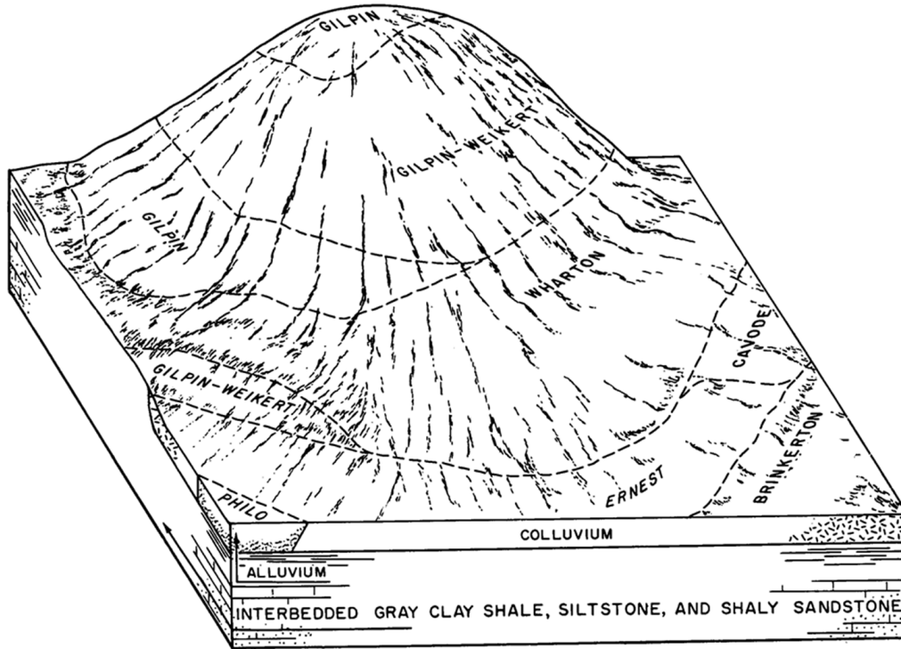
Figure 8.—Landscape positions of some of the major soils in Fort Necessity National Battlefield.
