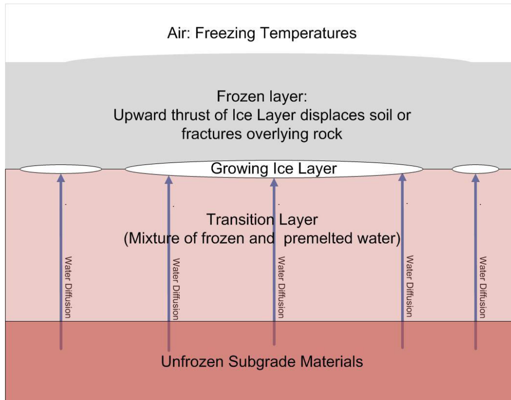
Figure 5.—Diagram illustrating ice lens formation in soils that results in frost heave or frost action. Image is from Williamborg ( http://en.wikipedia.org/wiki/File:Freezing_air_ice_lens_formation.jpg ).
