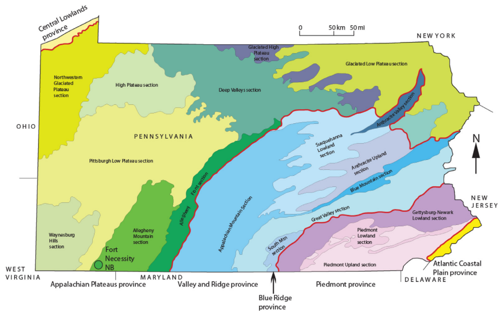
Figure 1.—Physiographic setting of Fort Necessity National Battlefield. The green circle marks the location of the park and historic site. Red lines indicate boundaries between major physiographic provinces. The black arrow locates the northern terminus of the Blue Ridge province. Graphic is by Trista L. Thornberry-Ehrlich, Colorado State University (2009) after Sevon (2000).
