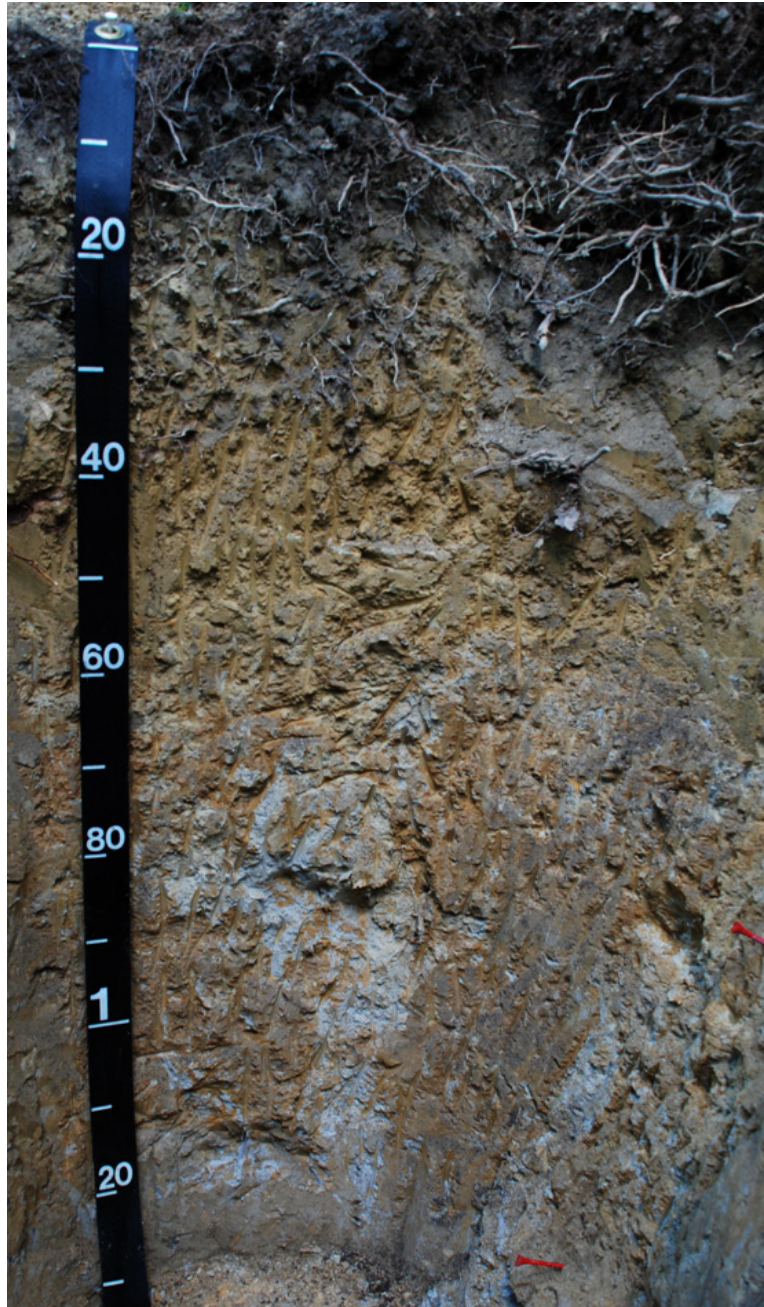
Figure 4.—Profile of a Buchanan soil. Restricted water movement is evidenced by grey colors below a depth of 60 centimeters. Scale is in centimeters. (Image is from the soil survey of New River Gorge National River.)
