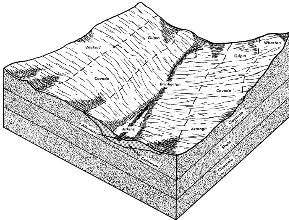
Figure 3.—Relative landscape positions of the soils near Washington's log fort. The fort was located in a small area of Atkins soils, included in the mapping of the Great Meadows. Diagram is not to scale.
