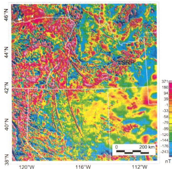
Figure 2. Aeromagnetic map of northern Great Basin with magnetic lineations (black lines) discussed in text. SRP—Snake River Plain.
