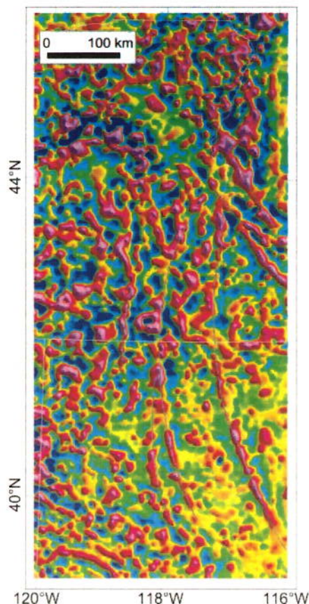
Figure 3. Match-filtered aeromagnetic map highlighting expression of anomalies arising from mid-crustal sources. Magnetic lineations shown in black.
