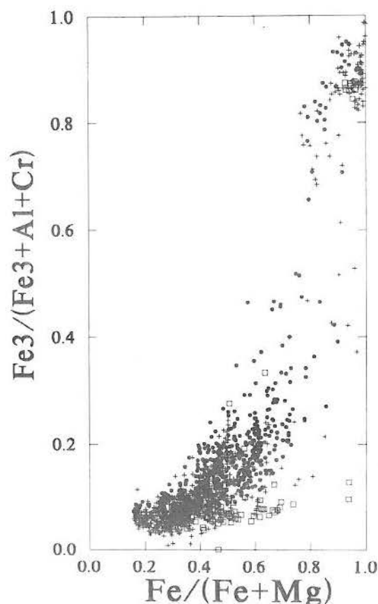
FIG. 6. \text{Fe}^{3+}/(\text{Fe}^{3+} + \text{Al} + \text{Cr}) versus \text{Fe}^{2+}/(\text{Fe}^{2+} + \text{Mg}) plot of spinel samples from boninitic basalts (open squares), ocean-island basalts (solid dots) and mid-ocean-ridge basalts (crosses).
