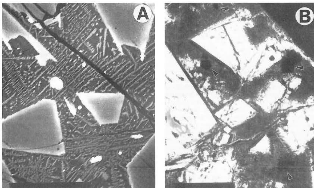
FIG. 17. Type-II porphyritic olivine chondrules in the Semarkona unequilibrated chondrite. A. Back-scattered electron image showing mesostasis texture between olivine phenocrysts in chondrule C11. B. Transmitted-light photomicrograph that shows olivine phenocrysts in a mesostasis containing small crystals of chromite (arrows). Scale bar: 100 \mu\text{m} . The photos are reprinted from Jones (1991) with permission (see Acknowledgements).
