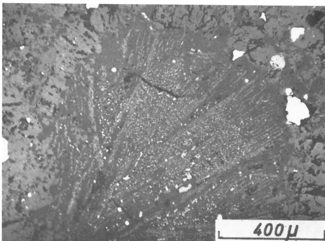
FIG. 18. A metamorphosed chondrule from the Bachmut chondrite. Reflected-light photomicrograph showing radiating crystals of albite with small crystals of chromite between the albite crystals, set in a fine-grained matrix. The photo is reprinted from Ramdohr (1973) with permission (see Acknowledgements).
