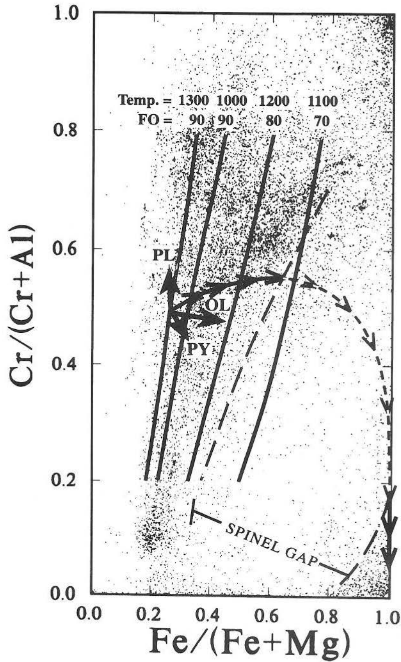
FIG. 4. \text{Cr}/(\text{Cr} + \text{Al}) versus \text{Fe}^{2+}/(\text{Fe}^{2+} + \text{Mg}) plot of all spinel samples in the database. The four sloping lines represent the calculated compositions of spinel that would be in equilibrium with the indicated olivine composition (FO: forsterite) at the indicated temperature (Temp. in ^{\circ}\text{C} ). The calculation was made using the formulation of Sack & Ghiorso (1991) and assumes that the spinel has a \text{Fe}^{3+}/(\text{Fe}^{3+} + \text{Al} + \text{Cr}) value of 0.05. See the text for an explanation of the other lines.
