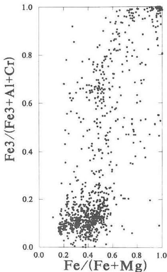
FIG. 14. \text{Fe}^{3+}/(\text{Fe}^{3+} + \text{Al} + \text{Cr}) versus \text{Fe}^{2+}/(\text{Fe}^{2+} + \text{Mg}) plot of spinel samples from kimberlites.
