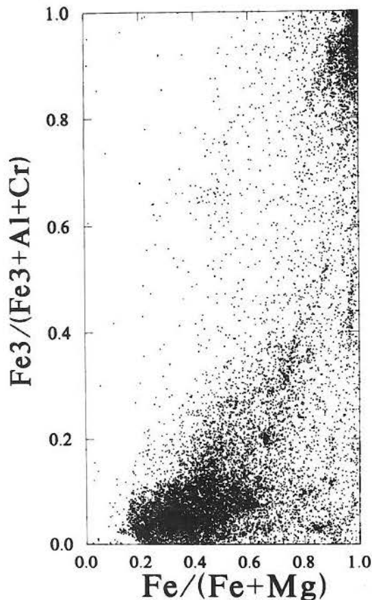
FIG. 3. \text{Fe}^{3+}/(\text{Fe}^{3+} + \text{Al} + \text{Cr}) versus \text{Fe}^{2+}/(\text{Fe}^{2+} + \text{Mg}) plot of 16 093 samples of spinel in the database.
