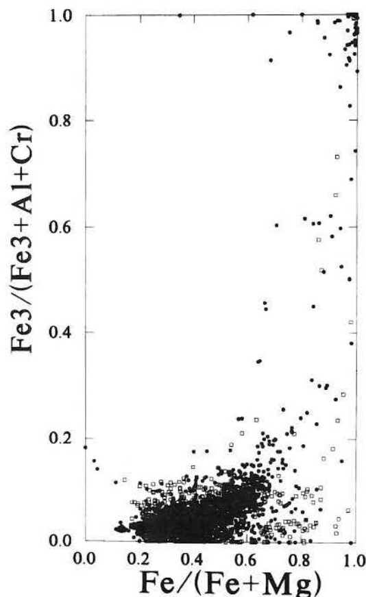
FIG. 10. \text{Fe}^{3+}/(\text{Fe}^{3+} + \text{Al} + \text{Cr}) versus \text{Fe}^{2+}/(\text{Fe}^{2+} + \text{Mg}) plot of spinel samples from ophiolites (solid dots) and chromitites (open squares).
