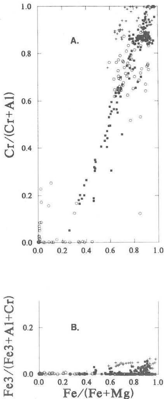
FIG. 19. The composition of spinel in chondritic meteorites. The spinel samples from CAI fragments in unequilibrated carbonaceous chondrites are shown by open circles, the chromite samples from unequilibrated ordinary chondrites are shown by crosses, and the samples of chromite and spinel from equilibrated ordinary chondrites are shown by filled squares. A. \text{Cr}/(\text{Cr} + \text{Al}) versus \text{Fe}^{2+}/(\text{Fe}^{2+} + \text{Mg}) . B. \text{Fe}^{3+}/(\text{Fe}^{3+} + \text{Al} + \text{Cr}) versus \text{Fe}^{2+}/(\text{Fe}^{2+} + \text{Mg}) .
