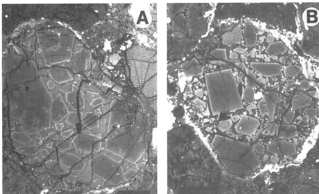
FIG. 16. Type-II porphyritic olivine chondrules in the Semarkona unequilibrated chondrite; back-scattered electron images. A. Chondrule C11, with zoned phenocrysts of olivine set in a mesostasis of glass and fine crystallites. B. Chondrule 51, with zoned phenocrysts of olivine, a small crystal of chromite ("C") and a small crystal of augite ("A") in mesostasis. Scale bar: 200 \mu\text{m} . The photos are reprinted from Jones (1991) with permission (see Acknowledgements).
