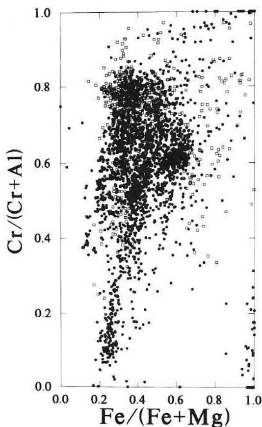
FIG. 9. \text{Cr}/(\text{Cr} + \text{Al}) versus \text{Fe}^{2+}/(\text{Fe}^{2+} + \text{Mg}) plot of spinel samples from ophiolites (solid dots) and chromitites (open squares).
