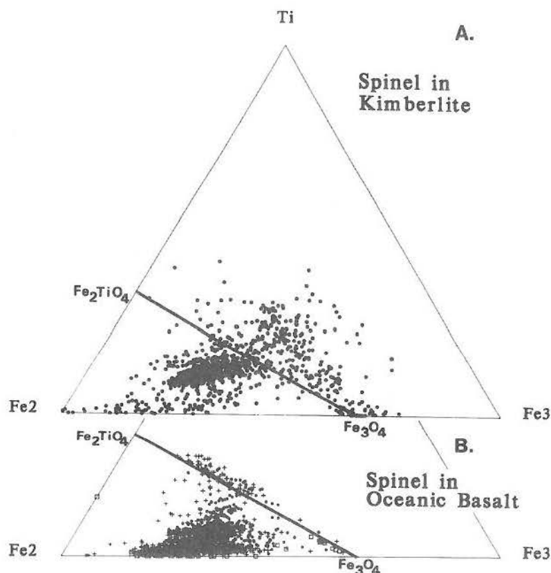
FIG. 15. \text{Fe}^{2+} – \text{Fe}^{3+} – Ti plot of spinel samples from kimberlites (A) and from oceanic basalts (B), that include boninitic basalts (open squares), ocean-island basalts (solid dots) and mid-ocean-ridge basalts (crosses).
