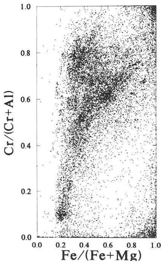
FIG. 2. \text{Cr}/(\text{Cr} + \text{Al}) versus \text{Fe}^{2+}/(\text{Fe}^{2+} + \text{Mg}) plot of 16 093 samples of spinel in the database.
