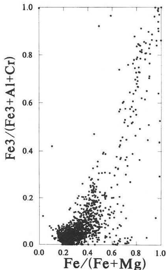
FIG. 12. \text{Fe}^{3+}/(\text{Fe}^{3+} + \text{Al} + \text{Cr}) versus \text{Fe}^{2+}/(\text{Fe}^{2+} + \text{Mg}) plot of spinel samples from xenoliths found in alkali basalts and kimberlites.
