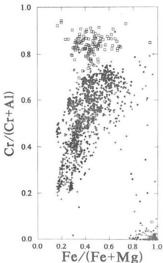
FIG. 5. \text{Cr}/(\text{Cr} + \text{Al}) versus \text{Fe}^{2+}/(\text{Fe}^{2+} + \text{Mg}) plot of spinel samples from boninitic basalts (open squares), ocean-island basalts (solid dots) and mid-ocean-ridge basalts (crosses).
