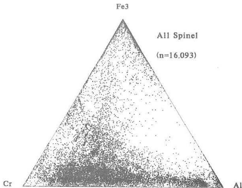
FIG. 7. \text{Cr} - \text{Al} - \text{Fe}^{3+} plot of all spinel samples in the database.
