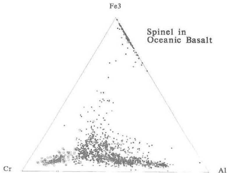
FIG. 8. \text{Cr} - \text{Al} - \text{Fe}^{3+} plot of spinel samples from boninitic basalts (open squares), ocean-island basalts (solid dots) and mid-ocean-ridge basalts (crosses).
