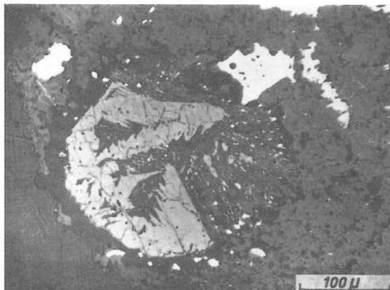
FIG. 21. Skeletal crystal of chromite in a feldspar matrix in a chondrule from the equilibrated Salisbury chondrite, as seen in reflected light. The photo is reprinted from Ramdohr (1973) with permission (see Acknowledgements).
