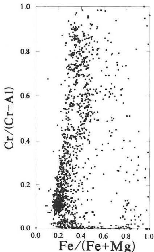
FIG. 11. \text{Cr}/(\text{Cr} + \text{Al}) versus \text{Fe}^{2+}/(\text{Fe}^{2+} + \text{Mg}) plot of spinel samples from xenoliths found in alkali basalts and kimberlites.
