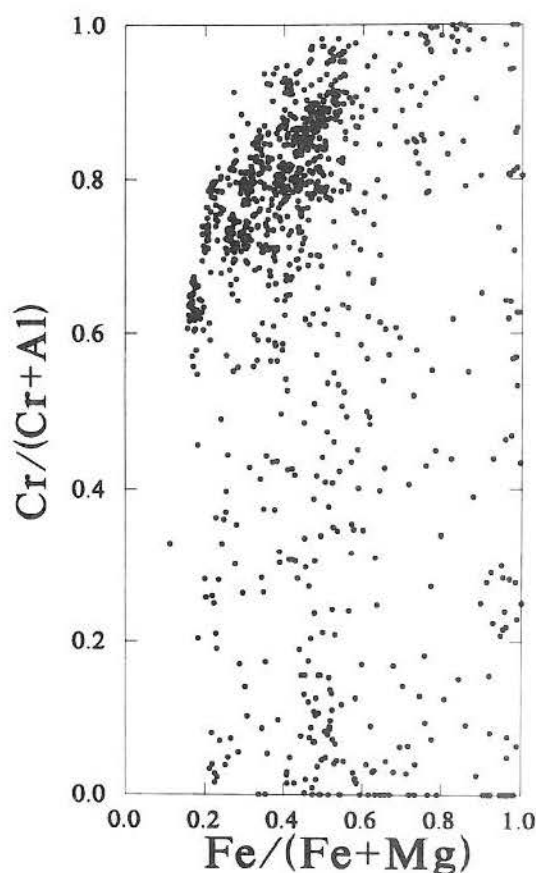
FIG. 13. \text{Cr}/(\text{Cr} + \text{Al}) versus \text{Fe}^{2+}/(\text{Fe}^{2+} + \text{Mg}) plot of spinel samples from kimberlites.
