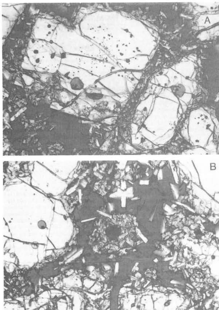
FIG. 1. Photomicrographs in transmitted light of a sample from the Kilauea Iki lava lake (sample K175-1-141.5) drilled in 1975 (Scowen et al. 1991). Width of field: 9 mm. A. Large phenocrysts of olivine containing small opaque crystals of chromite and surrounded by small crystals of clinopyroxene and plagioclase laths in a matrix of glass. B. An opaque crystal of chromite surrounded by a rim of clinopyroxene in a matrix of glass. Large clear phenocrysts of olivine also are surrounded by clinopyroxene.
