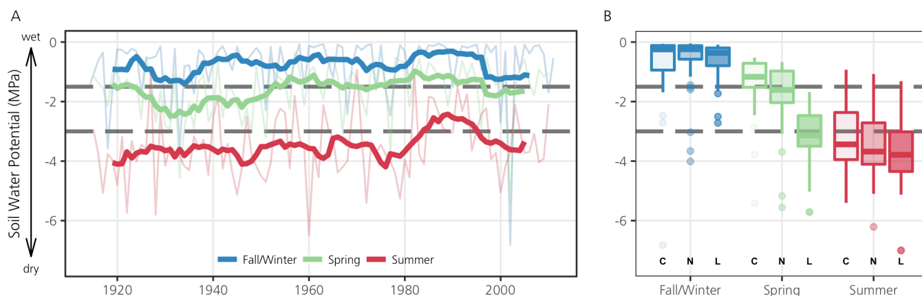
Figure 3. Historical (A) and future projections (B) of soil water potential (SWP) at intermediate soil depths (20–50 cm) in the shallow loamy mesa-top pinyon-juniper woodland ecosystem in Mesa Verde NP for three seasons: fall/winter (October–February), spring (March–June), and summer (July–September). Panel A shows historical annual variability (fine lines) and moving 10-year averages (thick lines) of drying and wetting from 1915–2010. Panel B compares variability amongst years for three time periods, current (C; 1970–2010), near future (N; 2020–2059), and long-term future (L; 2060–2099), grouped by season. Boxplot whiskers are 1.5 times the inter-quartile range of values, while dots are values outside this range. Dashed lines in both panels highlight plant-relevant SWP levels: traditional wilting point (-1.5 MPa) and a drylands wilting point (-3.0 MPa; Kolb and Sperry 1999a, 1999b).
