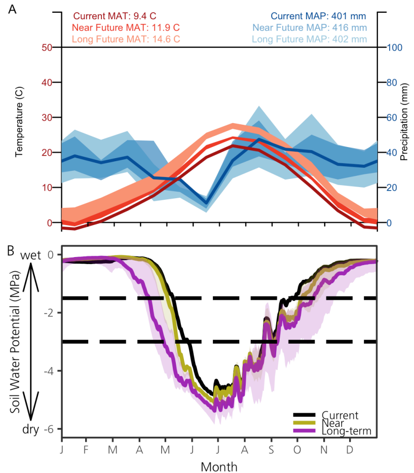
Figure 4: Panel A. Average seasonal patterns of climate in the shallow loamy mesa-top pinyon-juniper woodland ecosystem in Mesa Verde NP. Climate diagram (Walter and Leith 1967) shows mean monthly temperature (°C) and precipitation (mm) in dark red and blue lines, respectively, in the current period (1970–2010). Shaded red and blue areas indicate the range of potential values in the near (darker area; 2020–2059) and long-term (lighter area; 2060–2099) future periods. Mean annual temperature (MAT) and mean annual precipitation (MAP) are derived from the mean monthly values. Panel B. Average daily SWP for the current period (1970–2010; black), near future (2020–2059; yellow), and long-term future (2060–2099; purple). For future time periods, thick lines represent the median value among climate models, while shaded areas represent the range of values from the 11 th to 89 th percentile, removing both the highest and lowest model values.
