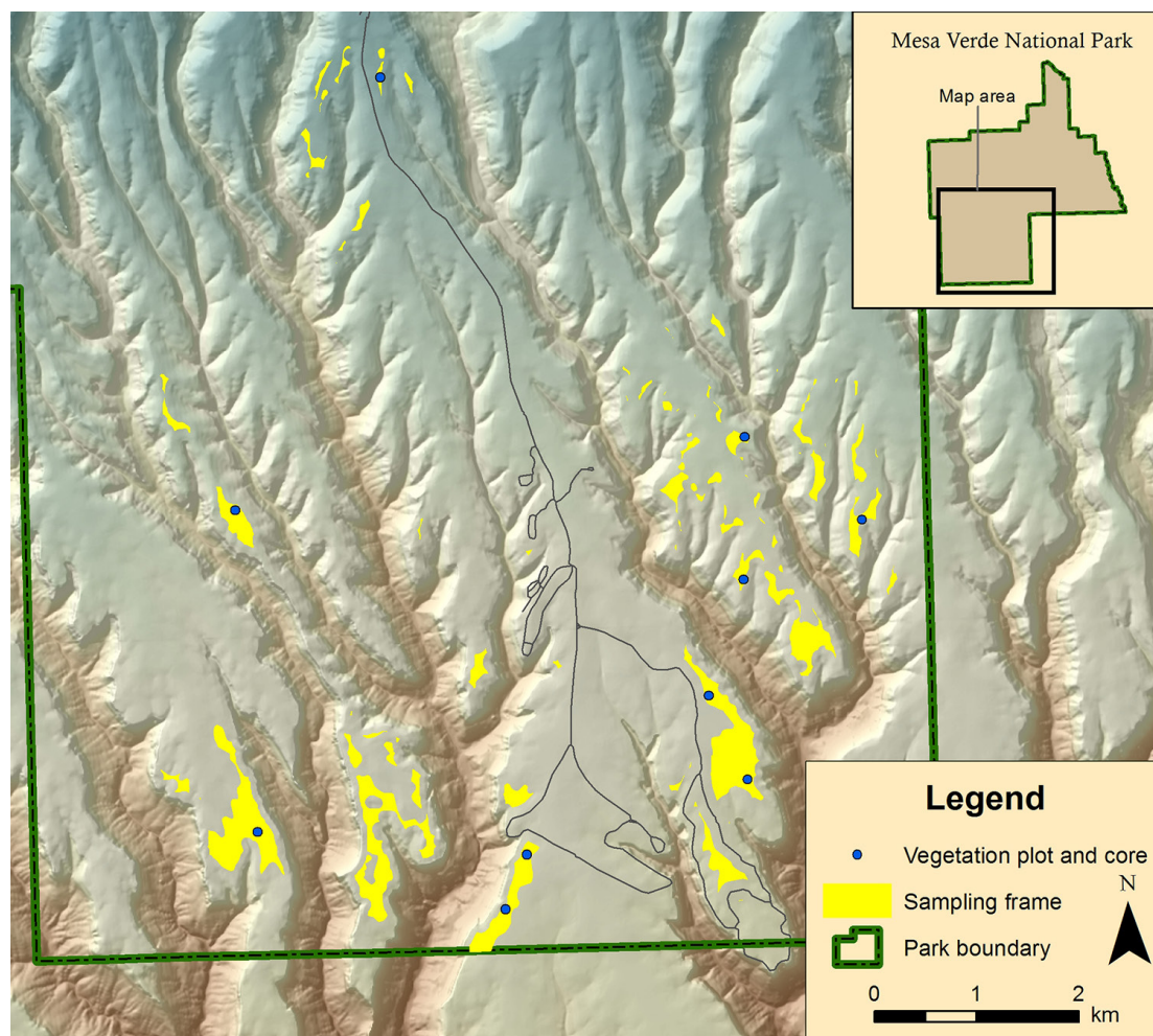
Figure 2. Map of Mesa Verde NP showing Southern Colorado Plateau Network monitoring plots in the shallow loamy mesa-top pinyon-juniper woodland ecosystem. Plots from which soil cores were used are indicated as solid blue dots. NPS map.
