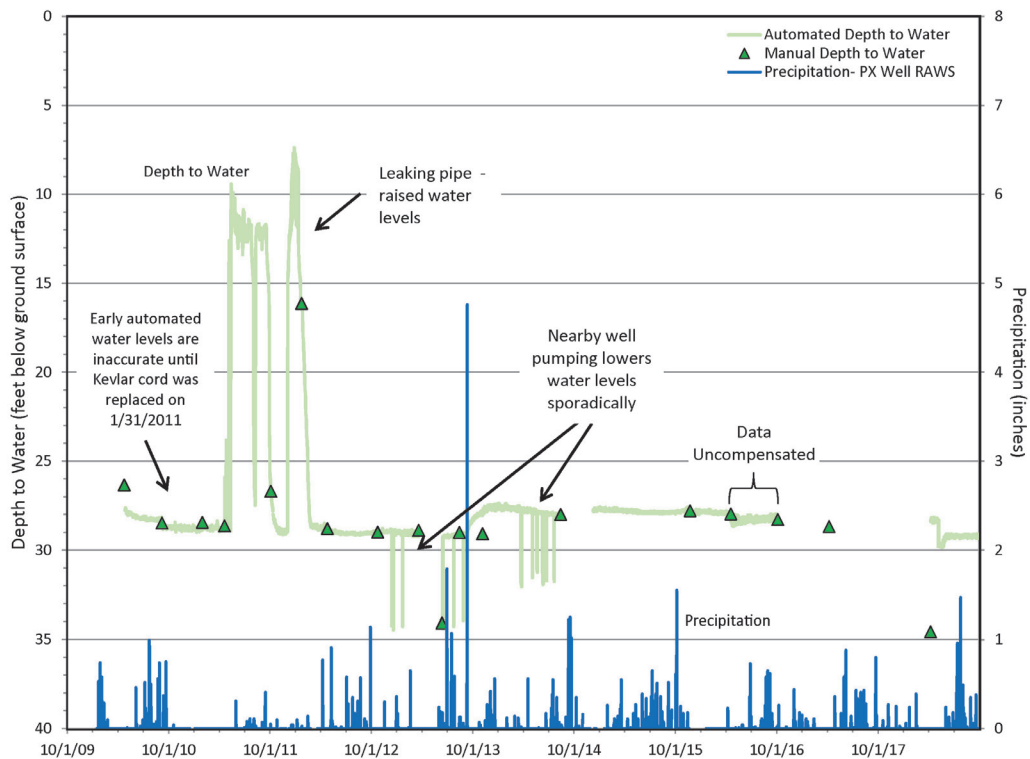
Figure 3-2. Depth to water below ground surface (bgs) at Lemonade Well with daily precipitation from the PX Well RAWS, water years 2010–2018, Guadalupe Mountains NP
