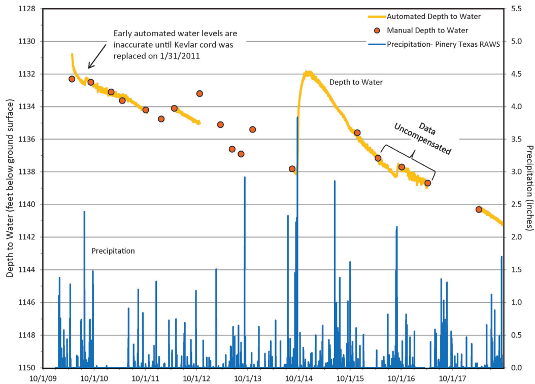
Figure 3-1. Depth to water below ground surface (bgs) at Signal Peak Well with daily precipitation from the Pinery RAWS, water years 2010–2018, Guadalupe Mountains NP
