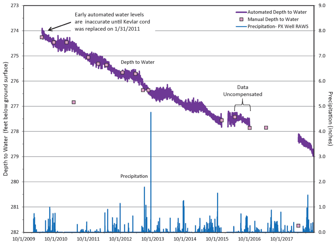
Figure 3-3. Depth to water below ground surface (bgs) at PX Well with daily precipitation from the PX Well RAWs, water years 2010–2018, Guadalupe Mountains NP
