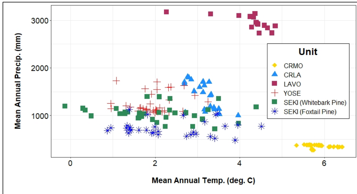
Figure 2. Climatic setting for white pine plot locations in Craters of the Moon National Monument and Preserve (CRMO), Crater Lake National Park (CRLA), Lassen Volcanic National Park (LAVO), Sequoia and Kings Canyon National Parks (SEKI), and Yosemite National Park (YOSE).
