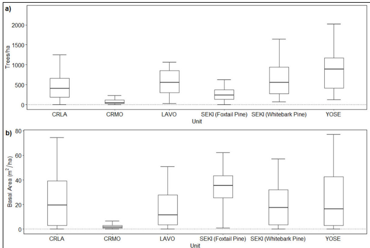
Figure 10. Boxplots of a) total tree density and b) basal area for white pine monitoring plots in five National Park Service units. Upper and lower whiskers represent the 95 th and 5 th percentiles, respectively. Upper and lower limits of the box represent the 75 th and 25 th percentiles, respectively, and lines represent medians.
