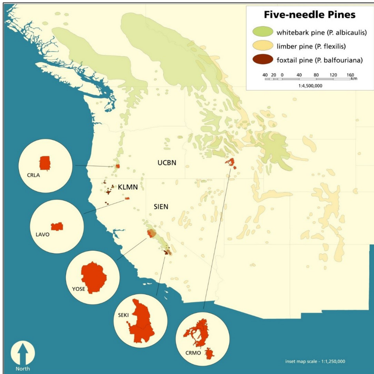
Figure 1. Geographic distribution of the ranges of limber pine, white bark pine, and foxtail pine from Little (1971) with locations of five National Park Service units (McKinney et al. 2012).
