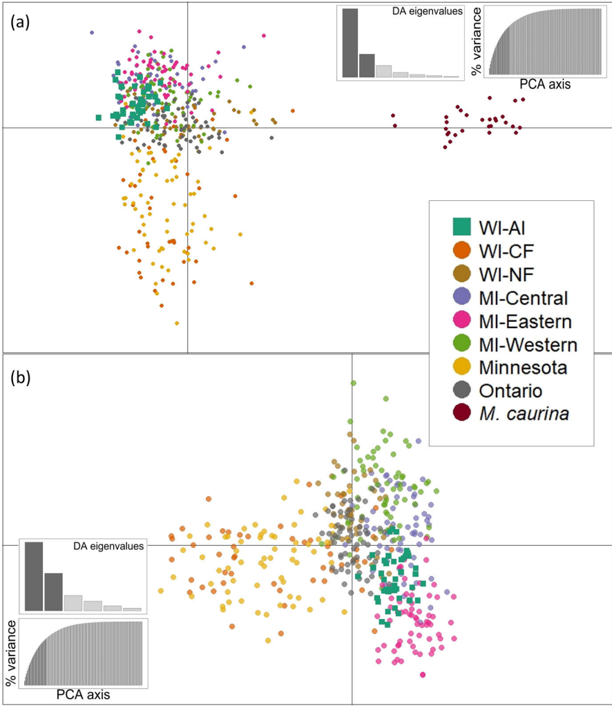
FIG. 2. Discriminant analysis of principle components of American marten ( Martes americana ) populations from the regional recovery network: Chequamegon National Forest, Wisconsin, United States (WI-CF), Nicolet National Forest, Wisconsin, United States (WI-NF), central Upper Michigan (MI-Central), eastern Upper Michigan (MI-Eastern), western Upper Michigan (MI-Western), Minnesota, Ontario, and with (a) and without (b) Pacific marten ( Martes caurina ). Predicted position of martens from the Apostle Islands (WI-AI) within the discriminant functions are symbolized with squares. Scatterplots of individuals along the first two discriminant functions eigenvalues. Included insets show the number of principal components analysis axis retained and discriminant functions eigenvalues.
