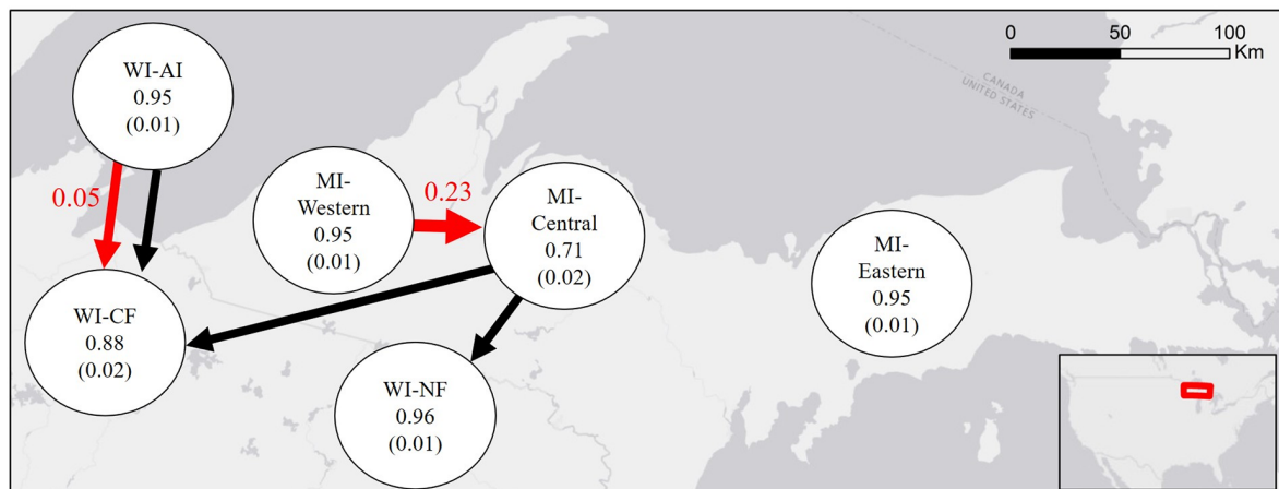
FIG. 3. Indirect gene flow between subpopulation pairs of American marten ( Martes americana ) within a regional recovery network: Apostle Islands (WI-AI), Chequamegon National Forest, Wisconsin, United States (WI-CF), Nicolet National Forest, Wisconsin, United States (WI-NF), central Upper Michigan (MI-Central), eastern Upper Michigan (MI-Eastern), and western Upper Michigan (MI-Western). Values in nodes represent proportion of sampled population from source population with standard deviation in parentheses and red values and arrows represent estimated recent gene flow that did not overlap zero at 95% confidence interval from BAYESASS. Black arrows represent significant directionality of relative gene flow between populations estimated from G_{ST} with 95% confidence from divMigrate.
