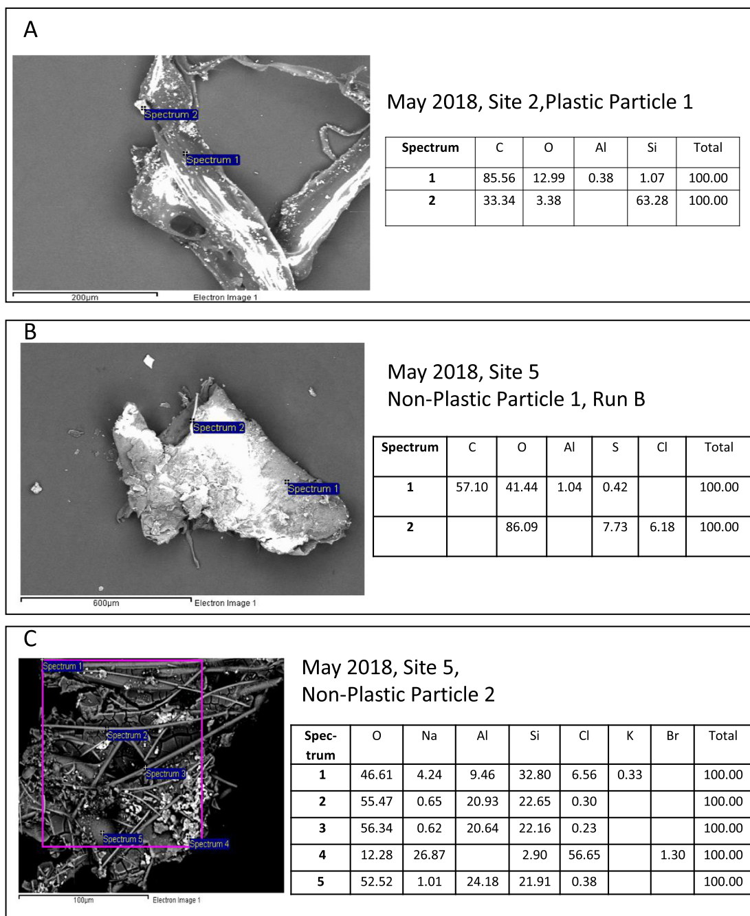
Fig. 6. SEM/EDS data for the following particles from beach sands sampled in May 2018: A. A particle from Site 2 found to be plastic by melt test. B and C. Particles that did not melt, thus considered non-plastic, from Site 5. Sites analyzed by each EDS spectrum are labeled, with the resulting elemental data for each spectrum given in percentages.
