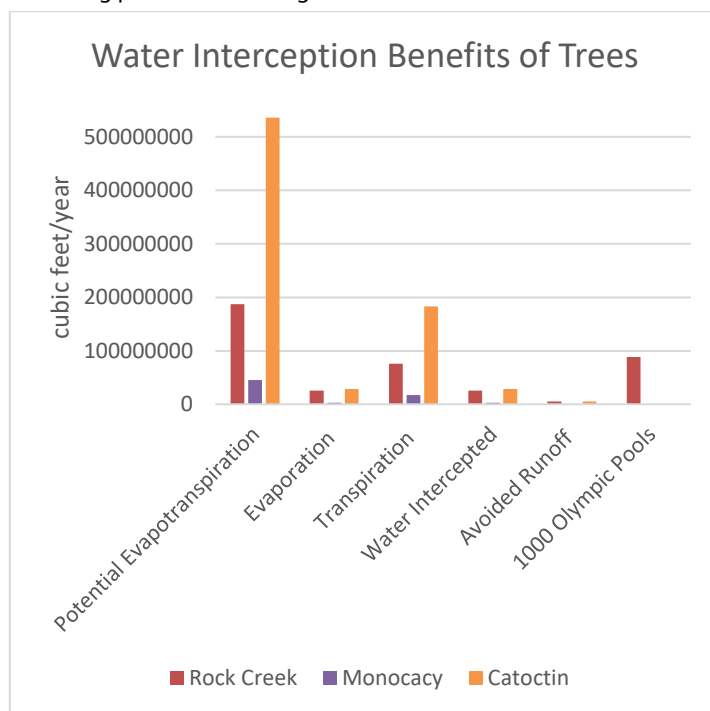
Figure 4. Avoided runoff value of trees in Rock Creek, Monocacy, and Catoctin.
