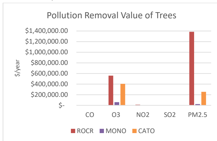
Figure 2. Monetary value of pollution removal capability of trees in Rock Creek, Monocacy, and Catoctin.
