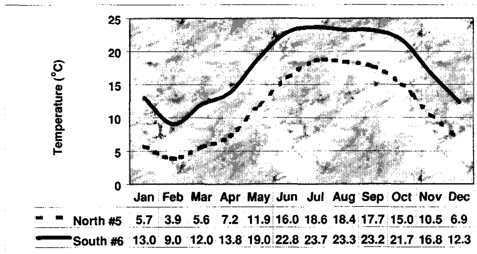
Figure 7.01.7.—Comparison of monthly soil temperature averages between north and south aspect sites.
