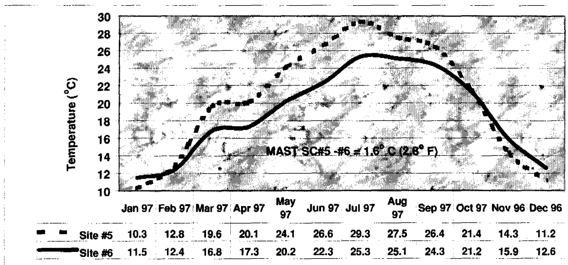
Figure 7.25.2.—Average monthly soil temperatures at 10 cm for sites 5 and 6.
