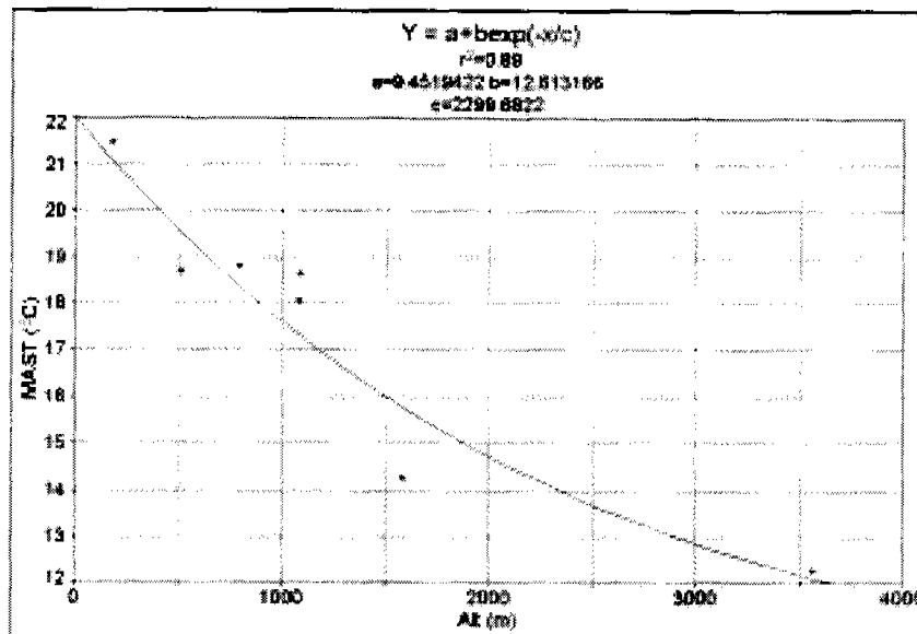
Figure 4.6.—Regression equation for eight sites on the Big Island of Hawaii.
