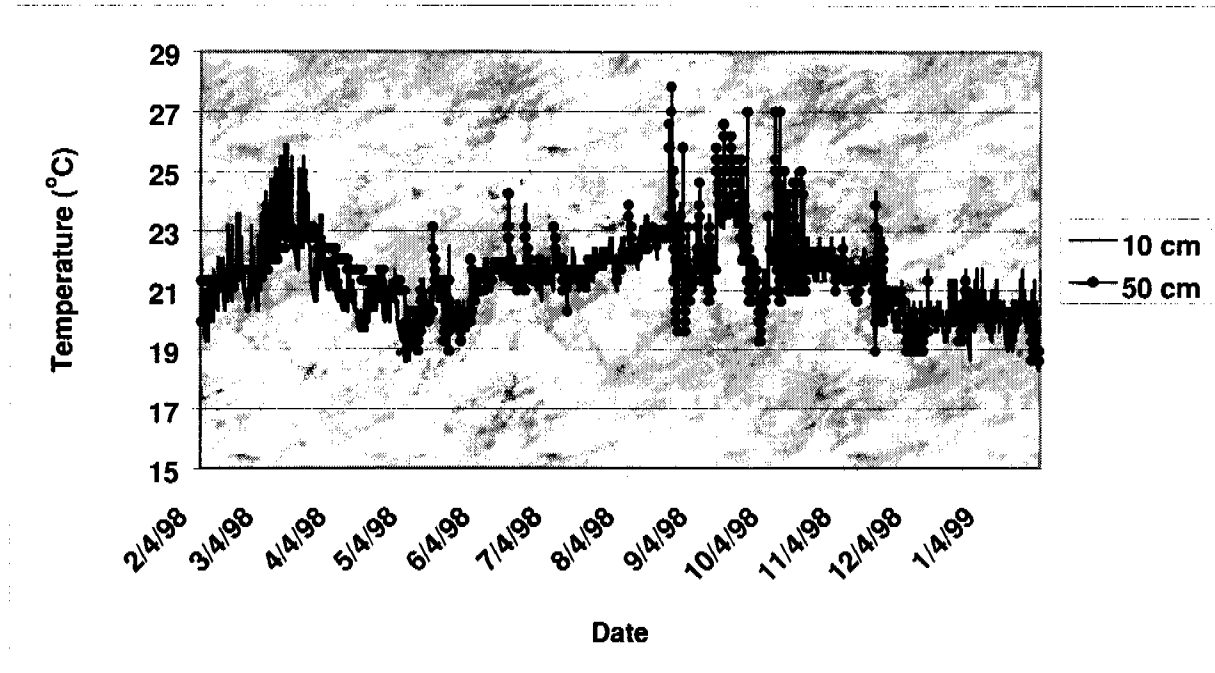
Figure 7.10.4.—Coincident exothermic spiking at 10 cm and 50 cm for the macadamia orchard site in Hawaii.
