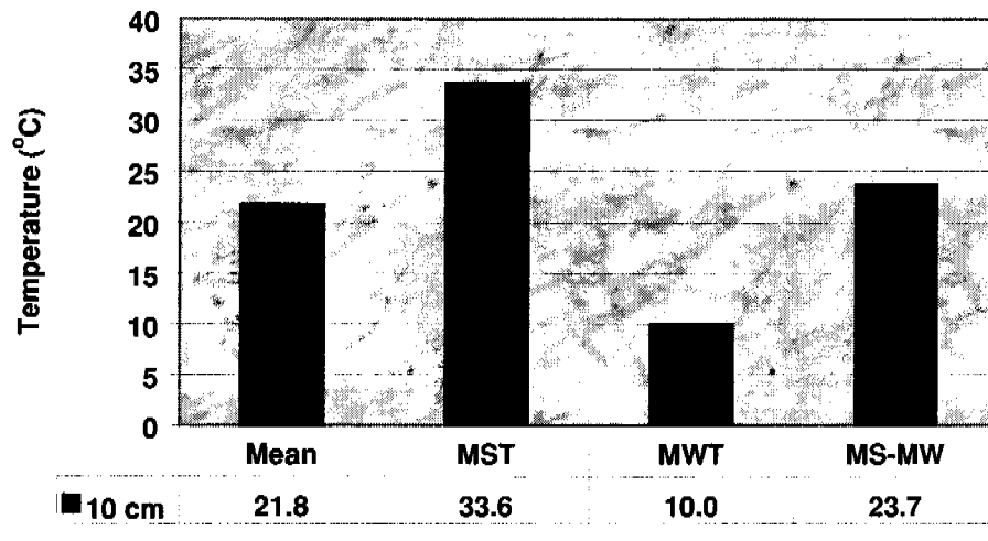
Figure 7.02.2.—Seasonal and annual analysis for the 10-cm depth at site 5.
