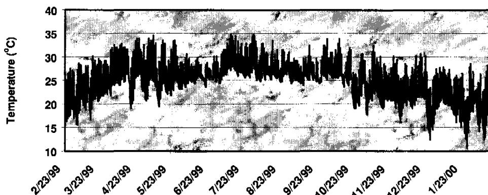
Figure 7.07.4.—Soil temperature signature at 10 cm for site 5.
