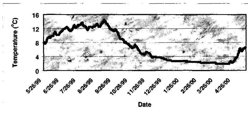
Figure 7.15.1.—Soil temperature signature at 50 cm for site 1.
