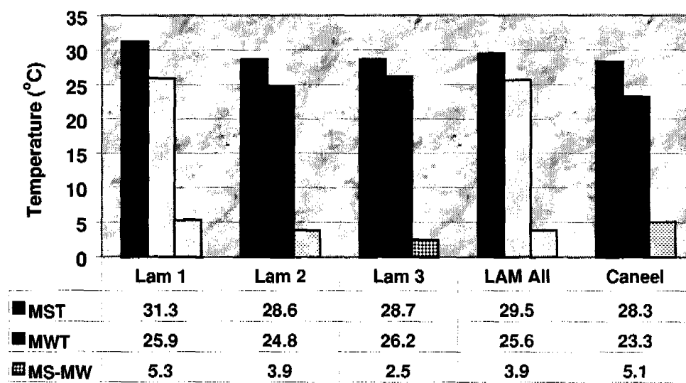
Figure 7.28.4.—MST, MWT, and isotivity values at Lameshur Bay and Caneel Hill.
