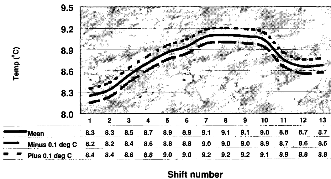
Figure 7.19.2.—Shift analysis of soil temperature at 50 cm for site 2.
