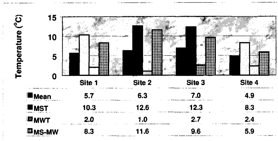
Figure 7.31.1.—Seasonal and annual comparisons at 50 cm among the four sites in the study area.
