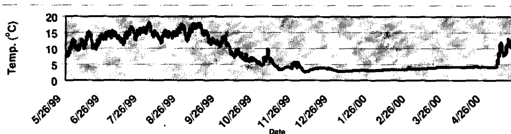
Figure 7.15.2.—Soil temperature signature for the 10-cm depth at site 3.
