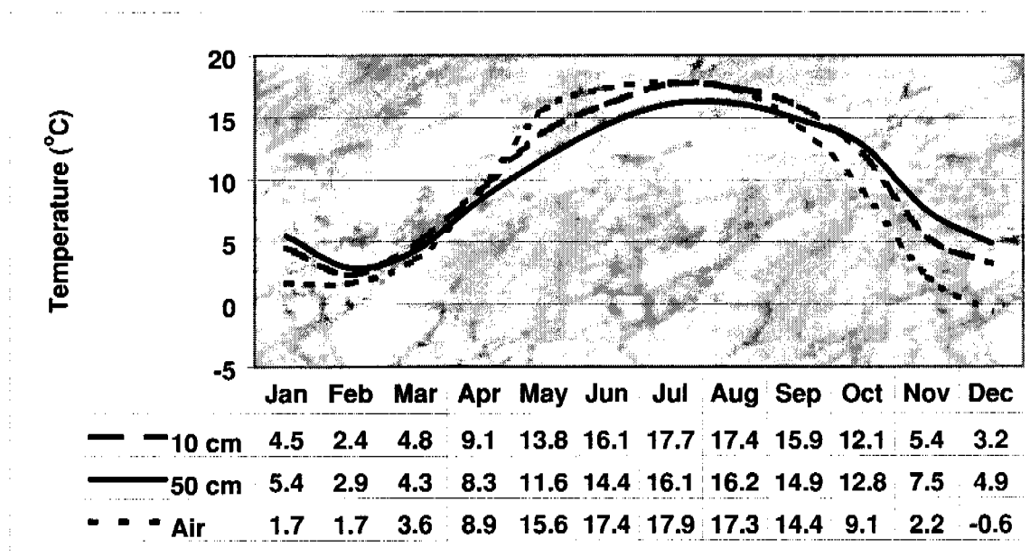
Figure 7.27.1.—Comparison of monthly air and soil temperatures at site 7.
