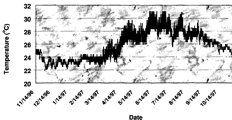
Figure 7.28.1.—Soil temperature signature for the 20-cm soil depth at Caneel Hill.
