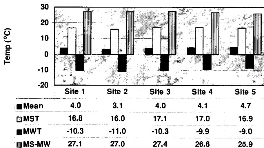
Figure 7.15.5.—Seasonal and annual summaries of air temperature in Maine.
