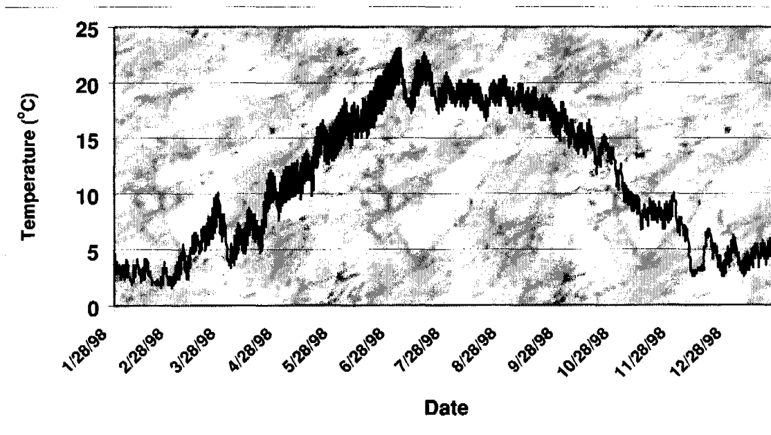
Figure 7.01.4.—Soil temperature signature of the 10-cm depth at site 5.
