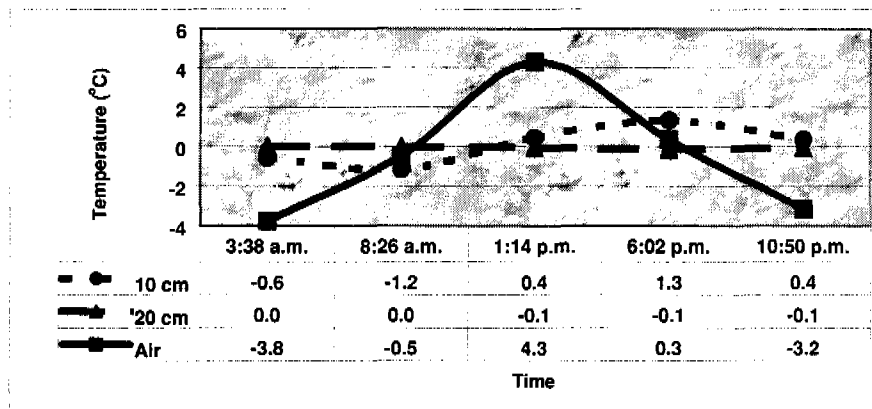
Figure 7.05.4.—Time analysis for air and soil temperatures at site 2.
