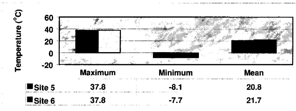
Figure 7.01.8.—Comparison of mean annual air temperatures for sites 5 and 6.
