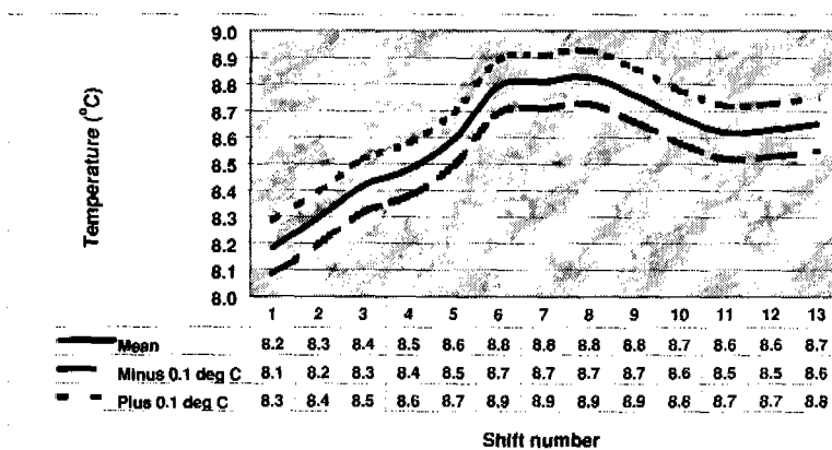
Figure 7.22.1.—Shift analysis for the 50-cm depth at the Jake's Rock site.
