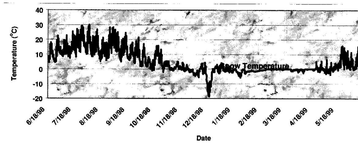
Figure 7.31.2.—Impact of snowfall on air temperature at site 4.
