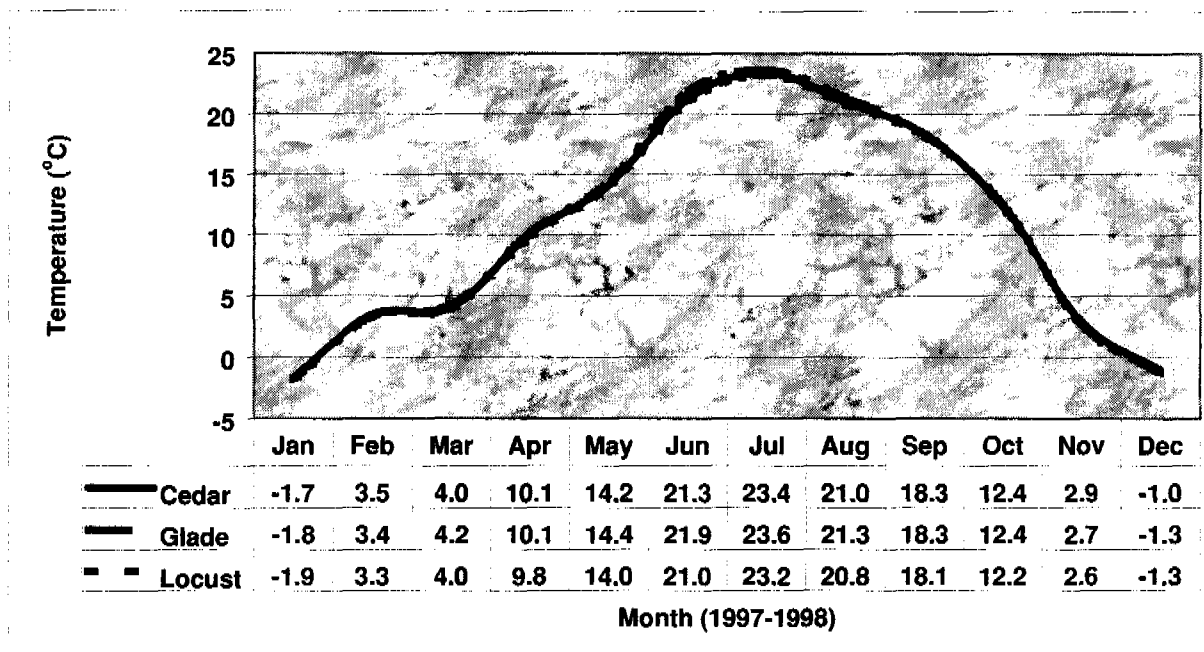
Figure 3.2.—Air temperature signatures and monthly averages at three sites within 100 m of each other in western Illinois.
