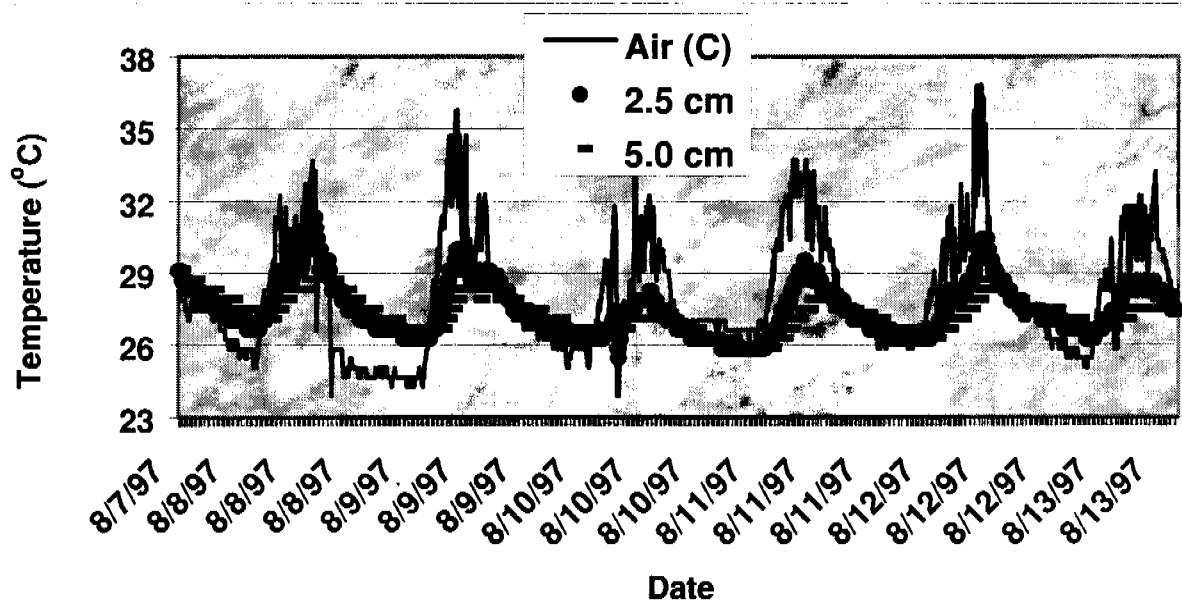
Figure 7.24.6.—Relationship between air temperature and soil temperature readings.
