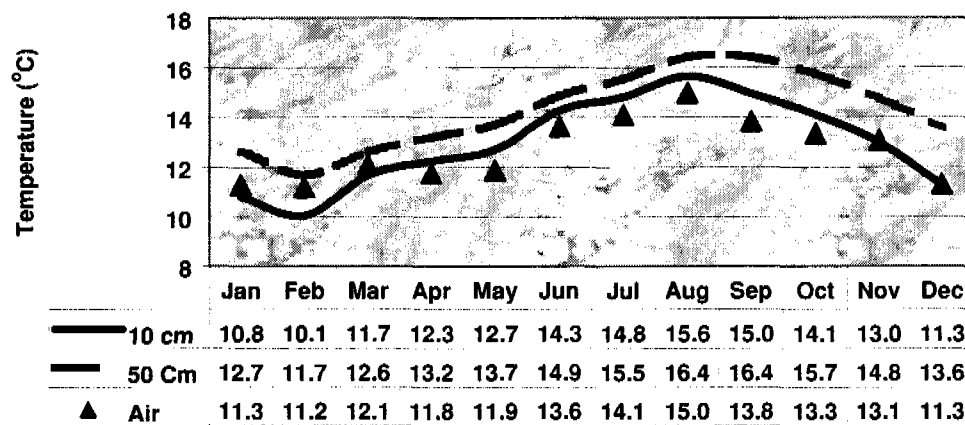
Figure 7.09.6.—Relationship of monthly temperatures at the Hanaipoe site.
