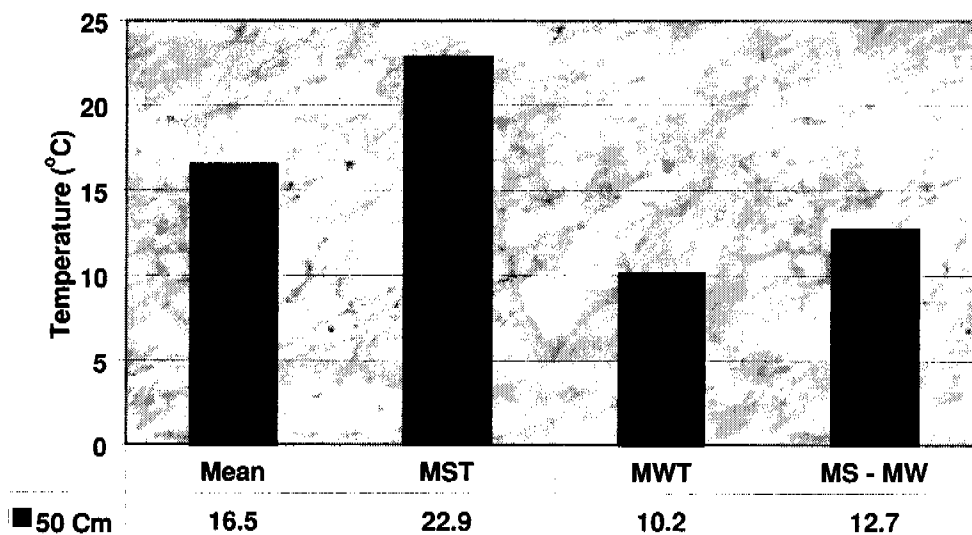
Figure 7.03.2.—An example of annual and seasonal analysis of soil temperature for the 50-cm depth.
