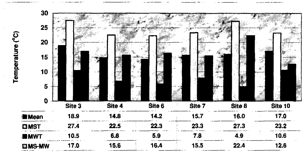
Figure 7.14.7.—Soil temperature at 10 cm for the study area.
