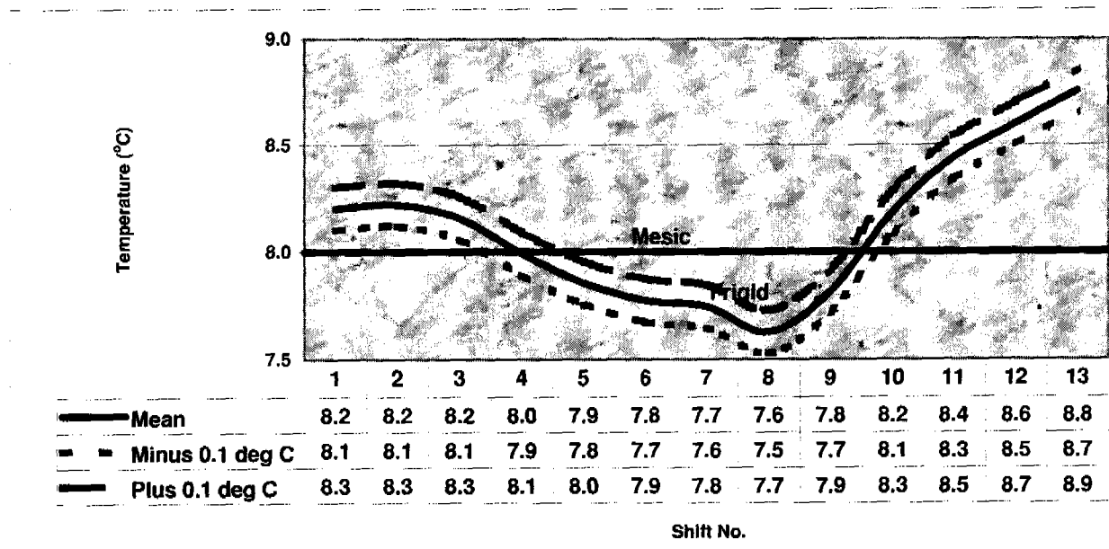
Figure 7.33.2.—Shift analysis of the 10-cm soil temperature at site 7.
