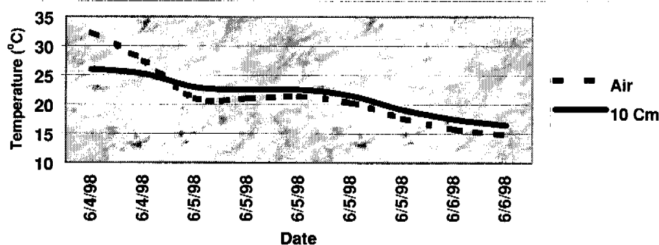
Figure 7.03.5.—Relationship of air temperature to 10-cm soil temperature from June 4 to June 6, 1998.
