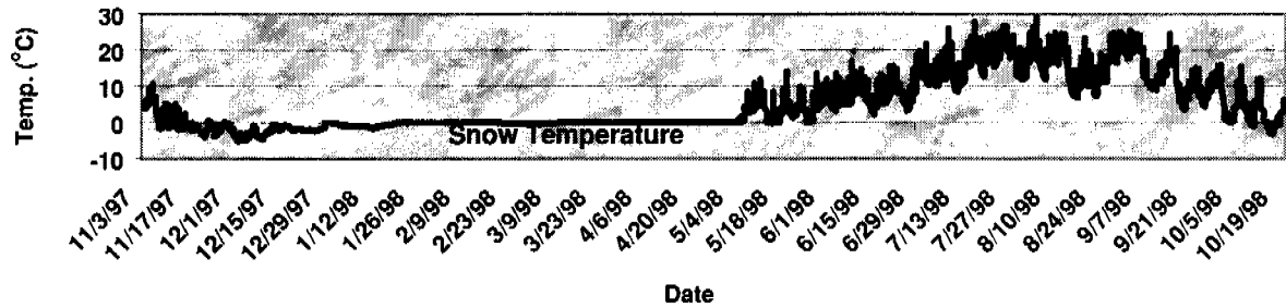
Figure 7.12.1.—Influence of snowpack on air temperature at site 4.
