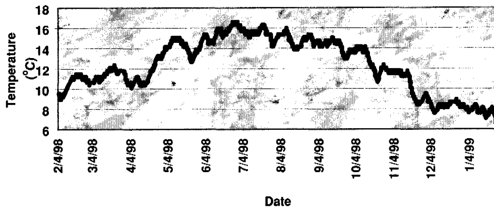
Figure 7.08.2.—Temperature signature of the 50-cm soil depth on Mauna Kea.
