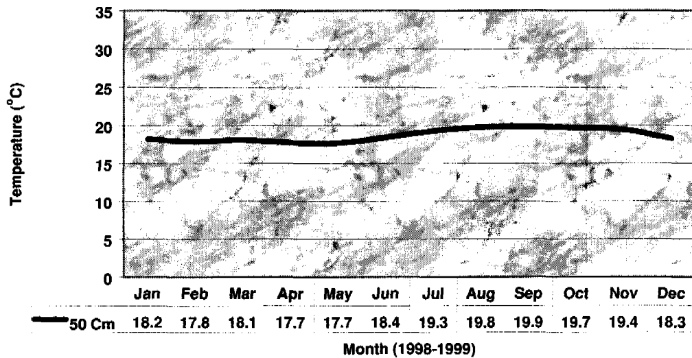
Figure 5.8.—Isothermic temperature signature of a soil in a rain forest on the Big Island of Hawaii.
