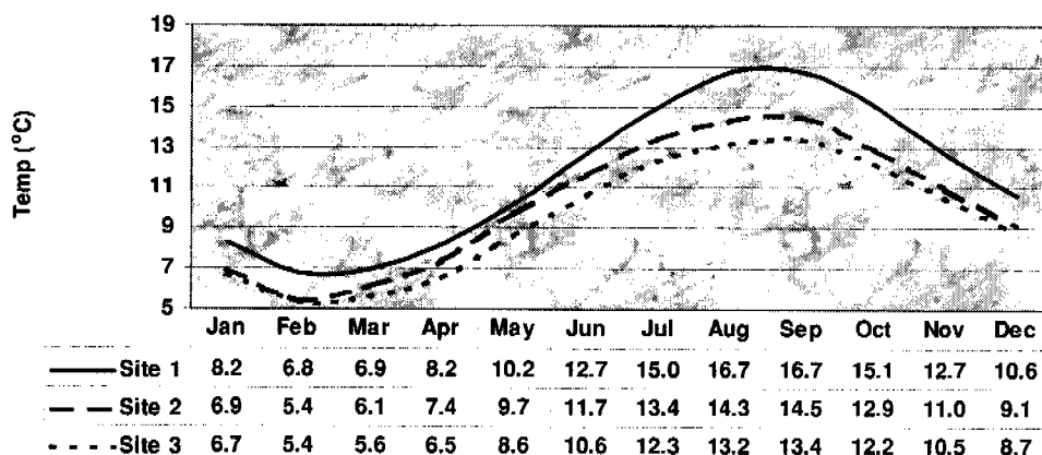
Figure 7.23.2.—Average monthly soil temperatures for the three sites during the second year.
