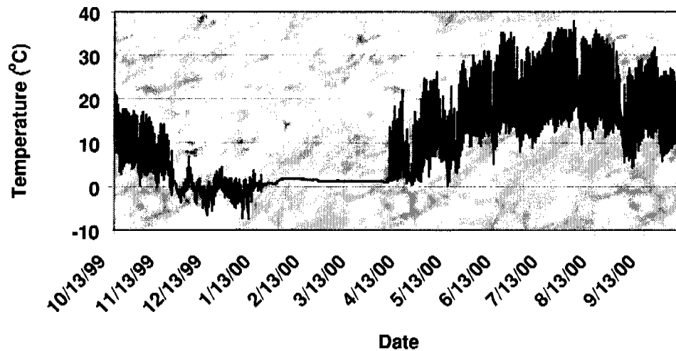
Figure 7.17.3.—Soil temperature signature at 10 cm for site 7 displaying extreme diurnal fluctuation during July.
