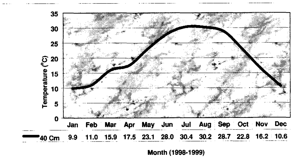
Figure 5.5.—A hyperthermic temperature regime in a soil in the Grand Canyon in Arizona.
