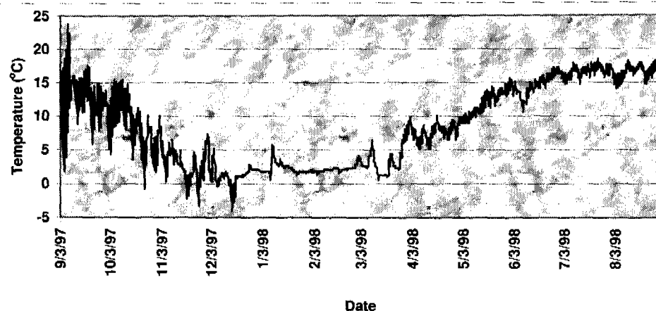
Figure 7.33.1.—Air temperature signature at site 7.
