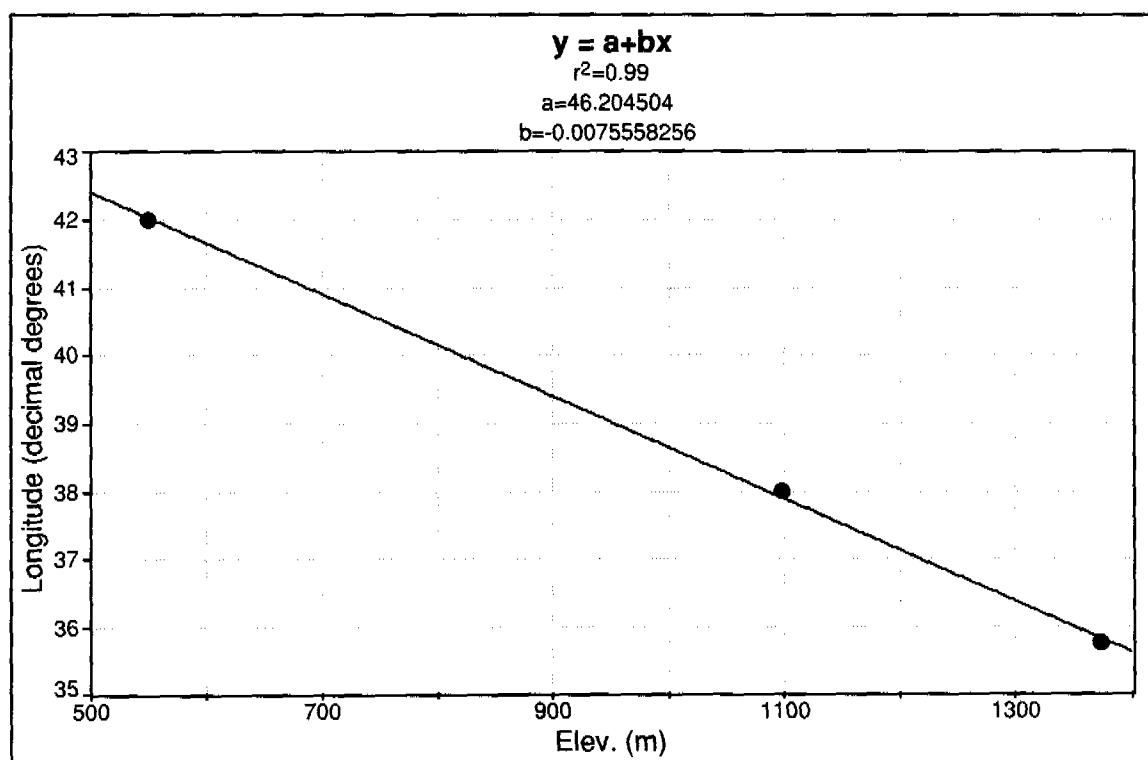
Figure 7.18.2.—Regression equation used to differentiate mesic and frigid soils in MO 13.
