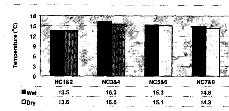
Figure 7.30.1.—Relationship of MAST for the poorly drained (wet) and well drained (dry) soils in North Carolina.
