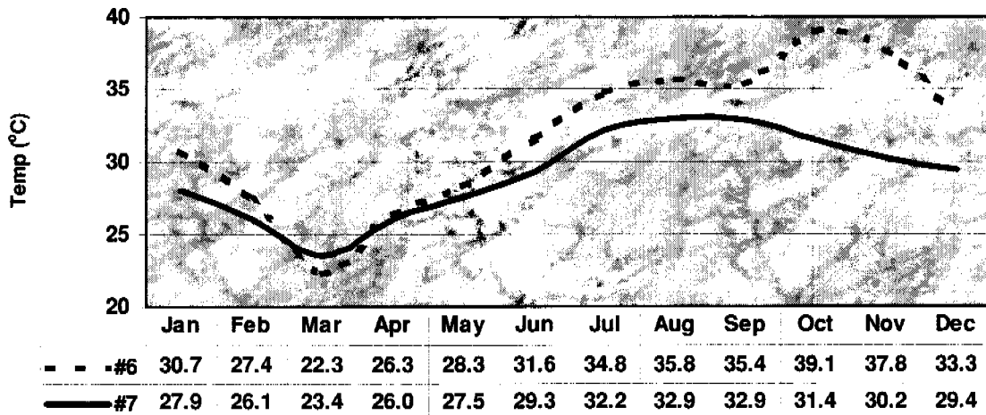
Figure 7.07.5.—Average monthly soil temperatures for the 43-cm depth at sites 6 and 7.
