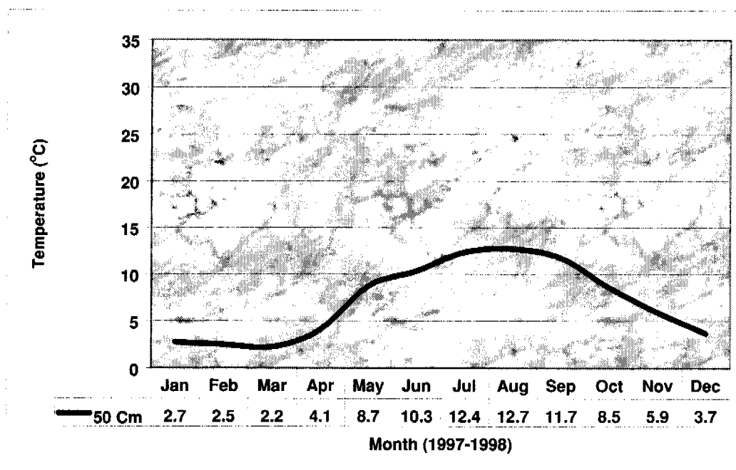
Figure 5.2.—A frigid temperature regime in a soil in Grafton County, New Hampshire.
