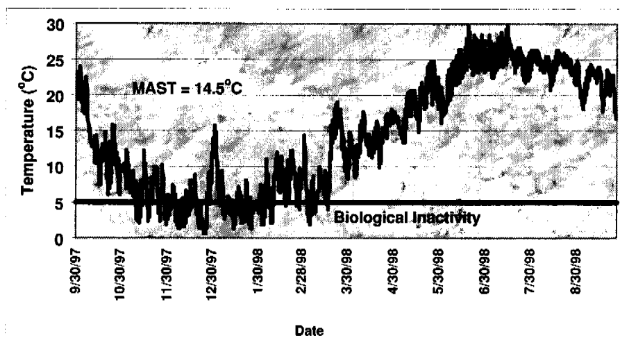
Figure 7.29.3.—Biological activity for the 25-cm depth at site 1.
