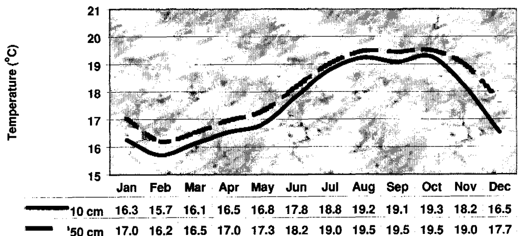
Figure 7.09.4.—Monthly soil temperature averages for the KDC 2 site.
