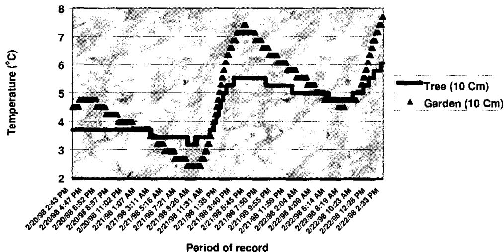
Figure 4.1.—Short-term study of soil temperature at a depth of 10 cm in Lincoln, Nebraska.
