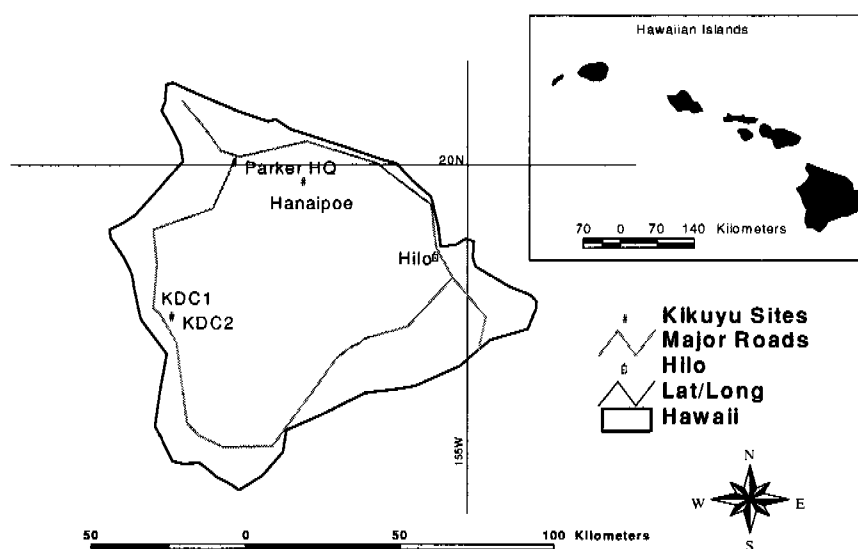
Figure 7.09.1.—Location of the temperature sites in the study area.
