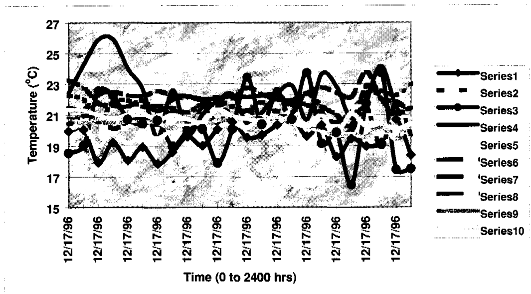
Figure 3.3.—Inaccurate soil temperature readings at 10 cm for 10 sites on St. John Island.
