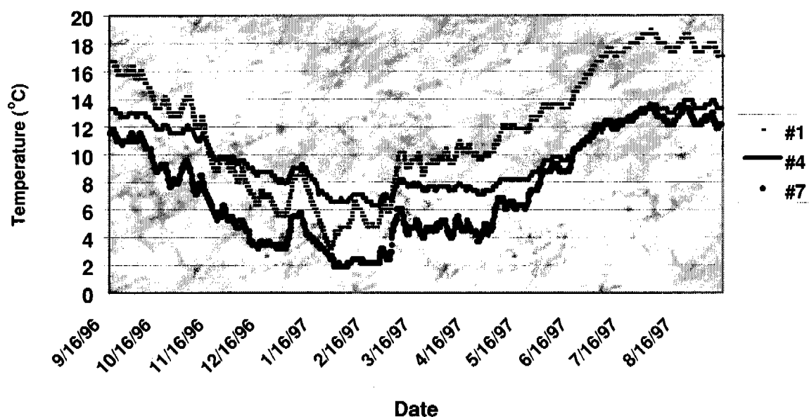
Figure 7.26.1.—Soil temperature signatures for the 50-cm soil depth at sites 1, 4, and 7.
