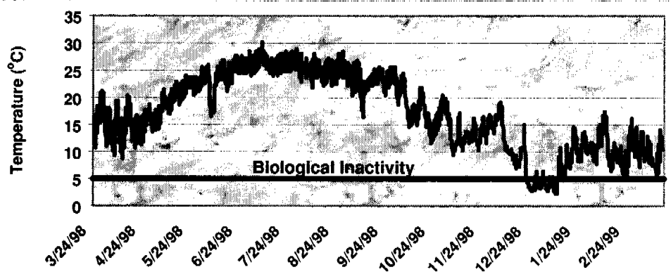
Figure 7.03.4.—Dates of biological activity for the 10-cm soil depth in Arkansas.
