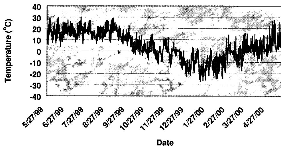
Figure 7.15.3.—The air temperature signature at site 5.
