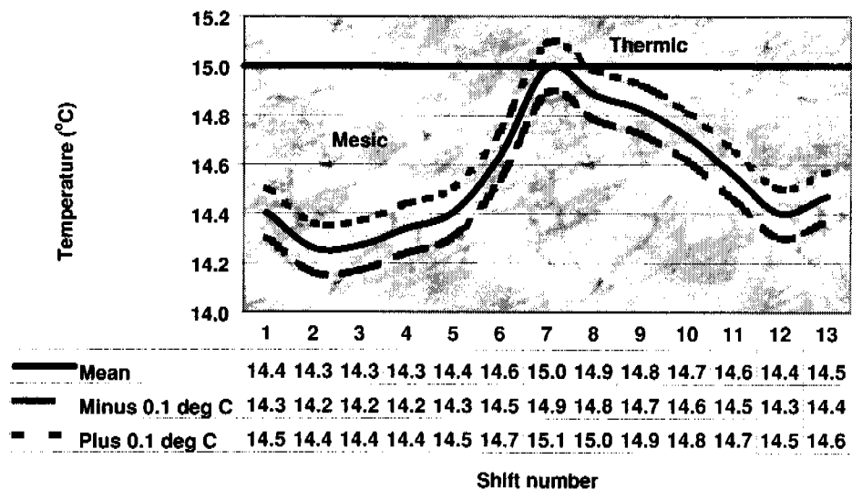
Figure 7.20.2.—Shift analysis for the soil temperature at New York City site 2.
