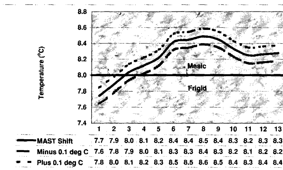
Figure 7.18.1.—Shift analysis for the soil temperature at Bay site 4.
