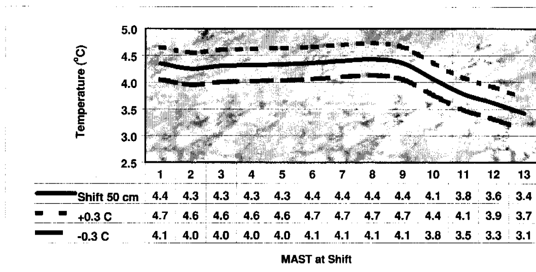
Figure 7.12.6.—Shift analysis for the 50-cm soil depth at site 10.
