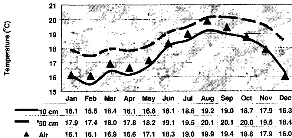
Figure 7.09.5.—Relationship of monthly air and soil temperatures at the Parker HQ site near Waimea.
