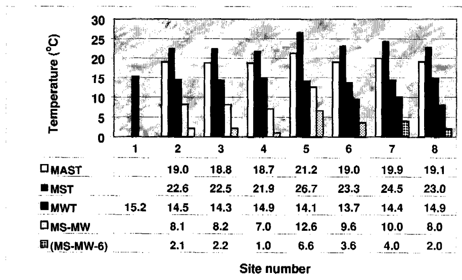
Figure 7.25.1.—Average seasonal and annual soil temperatures at 50-cm for sites in the study area.
