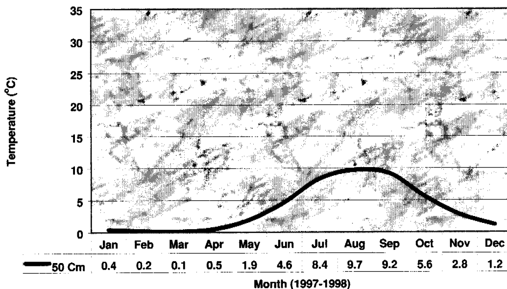
Figure 5.1.—A cryic temperature regime in a soil in Wyoming.
