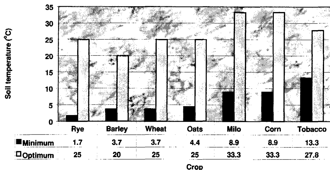
Figure 2.1.—Minimum and optimum soil temperature for germination of various crops.
