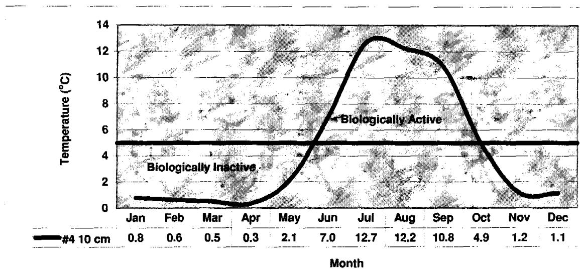
Figure 7.11.4.—Biological activity at 10-cm for Idaho site 4.
