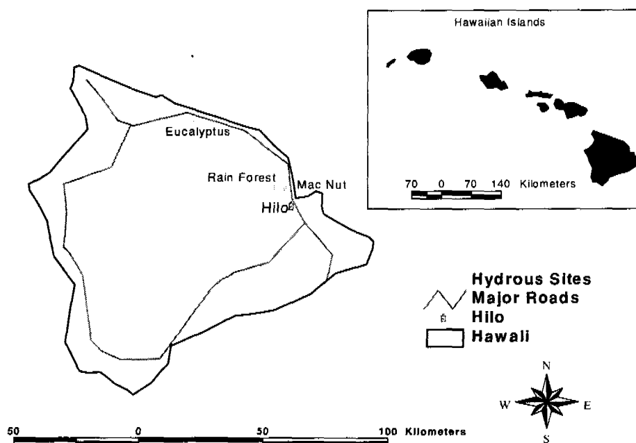
Figure 7.10.1.—Location of temperature sites in the study area.
