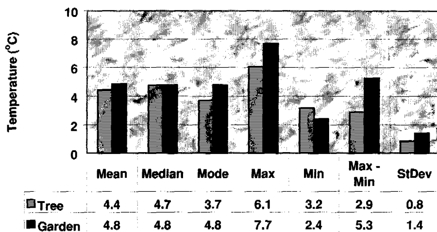
Figure 4.2.—Summary of soil temperature data for the 2-day study in Lincoln, Nebraska.
