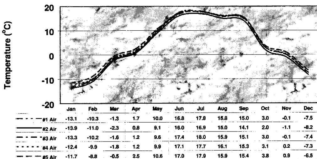
Figure 7.15.4.—Monthly air temperature signatures for sites in Maine.
