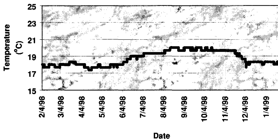
Figure 7.08.3.—Temperature signature of the 50-cm soil depth at the Hamakua forest site.
