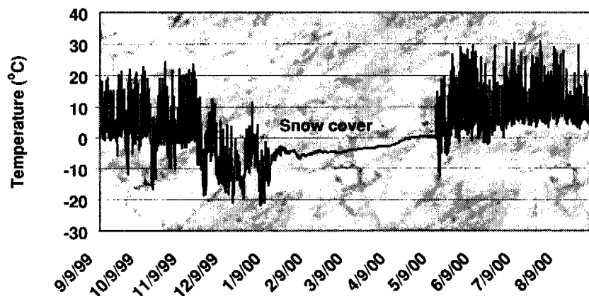
Figure 7.06.2.—Impact of snowfall on the air temperature signature at site 4.
