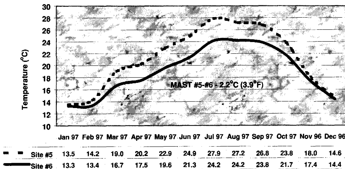
Figure 7.25.3.—Mean monthly soil temperatures at 50 cm for sites 5 and 6.
