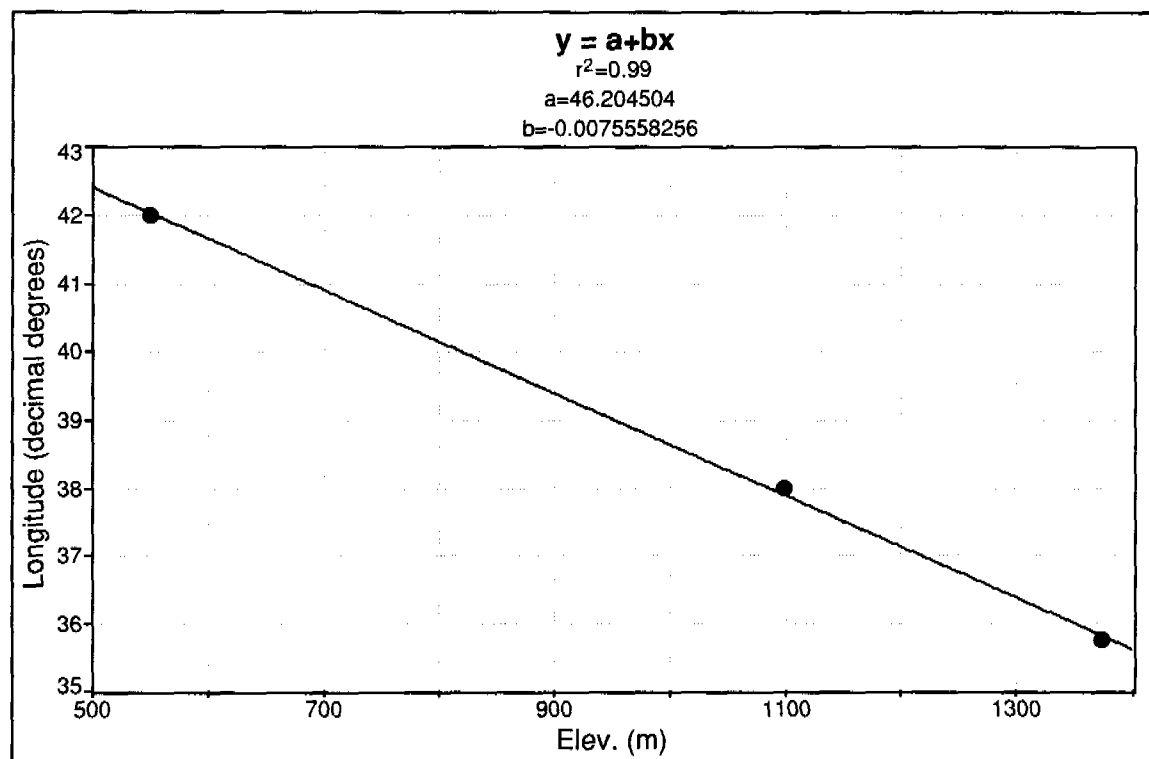
Figure 7.22.2.—Regression equation used to differentiate mesic and frigid soils in MO 13.
