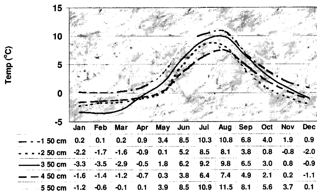
Figure 7.06.1.—Average monthly soil temperatures at 50 cm for the Guanella Pass study area.
