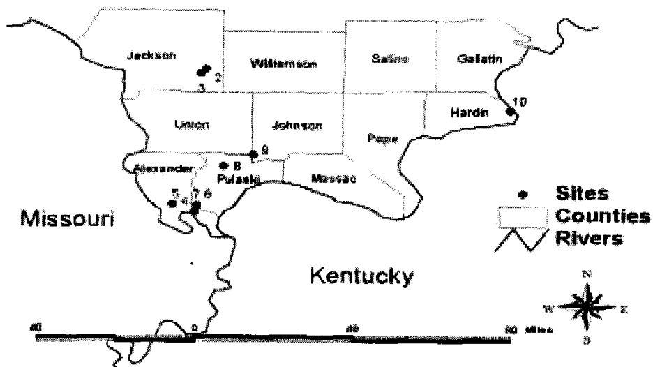
Figure 7.14.1.—Location of the sites in the soil temperature study area.
