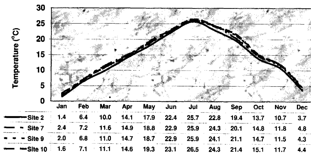
Figure 7.14.6.—Monthly air temperature signatures for sites in Illinois.
