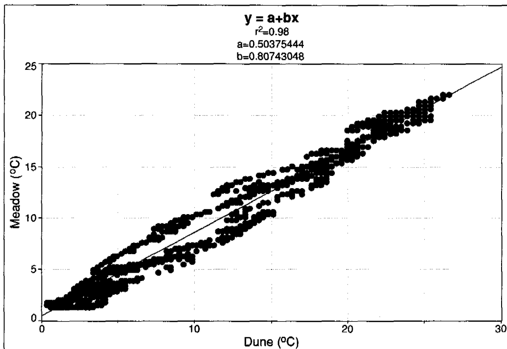
Figure 4.7.—Correlation of the 50-cm soil temperature at two sites in the Sand Hills of Nebraska.
