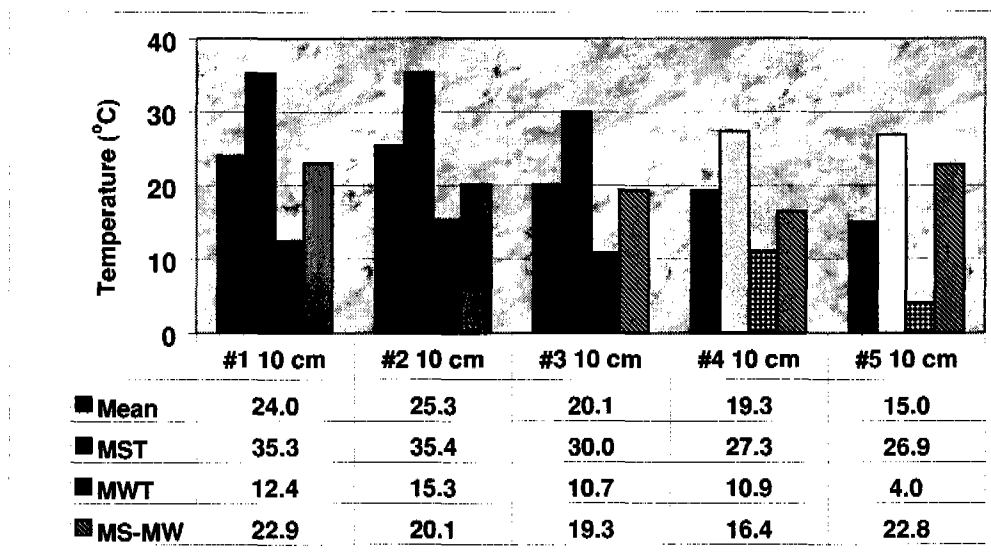
Figure 7.04.3.—Seasonal and annual soil temperature averages for the 10-cm depth.
