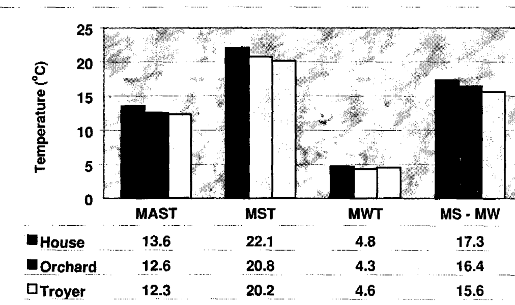
Figure 7.13.4.—Seasonal and annual analysis of the 50-cm soil depth in the study area.
