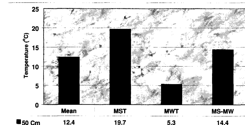
Figure 6.4.—An example of annual and seasonal analysis for soil temperature at 50 cm from a site in Missouri.
