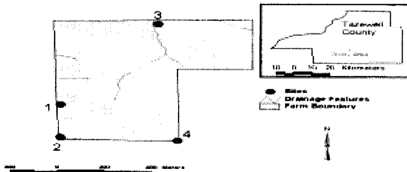
Figure 7.13.1.—Location of the sites in the study area.
