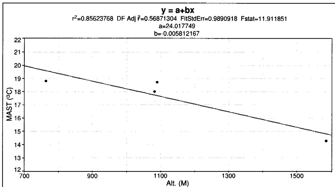
Figure 7.09.7.—A straight-line regression formula for the sites in kikuyugrass.
