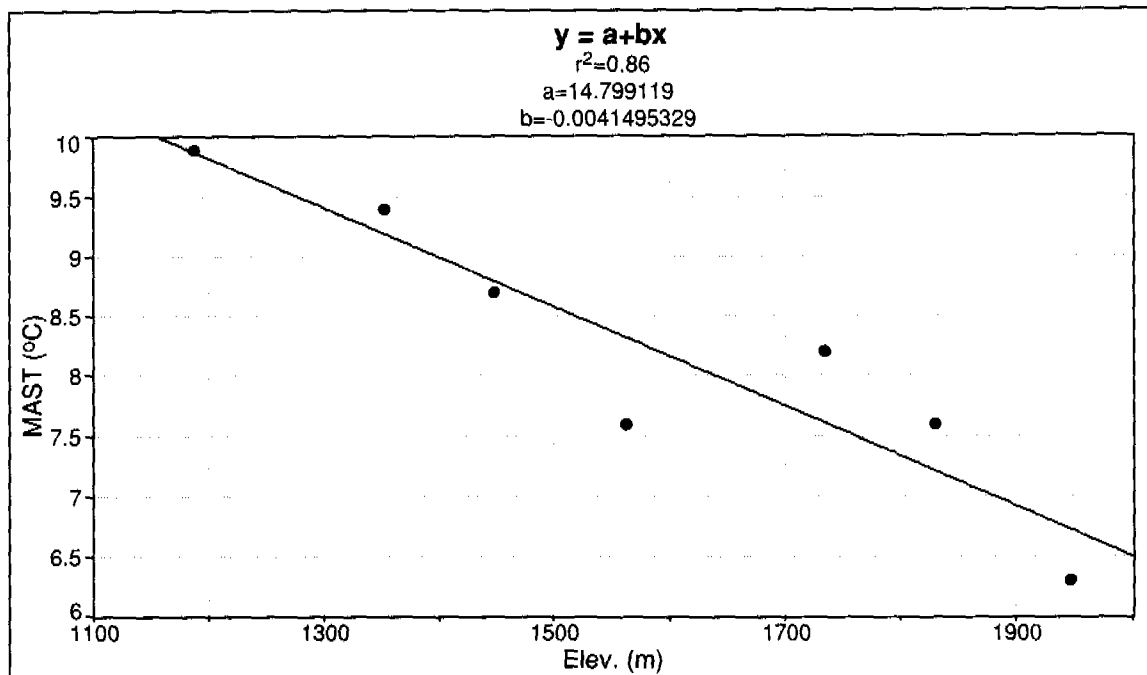
Figure 7.27.2.—Trend of MAST at 50 cm to elevation in the Great Smoky Mountains of Tennessee.
