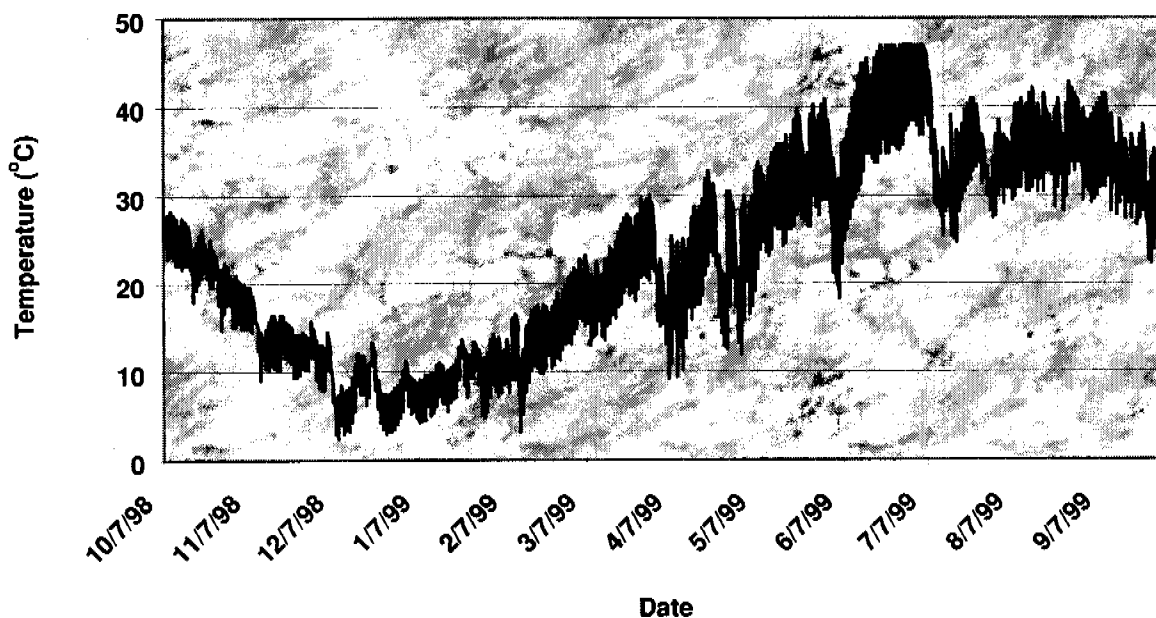
Figure 7.02.3.—Annual signature displaying maximum readings of the 10-cm depth at site 4 during July.
