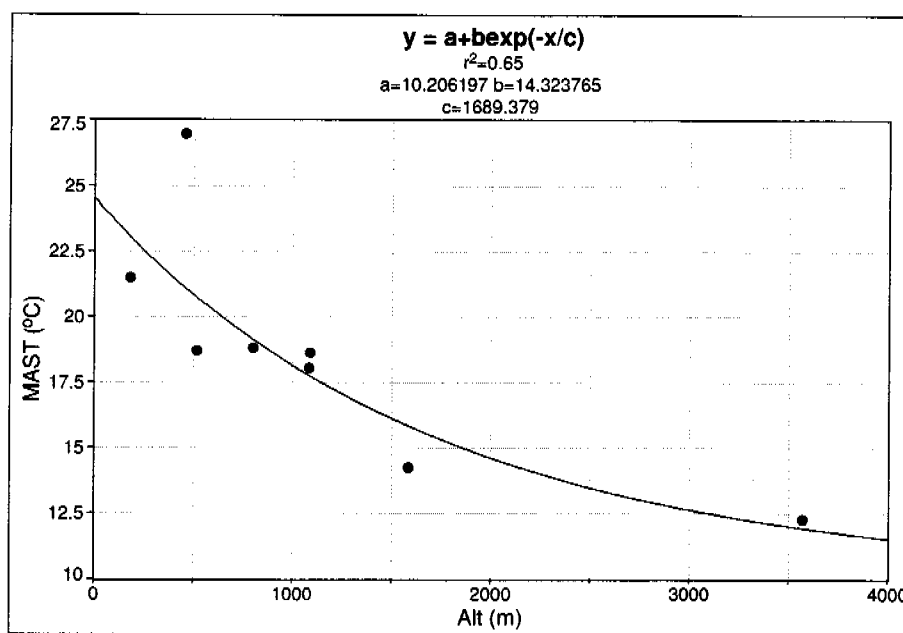
Figure 7.08.4.—Regression analysis comparing MAST and altitude for sites on the Island of Hawaii.
