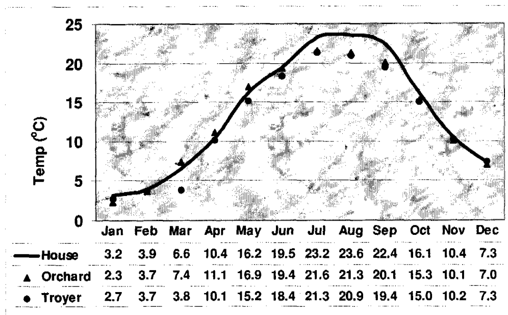
Figure 7.13.3.—Average monthly soil temperatures for the 50-cm depth.
