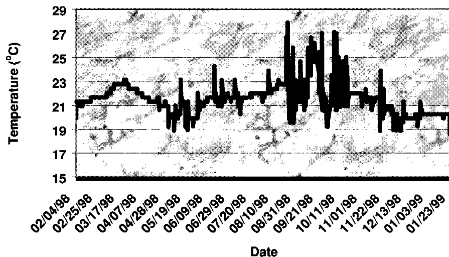
Figure 7.10.3.—Exothermic spikes at the 50-cm soil depth for the macadamia orchard site near Hamakua.
