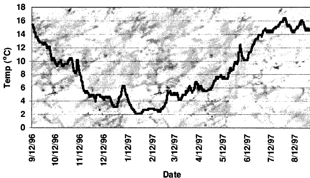
Figure 4.3.—Annual soil temperature at 50 cm for a site in West Virginia.
