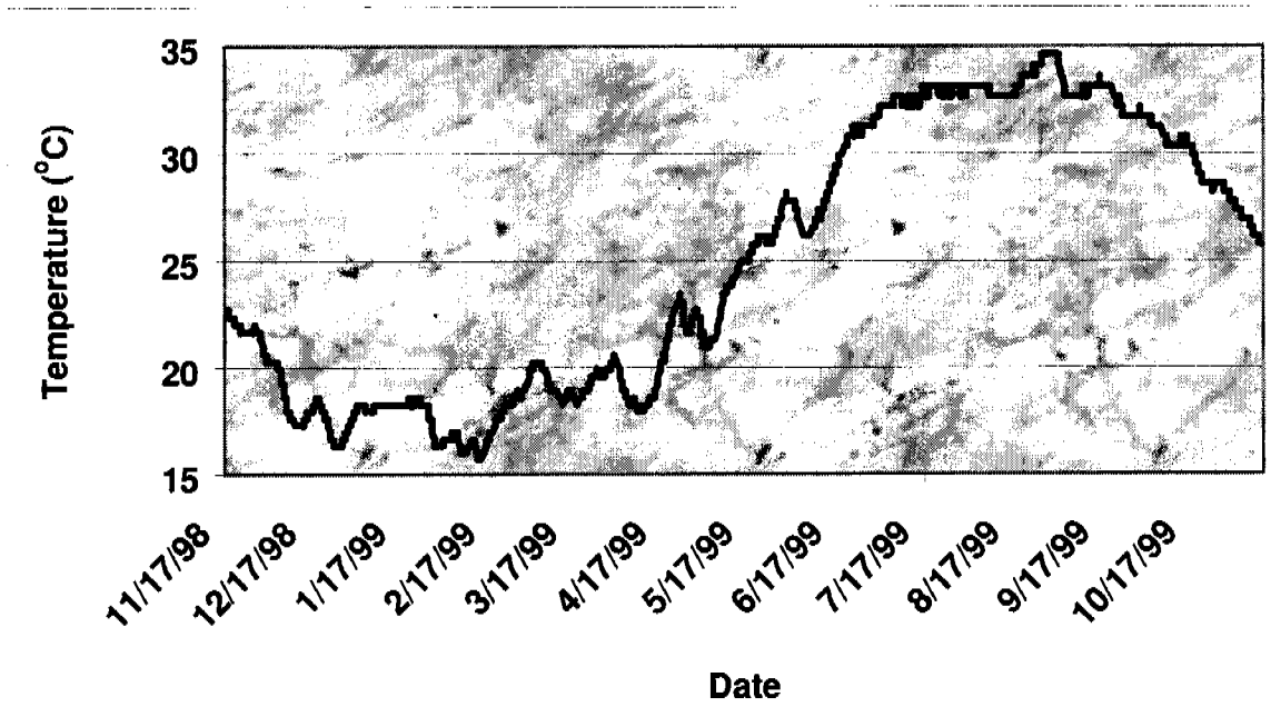
Figure 7.04.1.—Soil temperature signature at 50 cm for site 2.
