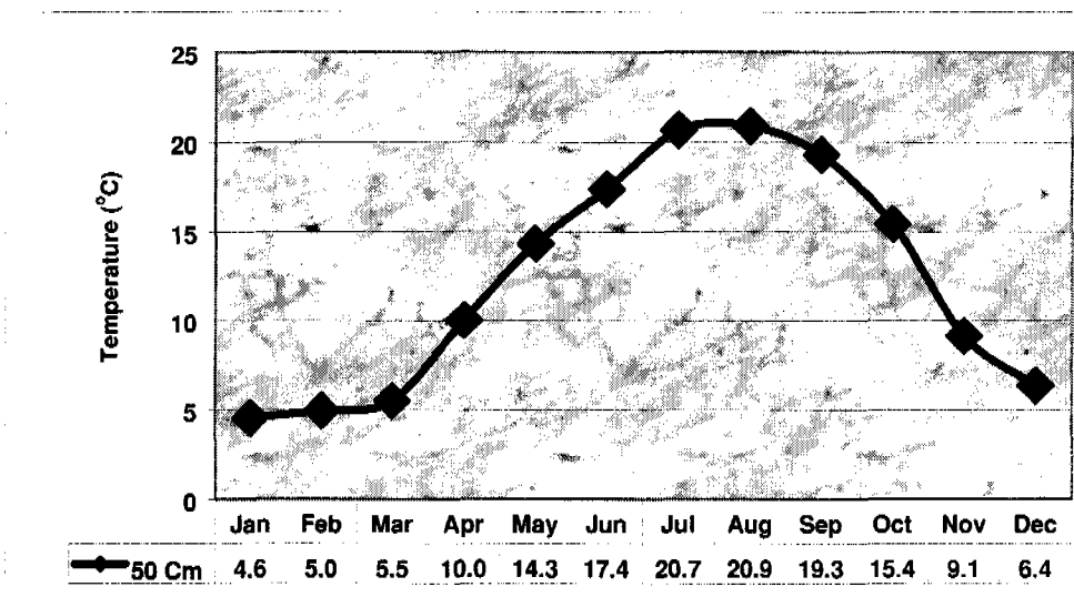
Figure 6.3.—Monthly soil temperature averages at 50 cm for a site in Missouri.
