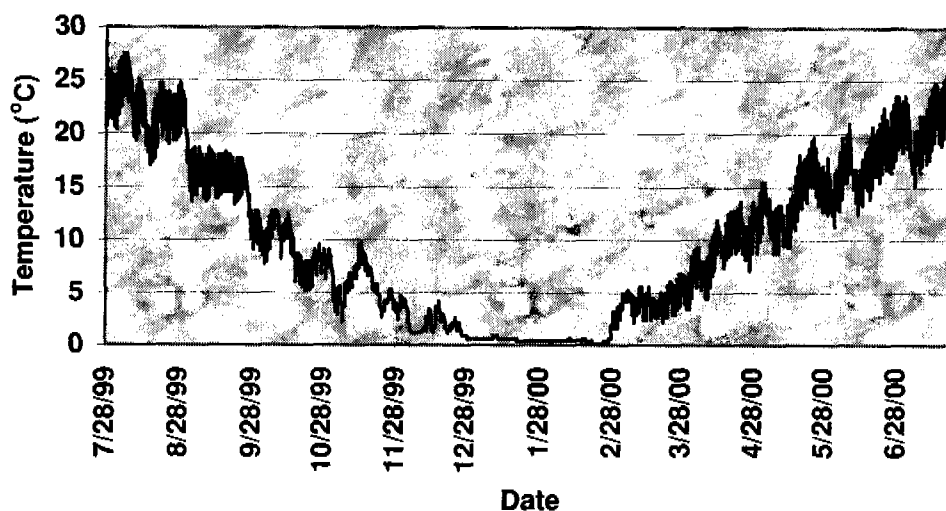
Figure 7.32.1.—Soil temperature signature for the 10-cm depth at site 1.
