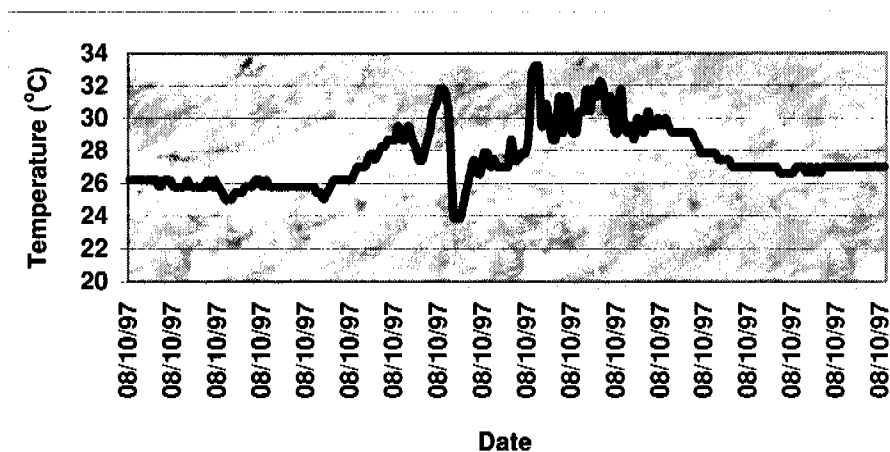
Figure 7.24.2.—The air temperature in the study area on August 10, 1997.
