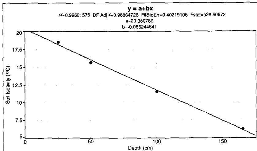
Figure 7.23.3.—The reduction in soil isotivity (°C) with depth at site 1.
