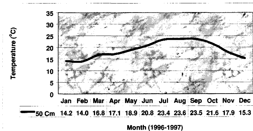
Figure 5.4.—A thermic temperature regime in a soil on Edisto Island, South Carolina.
