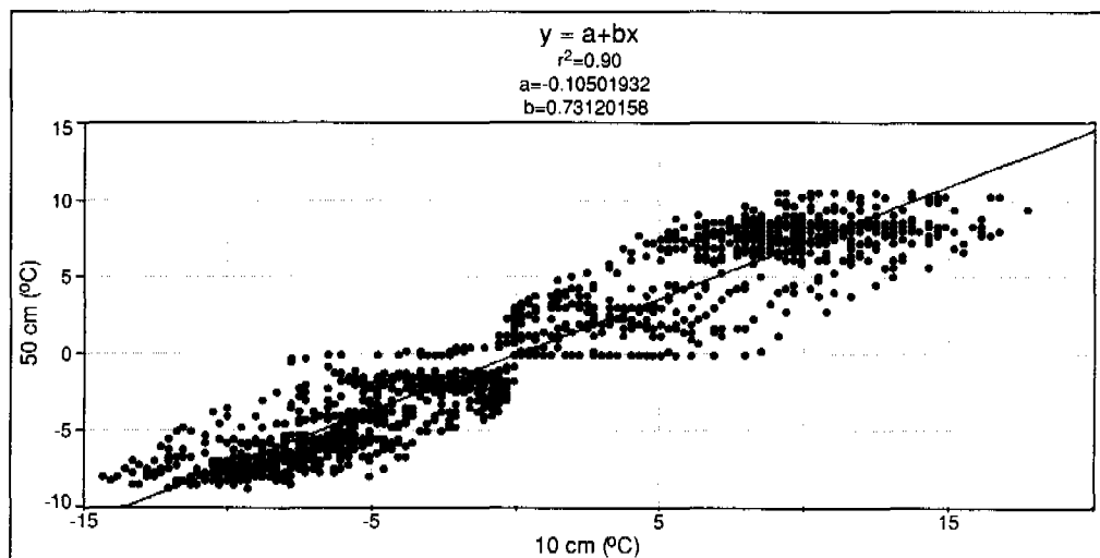
Figure 7.05.5.—Correlation of soil temperatures at 10 cm and 50 cm for site 2.
