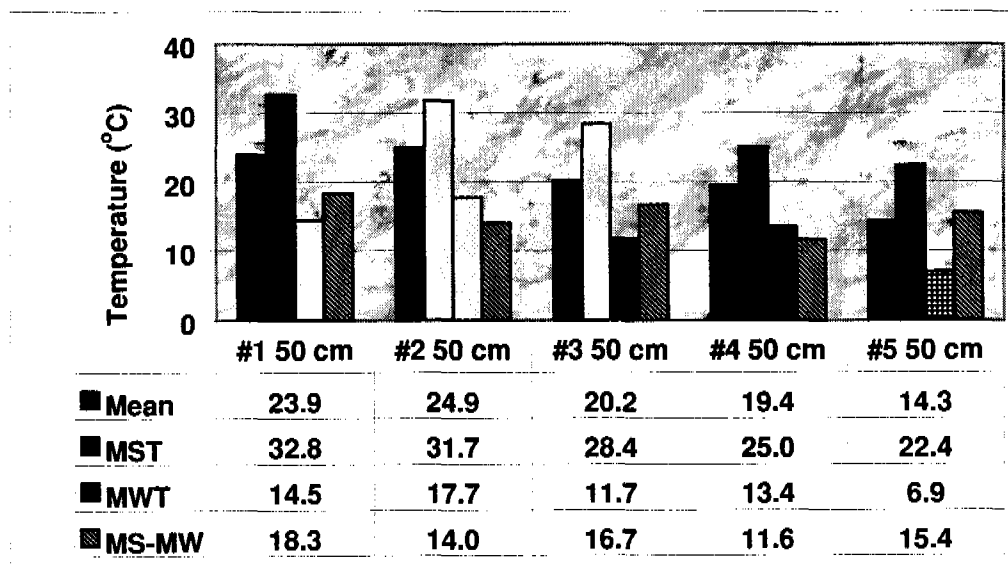
Figure 7.04.4.—Seasonal and annual soil temperature averages for the 50-cm depth.
