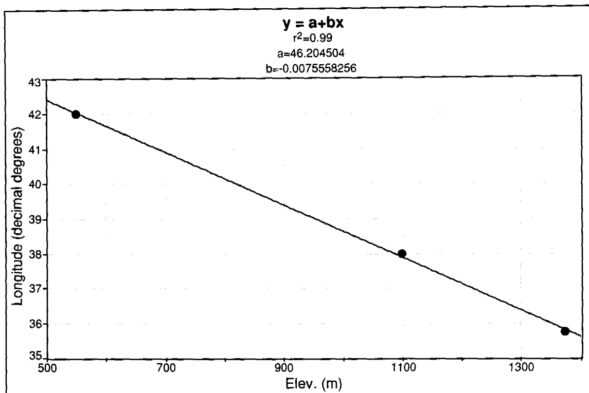
Figure 7.33.3.—Regression equation used to differentiate mesic and frigid soils in MLRA Region 13.
