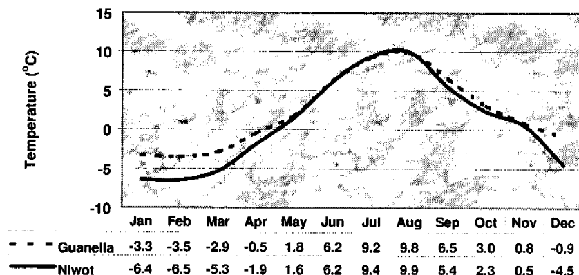
Figure 7.06.4.—Average monthly temperatures for site 3 in Guanella Pass and site 2 on Niwot Ridge.
