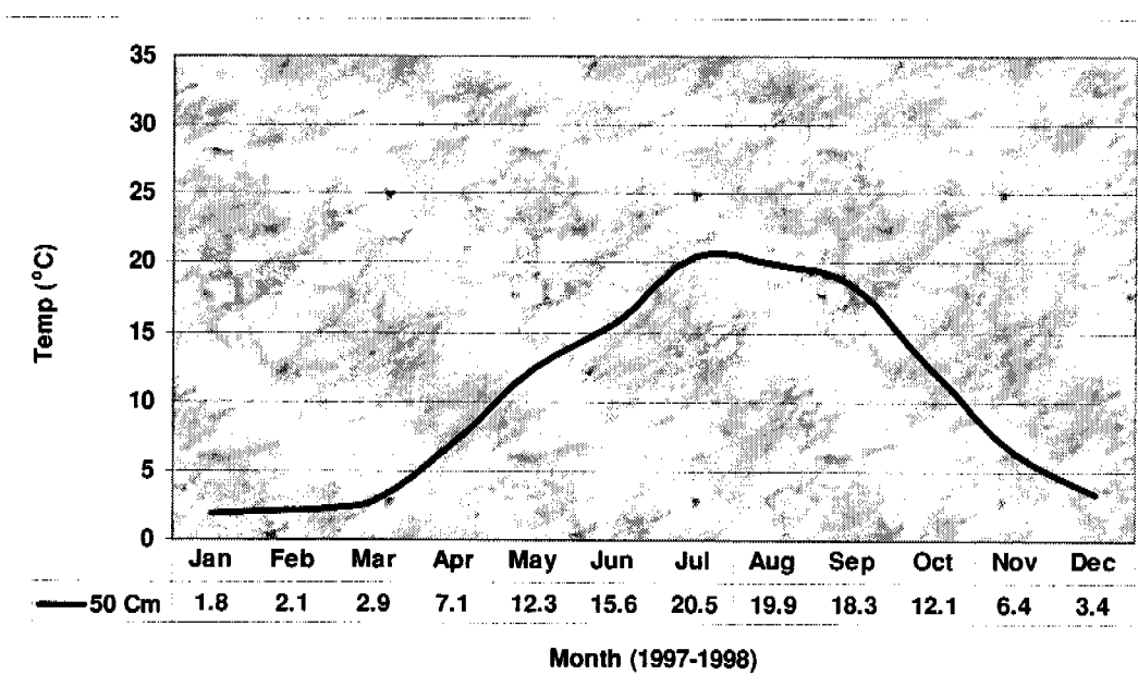
Figure 5.3.—A mesic temperature regime in a soil in the Sand Hills of Nebraska.
