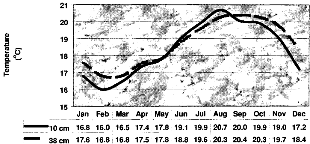
Figure 7.09.3.—Monthly soil temperature averages for the KDC 1 site.
