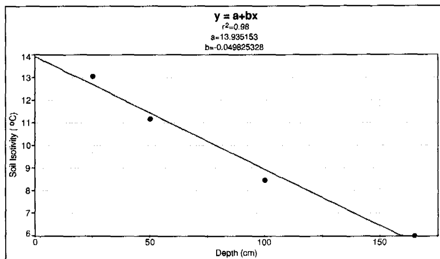
Figure 7.23.4.—The reduction in soil isotivity (°C) with depth at site 2.
