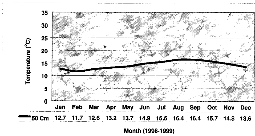
Figure 5.7.—Isomesic temperature signature of a soil on the Big Island of Hawaii.
