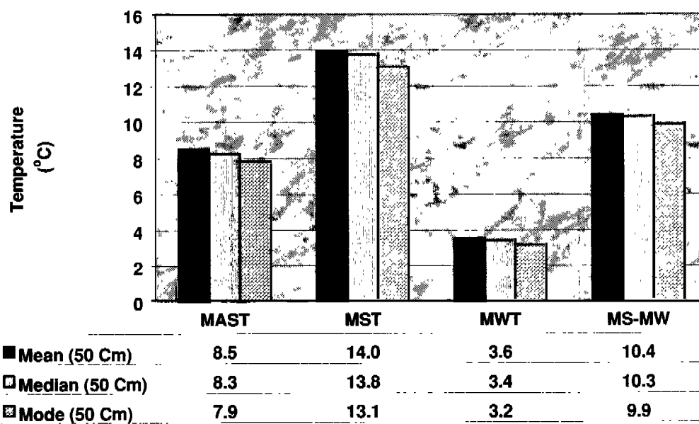
Figure 4.4.—The annual mean, median, and mode for a site in West Virginia.
