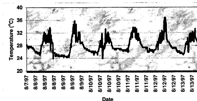
Figure 7.24.1.—Air temperature signature for the 6-day study on Vieques Island.
