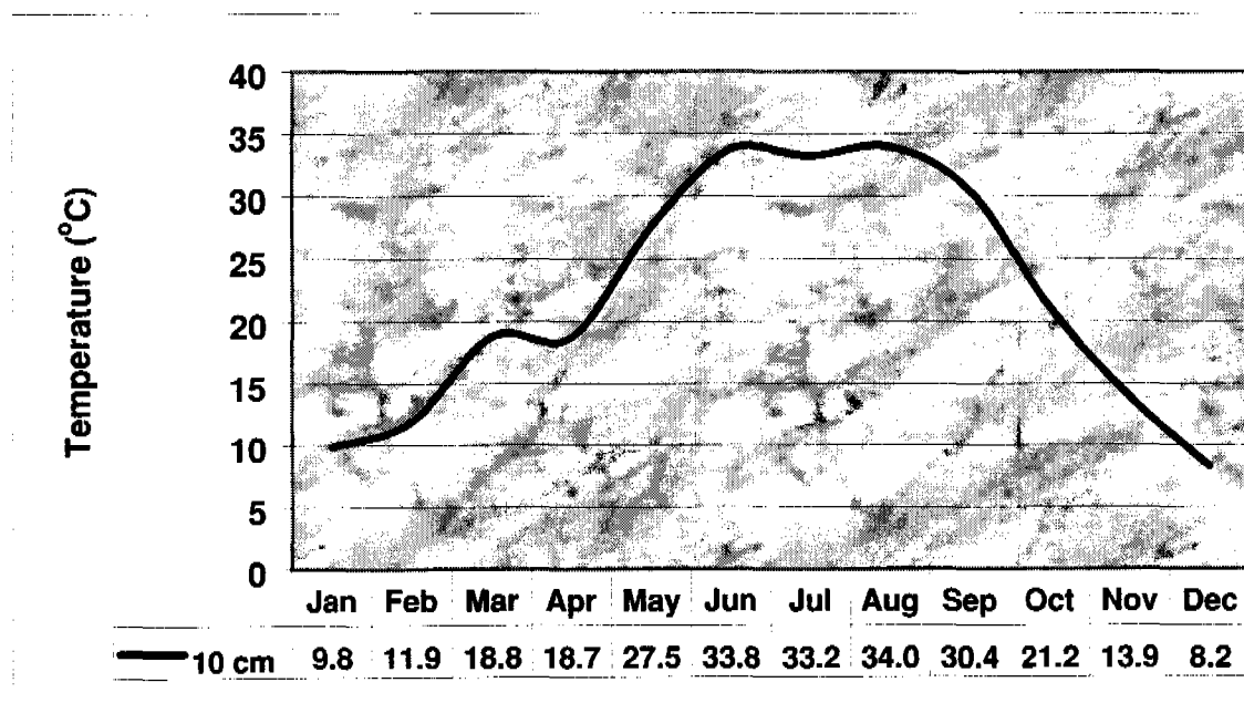
Figure 7.02.1.—Average monthly soil temperature for the 10-cm depth at site 5.
