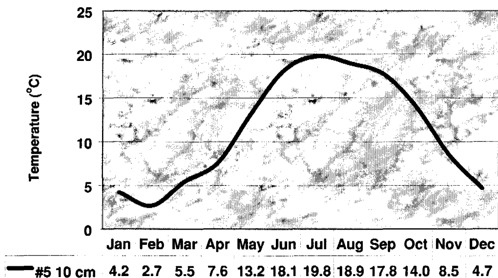
Figure 7.01.5.—Average monthly soil temperature for the 10-cm depth at site 5.
