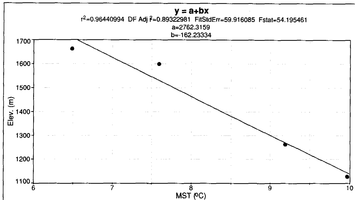
Figure 7.11.2.—Regression of elevation and mean summer soil temperature.
