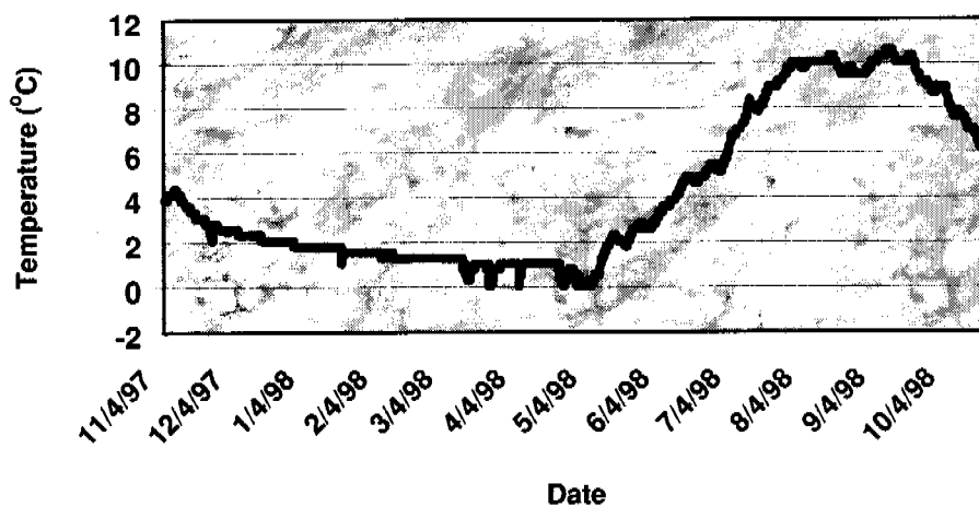
Figure 7.12.5.—Soil temperature signature at 50 cm for site 10 during the first year.
