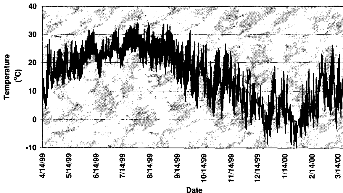
Figure 7.14.3. —Air temperature signature at the Horseshoe Lake Wildlife Area.
