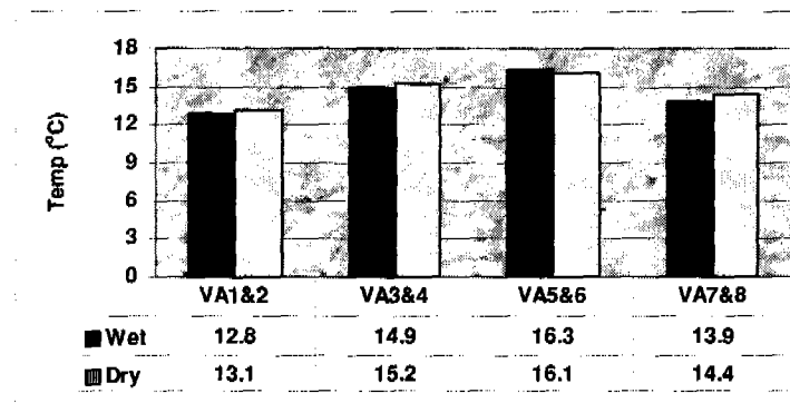
Figure 7.30.2.—Relationship of MAST for the poorly drained (wet) and well drained (dry) soils in Virginia.
