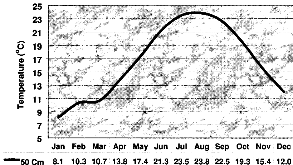
Figure 7.03.1.—Average monthly soil temperatures at a depth of 50 cm.
