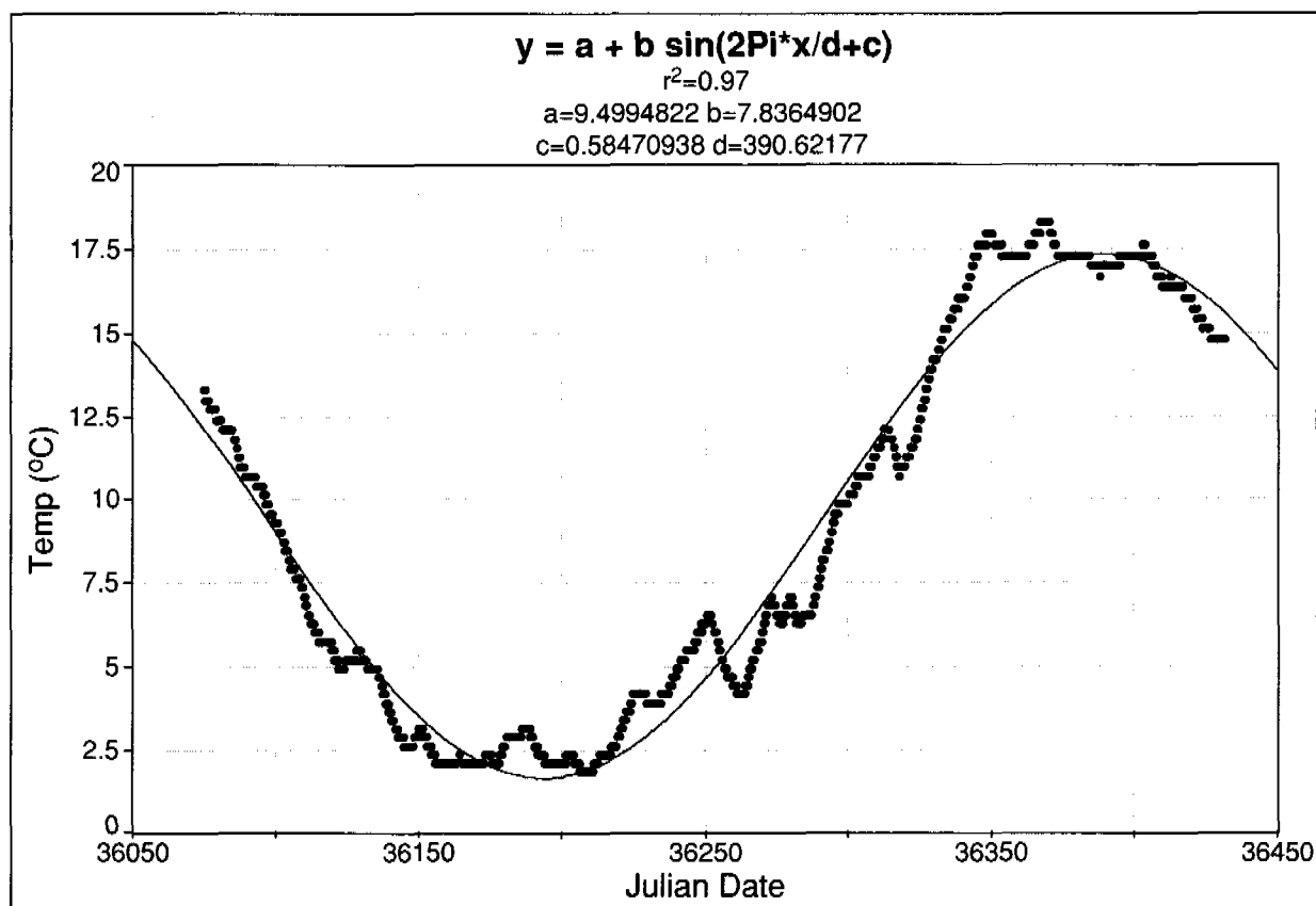
Figure 7.02.4.—Sine wave nature of the temperature signature at 50 cm for site 3.
