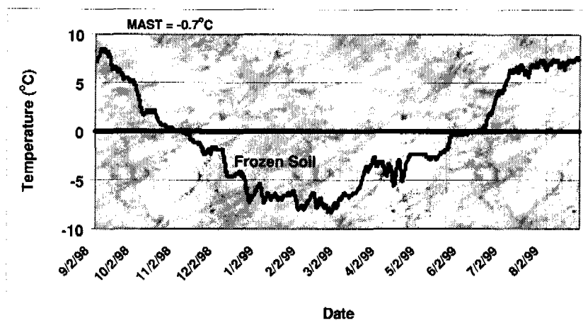
Figure 7.05.1.—Soil temperature signature for the 50-cm depth at site 3. This is a very cold soil with more than 7 continuous months below freezing.
