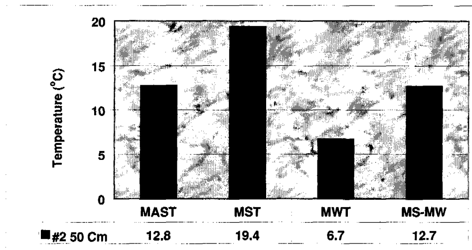
Figure 7.21.1.—Summarized temperature data for the wet spring seep at site 2.
