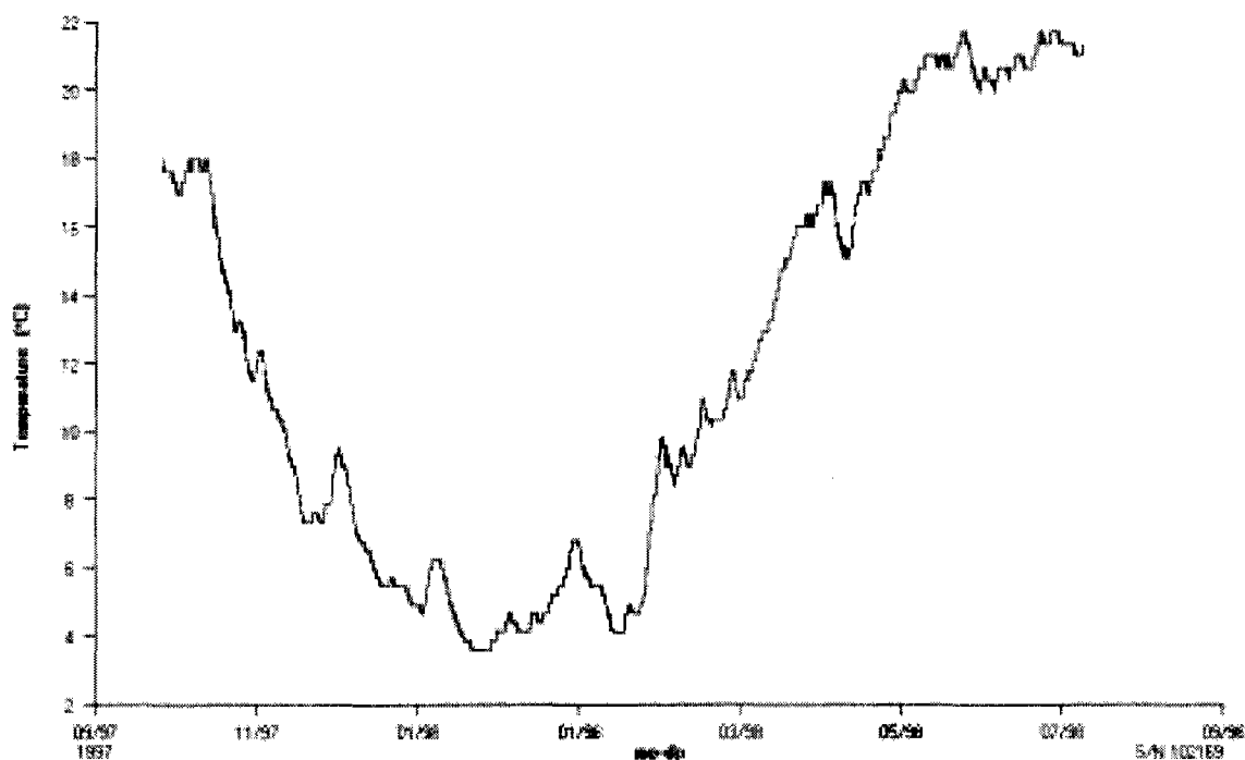
Figure 6.2.—Data are off-loaded into OnSet “dtf” files before being exported to Excel format. This example is from a soil in central Missouri.
