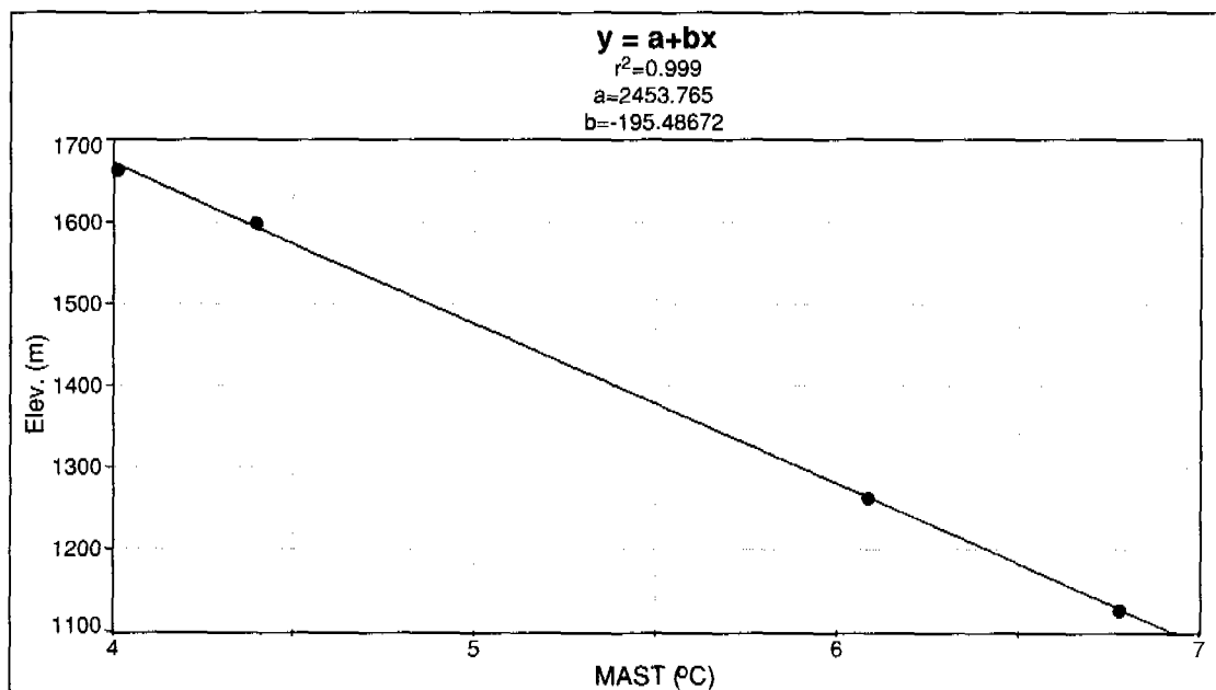
Figure 7.11.1.—Regression of elevation and mean annual soil temperature.
