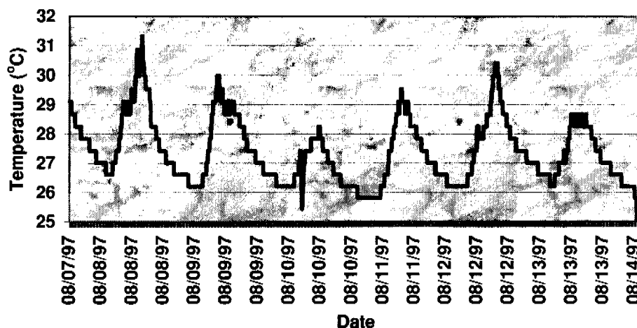
Figure 7.24.3.—Soil temperature signature at 2.5 cm for the 6-day study.
