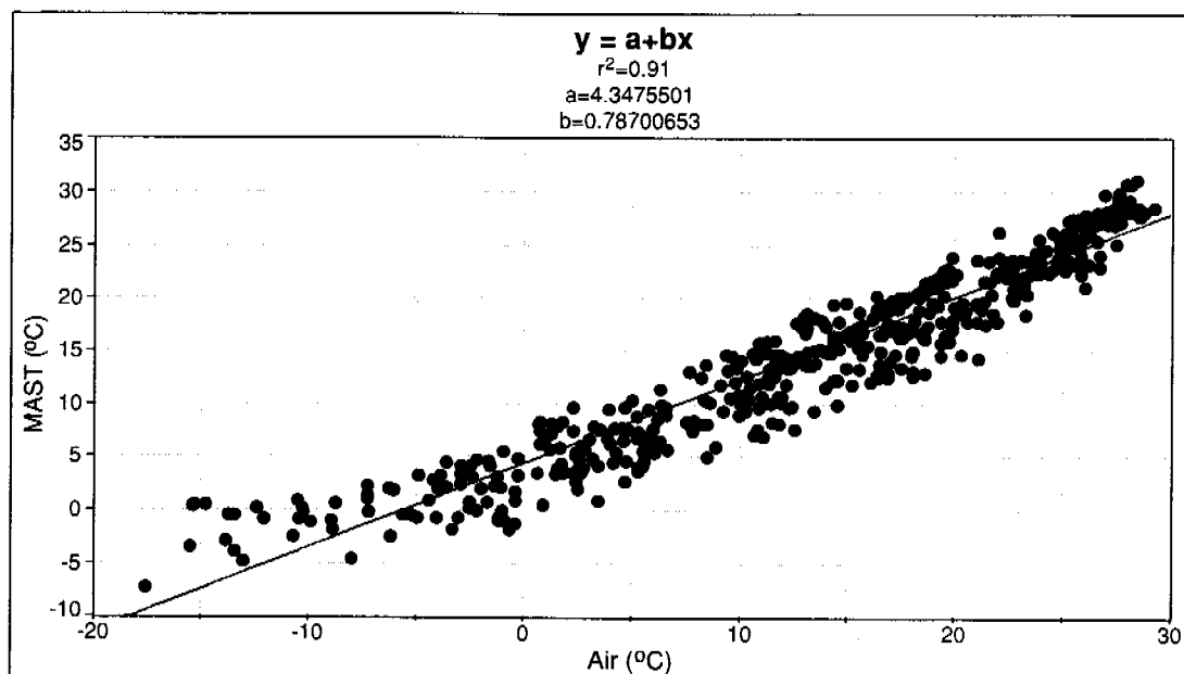
Figure 7.14.10.—Regression (autocorrelation) of air and soil temperatures from 100 sites in the U.S.
