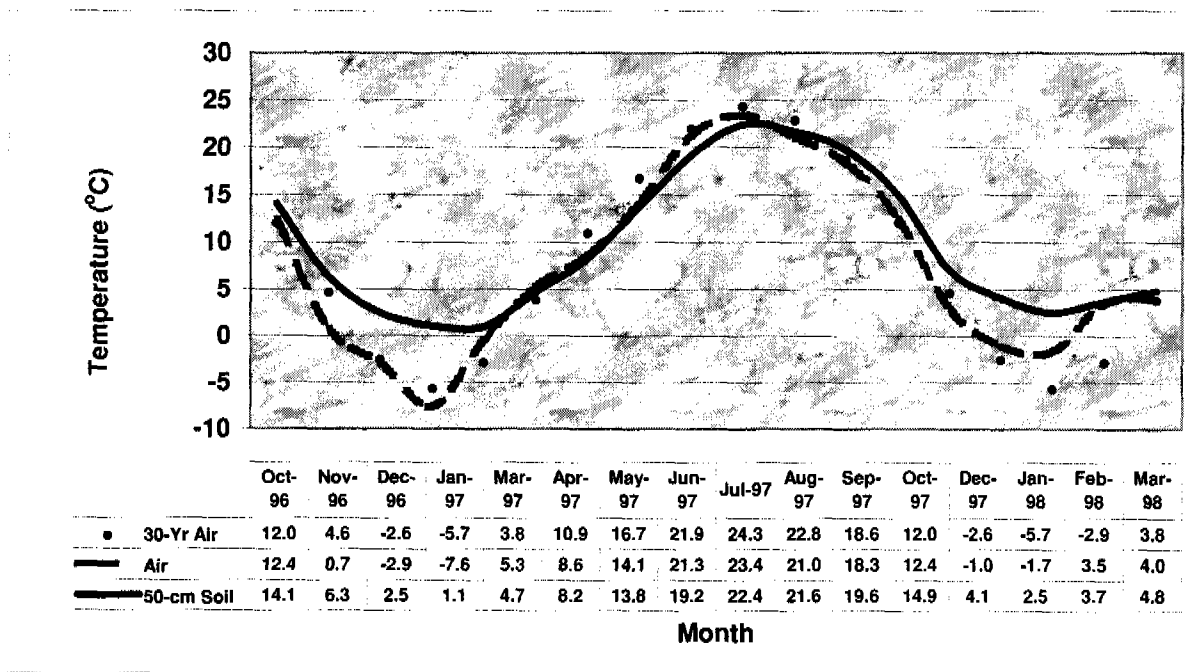
Figure 4.8.—Short-term data used to effect shift analysis.
