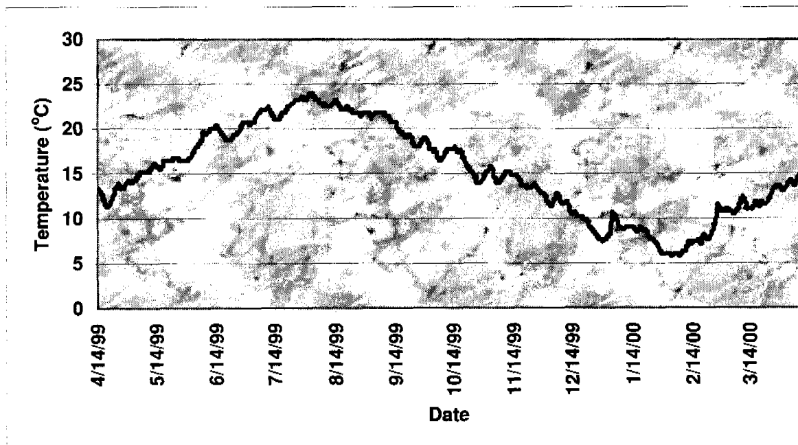
Figure 7.14.4.—The soil temperature signature at 50 cm for site 7.
