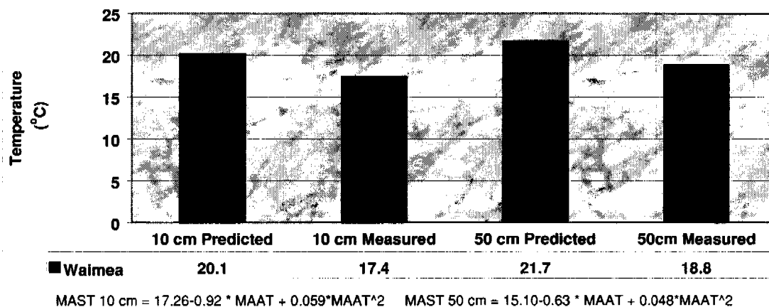
Figure 7.08.5.—Comparison of predicted MAST and measured data from the Parker HQ site near Waimea, Hawaii.
