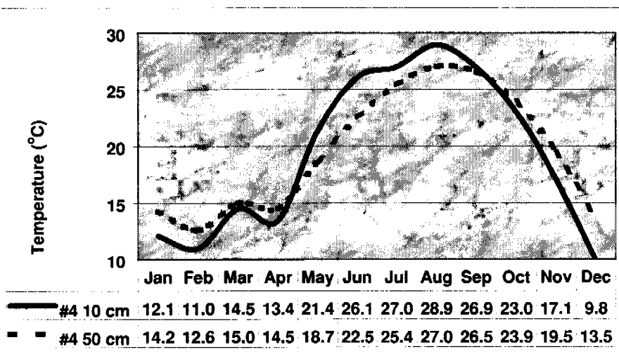
Figure 7.04.2.—Monthly analysis of soil temperature at site 4.
