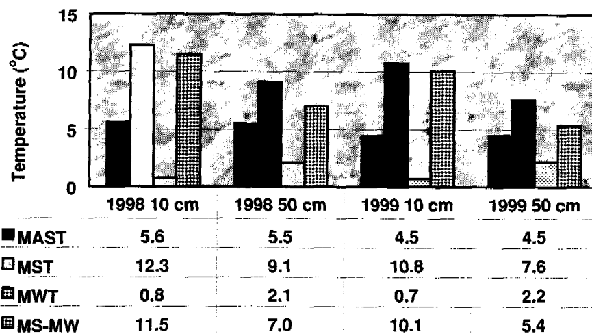
Figure 7.12.4.—Soil temperature relationships at site 8 during the 2-year study.
