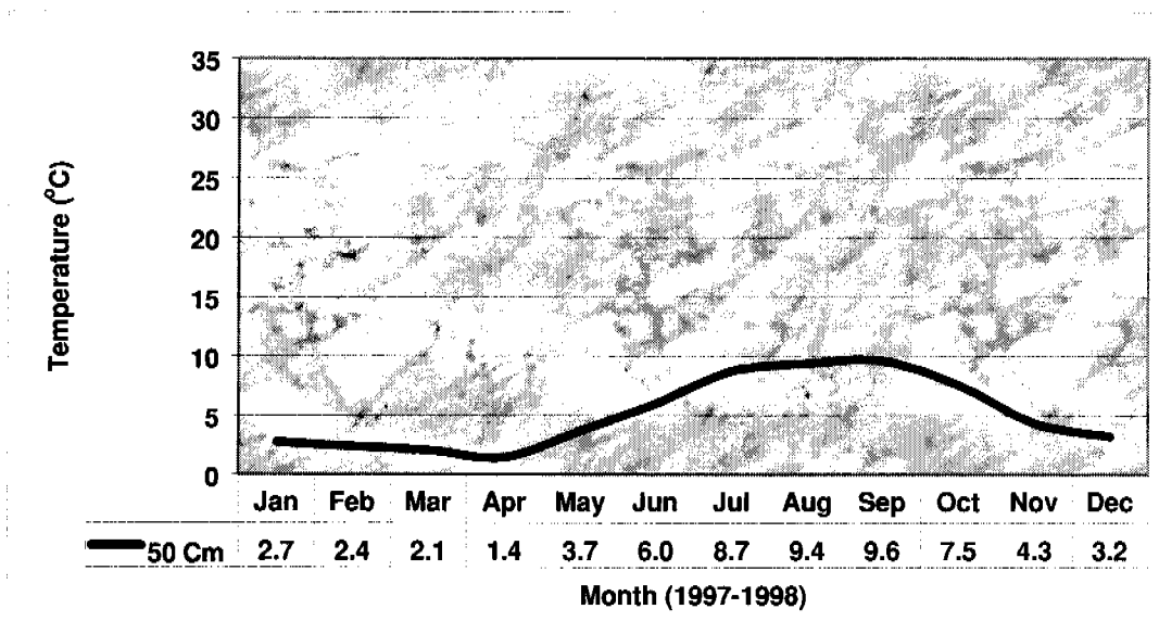
Figure 5.6.—Isofrigid temperature signature in a soil in Clearwater County, Idaho.
