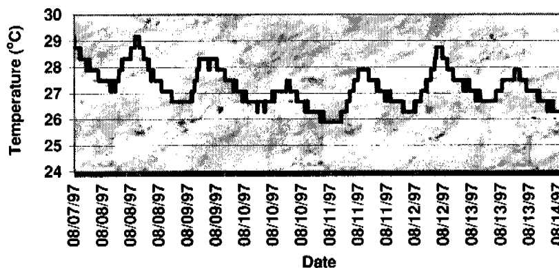
Figure 7.24.4.—Soil temperature signature at 5 cm.
