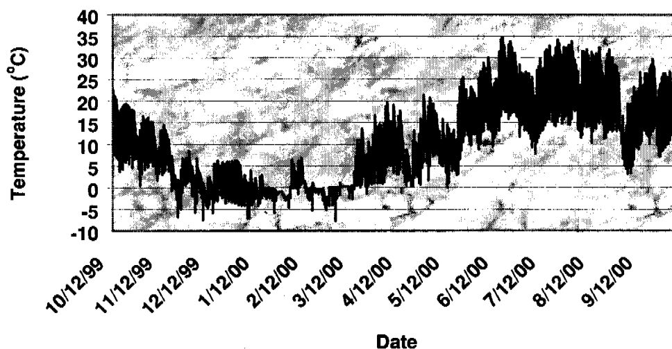
Figure 7.17.2.—The 10-cm soil temperature signature at site 3 showed extreme diurnal fluctuation during July.
