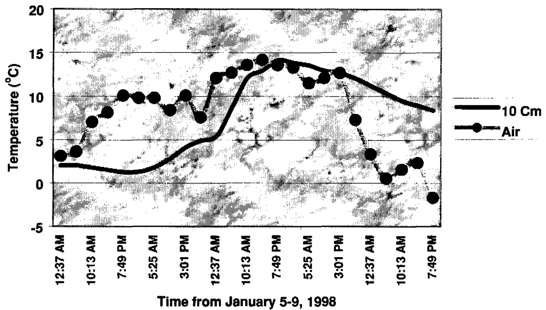
Figure 3.5.—Same data from figure 3.4 examined in closer detail. The period from January 5-9, 1998, looks valid after scrutiny of the air and soil temperature data. This is a winter thaw phenomenon.
