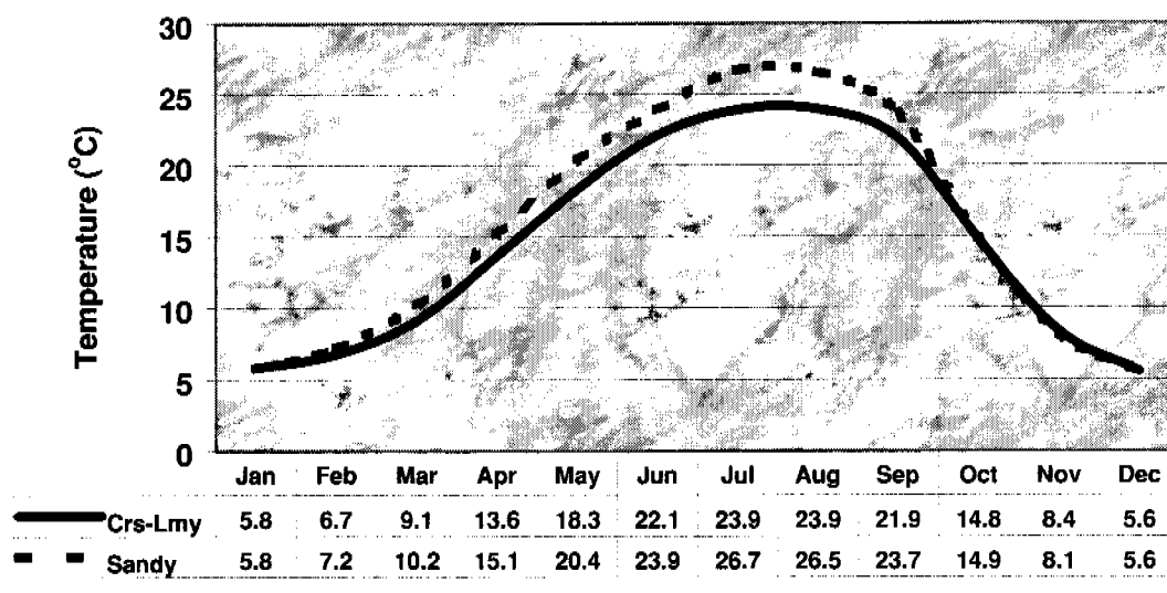
Figure 7.29.1.—Monthly temperature signature at 50 cm showing warmer averages for the sandy sites.
