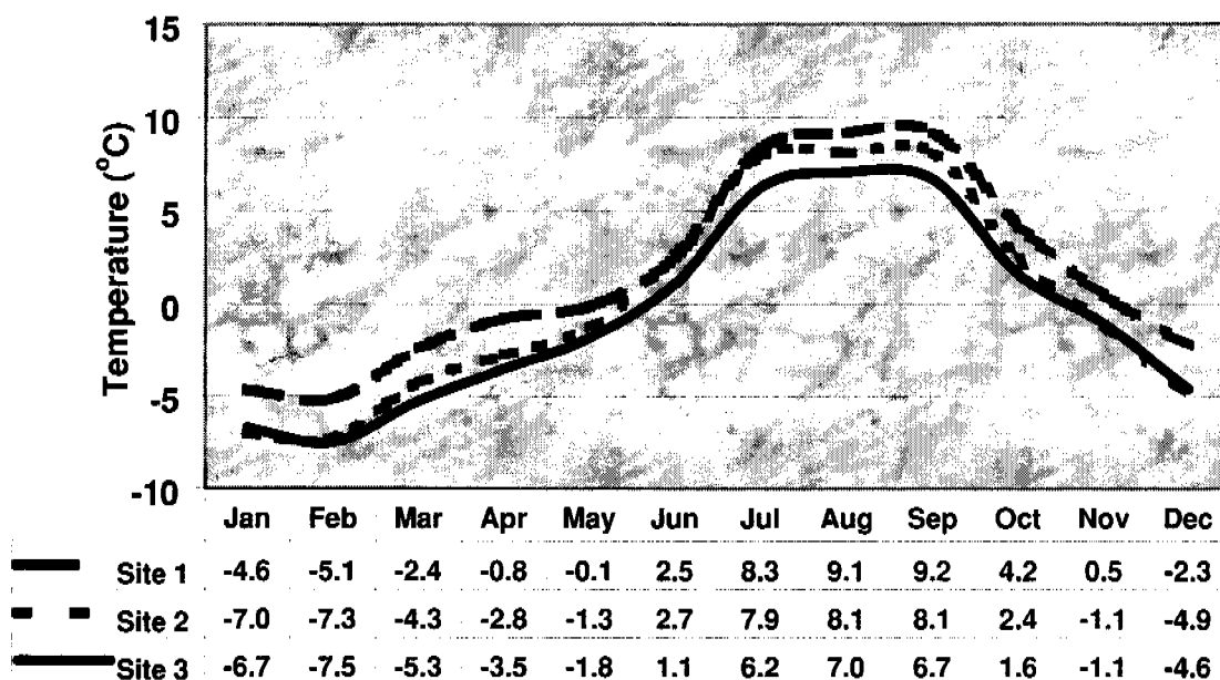
Figure 7.05.2.—Average monthly soil temperatures for the Niwot Ridge study area.
