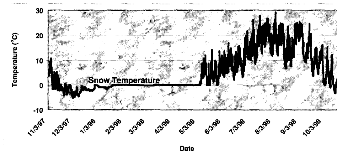
Figure 7.11.3.—Air temperature signature for Idaho site 4.
