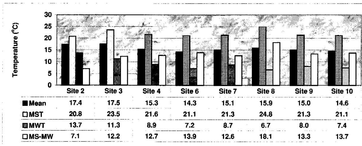
Figure 7.14.9.—Average seasonal and annual soil temperatures for the 50-cm soil depth.
