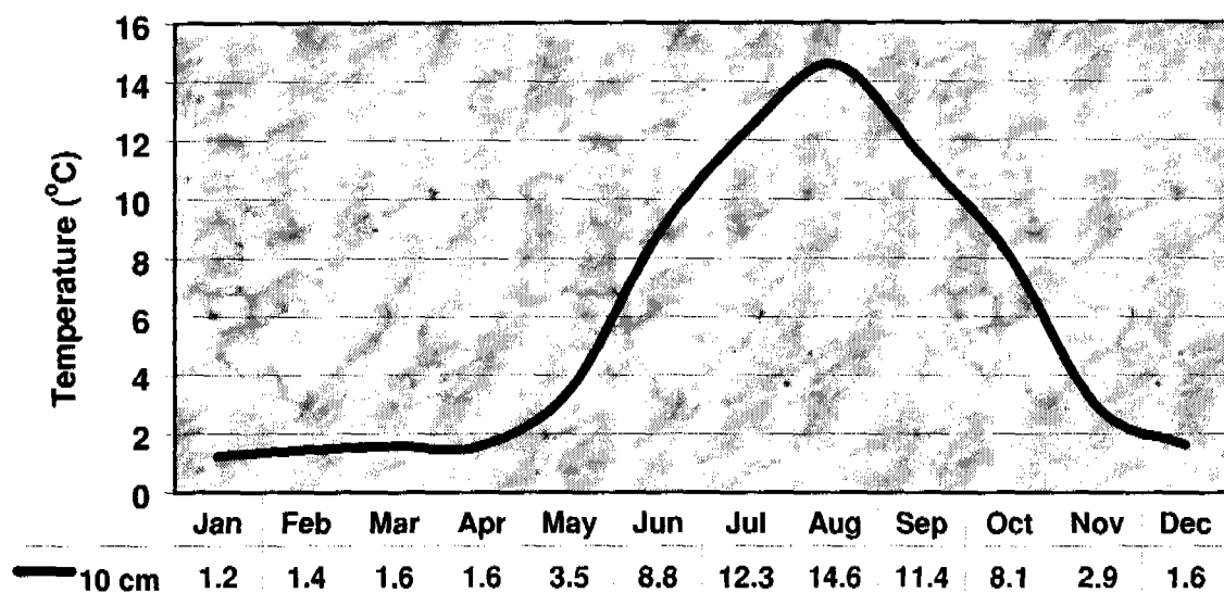
Figure 7.12.3.—Monthly soil temperature averages at 10 cm for site 7 during the second year of the study.
