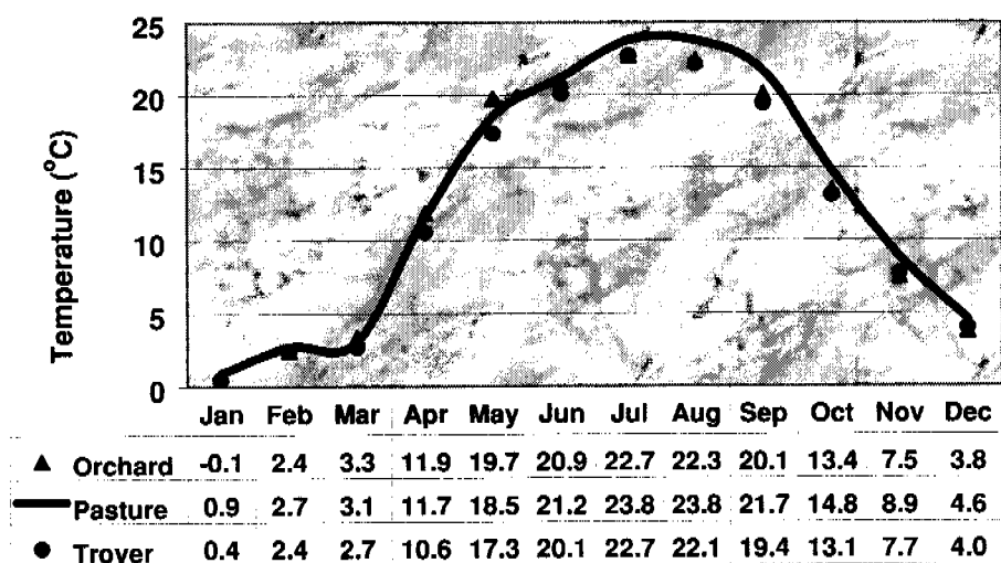
Figure 7.13.2.—Average monthly soil temperatures for the 10-cm depth in the study area.
