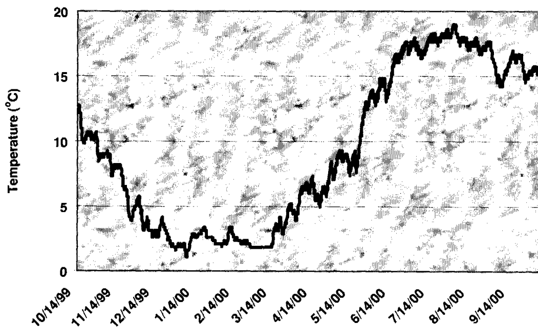
Figure 7.17.5.—Soil temperature signature for the 48-cm depth at site 10.
