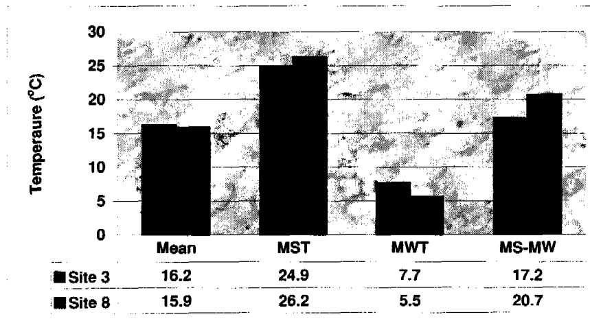
Figure 7.14.8.—Seasonal and annual soil temperatures for sites 3 and 8.
