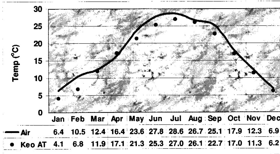
Figure 7.03.3.—Comparison of 1998-1999 air temperature data to the 30-year normal at Keo.
