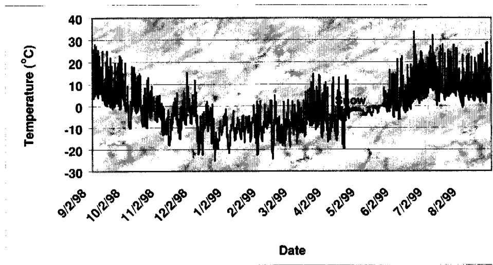
Figure 7.05.3.—Impact of snowfall on the air temperature signature at site 3.
