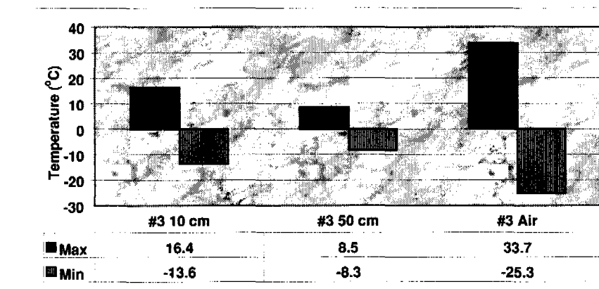
Figure 7.05.6.—Maximum and minimum extremes for air and soil temperatures at site 3.
