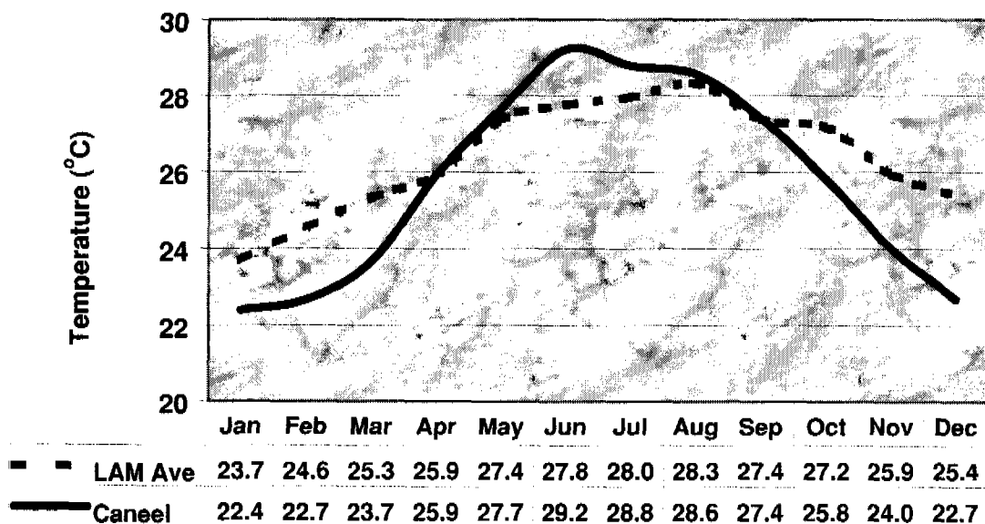
Figure 7.28.2.—Monthly air temperature values for the average of the Lameshur Bay sites and for the Caneel Hill site.
