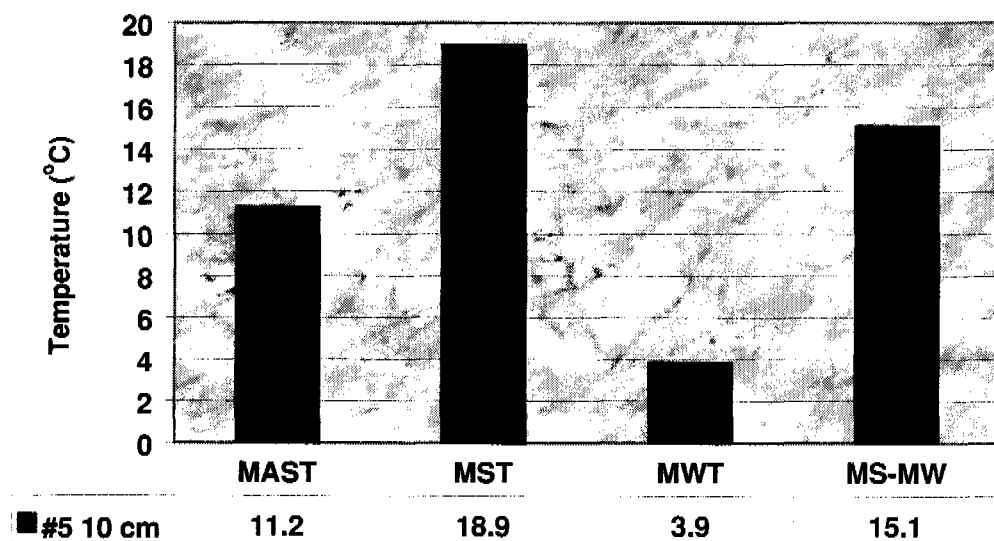
Figure 7.01.6.—Seasonal and annual analysis for the 10-cm depth at site 5.
