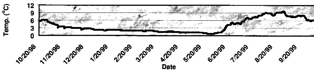
Figure 7.12.2.—Soil temperature signature at 50 cm for site 5.
