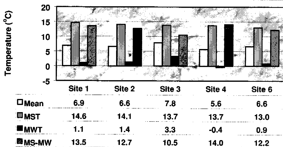
Figure 7.15.6.—Average seasonal and annual soil temperatures at 10 cm for five sites in the study area.
