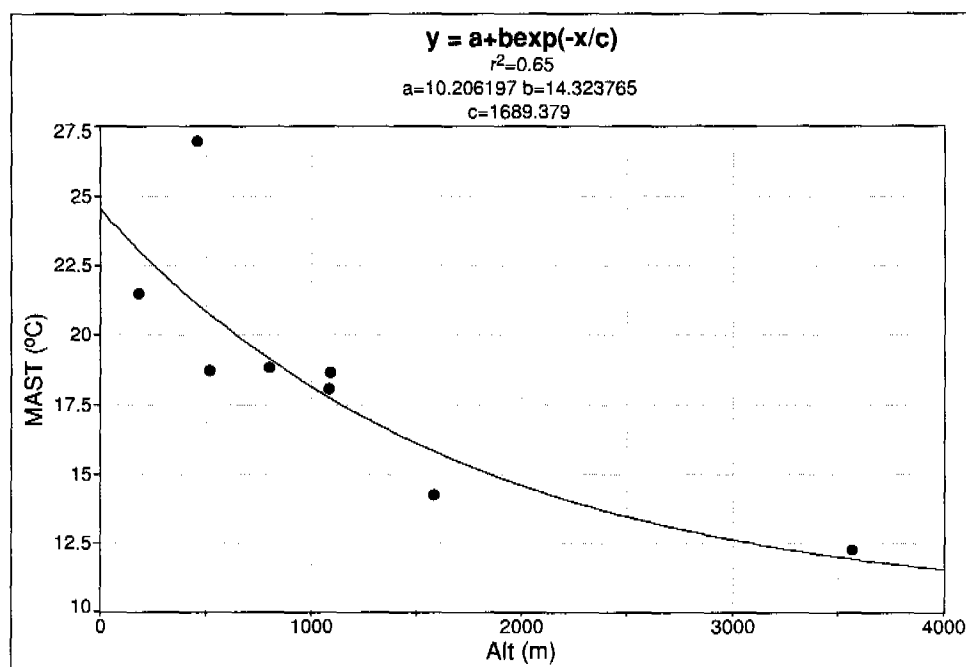
Figure 4.5.—Regression equation for nine sites on the Big Island of Hawaii.
