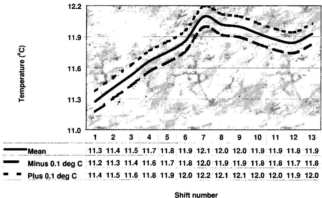
Figure 7.20.1.—Shift analysis for the 50-cm soil depth at New York City site 1.
