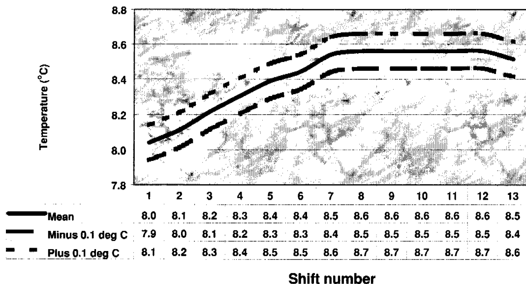
Figure 7.19.1.—Modeled shift of the MAST at 50 cm from July 1998 through July 1999 at site 1.
