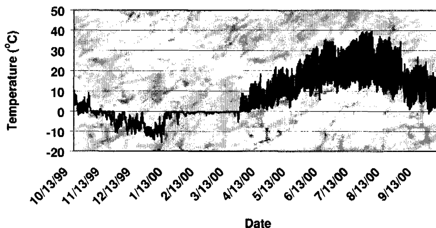
Figure 7.17.4.—Soil temperature signature for 10 cm at site 8 showing extreme highs and lows.
