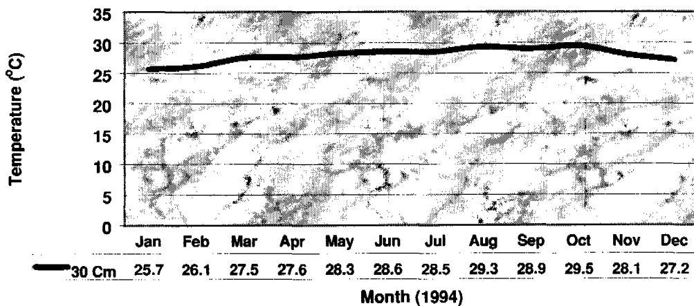
Figure 5.9.—Isohyperthermic temperature signature of a soil on St. John Island, Virgin Islands.
