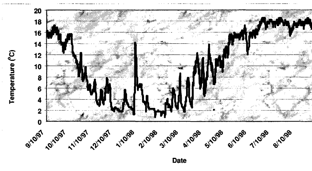
Figure 3.4.—A troublesome spike at the 10-cm soil depth on a site in the Great Smoky Mountains of Tennessee.
