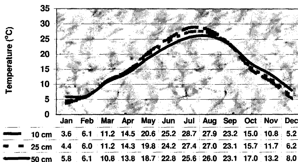
Figure 7.14.5.—Monthly soil temperatures at Bellrose Waterfowl Reserve.
