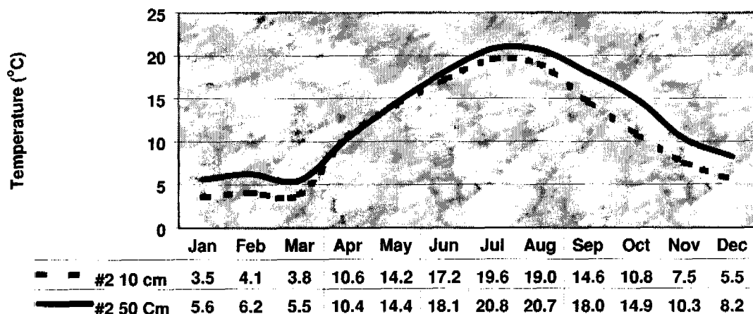
Figure 7.21.2.—Relationship of soil temperature between 10 cm and 50 cm at site 2.
