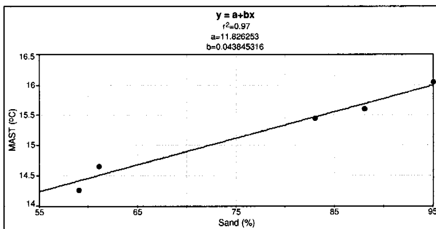
Figure 7.29.4.—Regression of sand content to the MAST at 50 cm.
