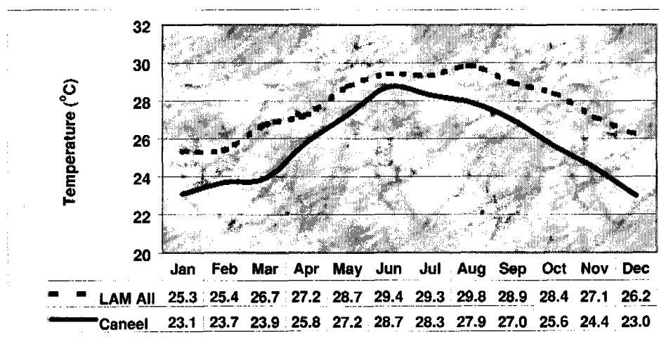
Figure 7.28.3.—Average monthly soil temperatures at 20 cm for Lameshur Bay and Caneel Hill.
