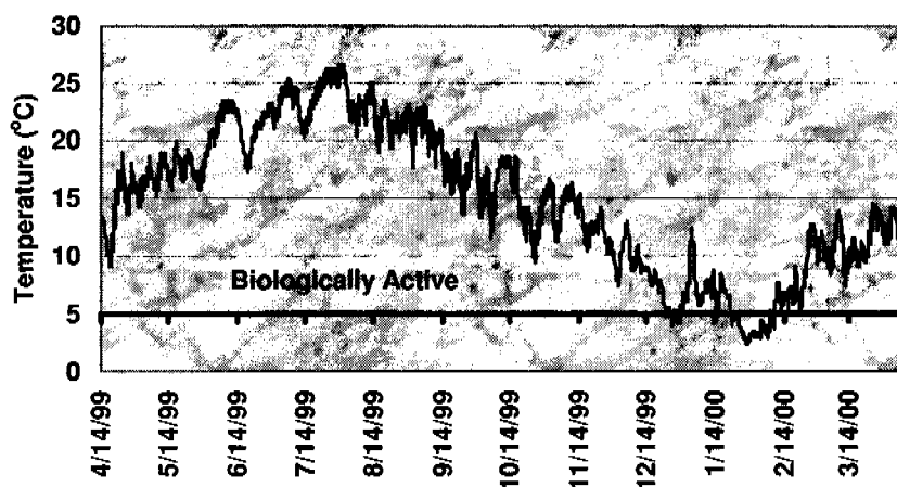
Figure 7.14.2.—Temperature data for the 10-cm soil depth at site 4.
