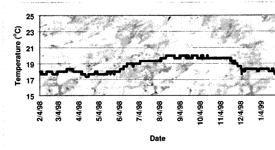
Figure 7.10.2.—Soil temperature signature at 50 cm for the rain forest site at Hamakua.
