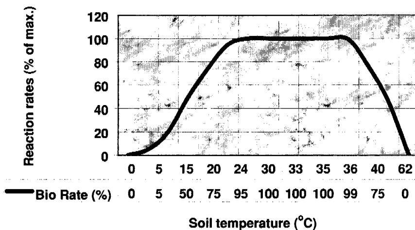
Figure 7.29.2.—Conceptual model for biological activity rates (Paul and Clark, 1989).
