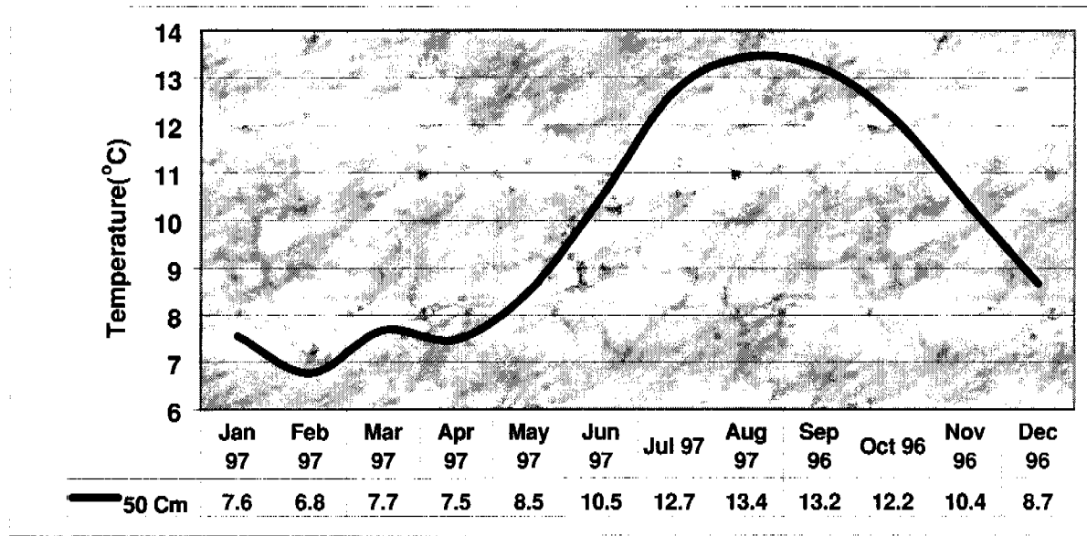
Figure 7.26.2.—Average monthly soil temperatures for the isomesic soil at site 4.
