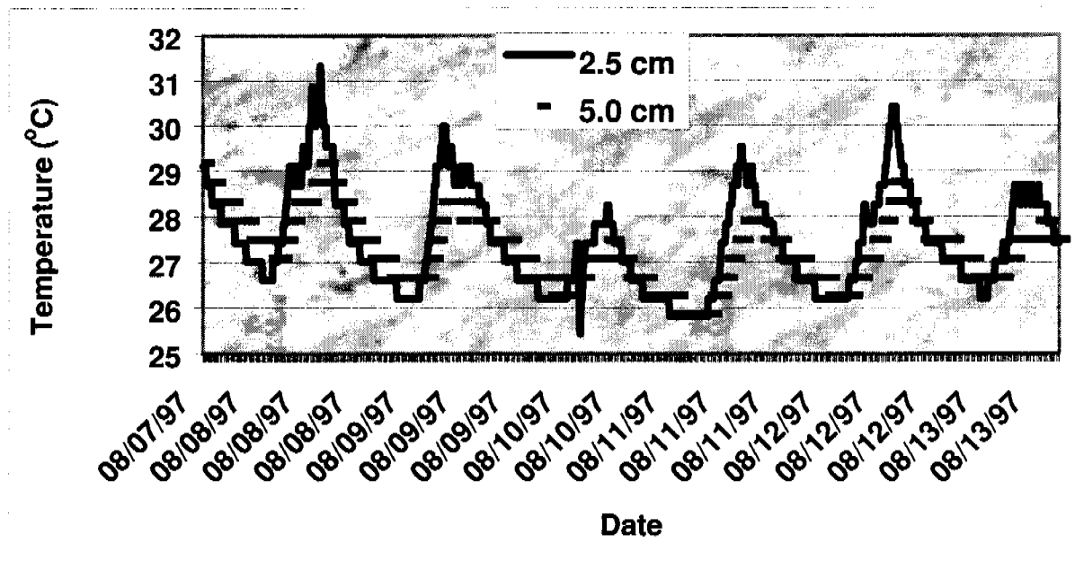
Figure 7.24.5.—Relationship of the soil temperature signatures at 2.5 cm and 5 cm.
