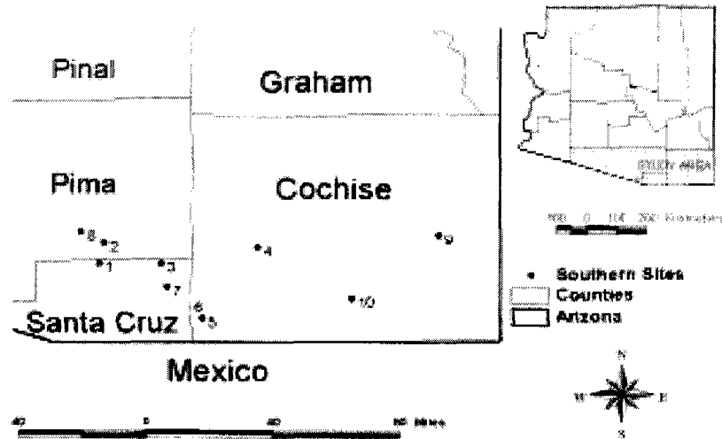
Figure 7.01.1.—Location of temperature sites in the study area.
