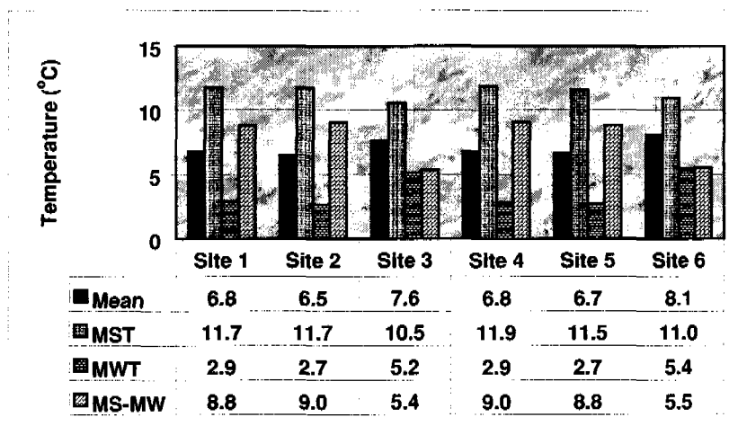
Figure 7.15.7.—Average seasonal and annual soil temperatures for the 50-cm depth.
