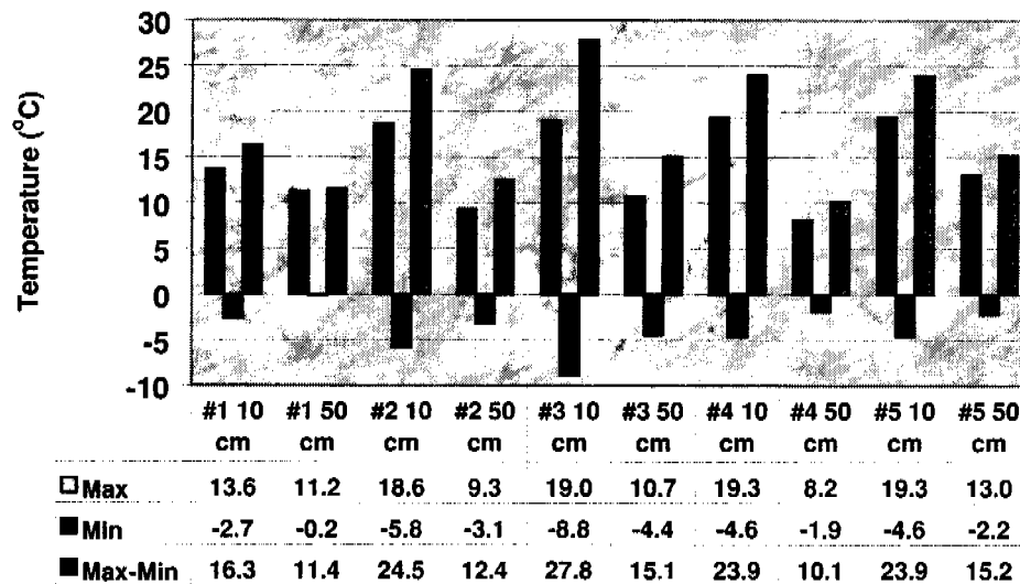
Figure 7.06.3.—Maximum and minimum soil temperature extremes at 10 cm and 50 cm.
