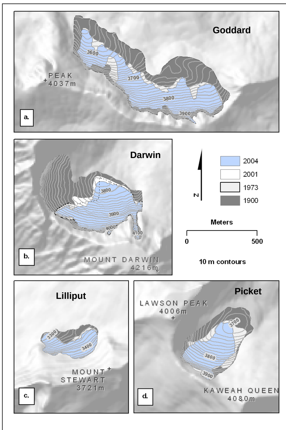
Appendix E2. Individual glacier chronology maps for (a) Goddard Glacier, (b) Darwin Glacier, (c) Lilliput Glacier, and (d) Pickett Glacier. The 1973 boundary of Darwin Glacier is dashed where the glacier was smaller than the recent extents.
