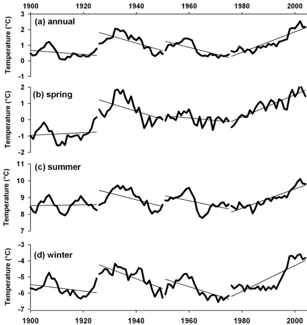
Figure 19. Linear trend lines for 25-year time periods for (a) annual, (b) spring, (c) summer, and (d) winter mean temperatures. Trends are based on 5-year running means.
