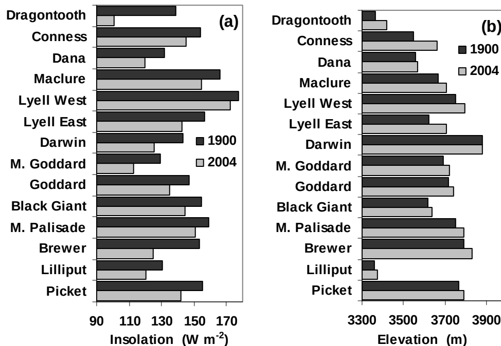
Figure 27. Mean (a) annual clear sky insolation ( \text{W m}^{-2} ) and (b) mean elevation (m) calculated at 14 glaciers for the 1900 and 2004 glacier areas.
