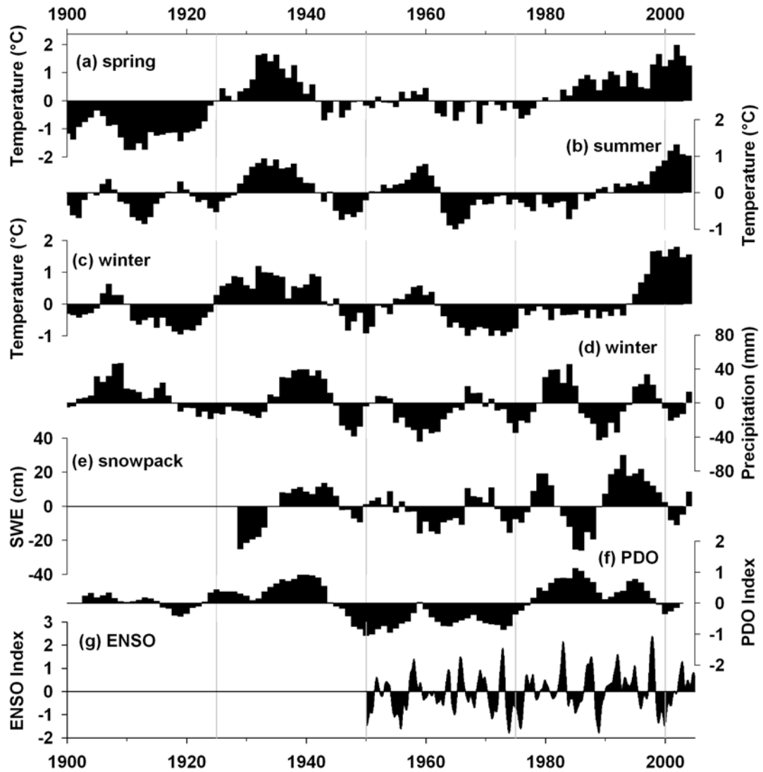
Figure 22. Climate summary with deviations from the mean monthly temperature for (a) spring, (b) summer, (c) winter; (d) mean monthly winter precipitation, (e) April 1 snowpack, (f) PDO for the past century, and (g) monthly ENSO index. All data is smoothed using a 5-year running mean, except for ENSO.
