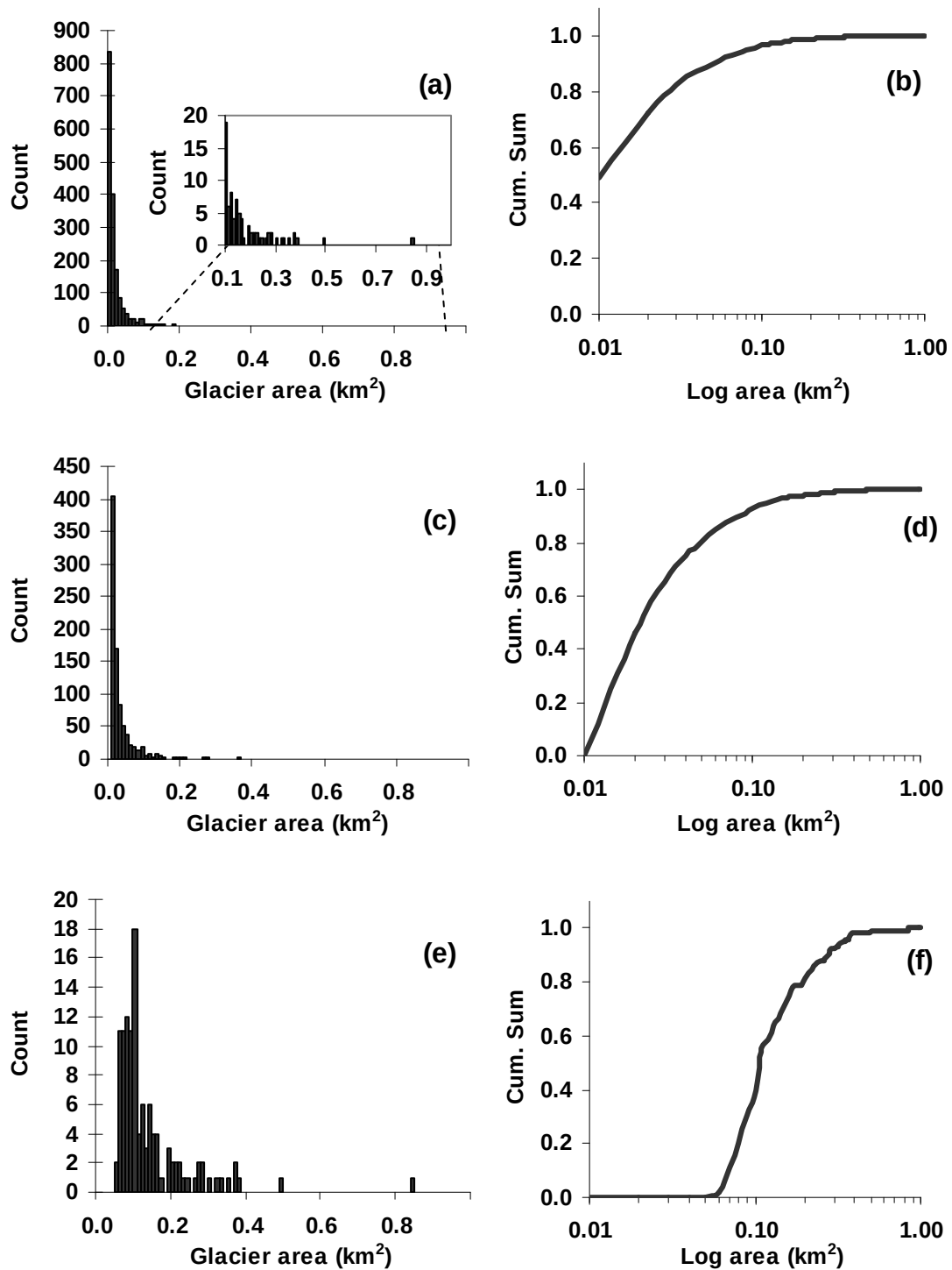
Figure 8. Glacier count (left) and cumulative sum (right) area for all glaciers (a, b), glaciers > 0.01 km 2 (c, d), and glaciers with basal shear stress > 10 5 Pa (e, f). The insert in (a) displays the count of glaciers with area > 0.1 km 2 . Note change in scale for count in a, c, and e.
