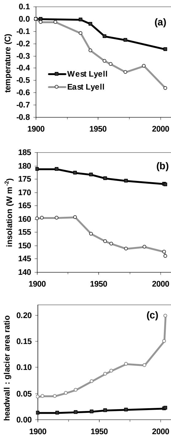
Figure 29. Calculated change in (a) temperature based on environmental lapse rate ( 6.5^{\circ}\text{C km}^{-1} ), (b) potential mean annual insolation, and (c) headwall to glacier area ratio for East and West Lyell Glaciers over the 20 th century.
