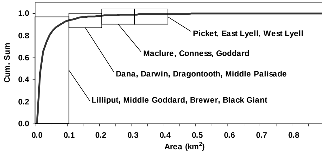
Figure 11. Cumulative sum of glacier population ( >0.01\text{km}^2 ) by area and study glaciers.
