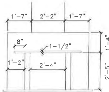
Elevation of fireplace
