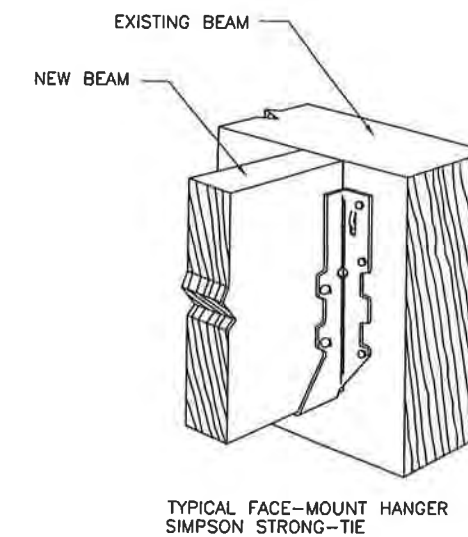
A S2 TYPICAL DETAIL NO SCALE
