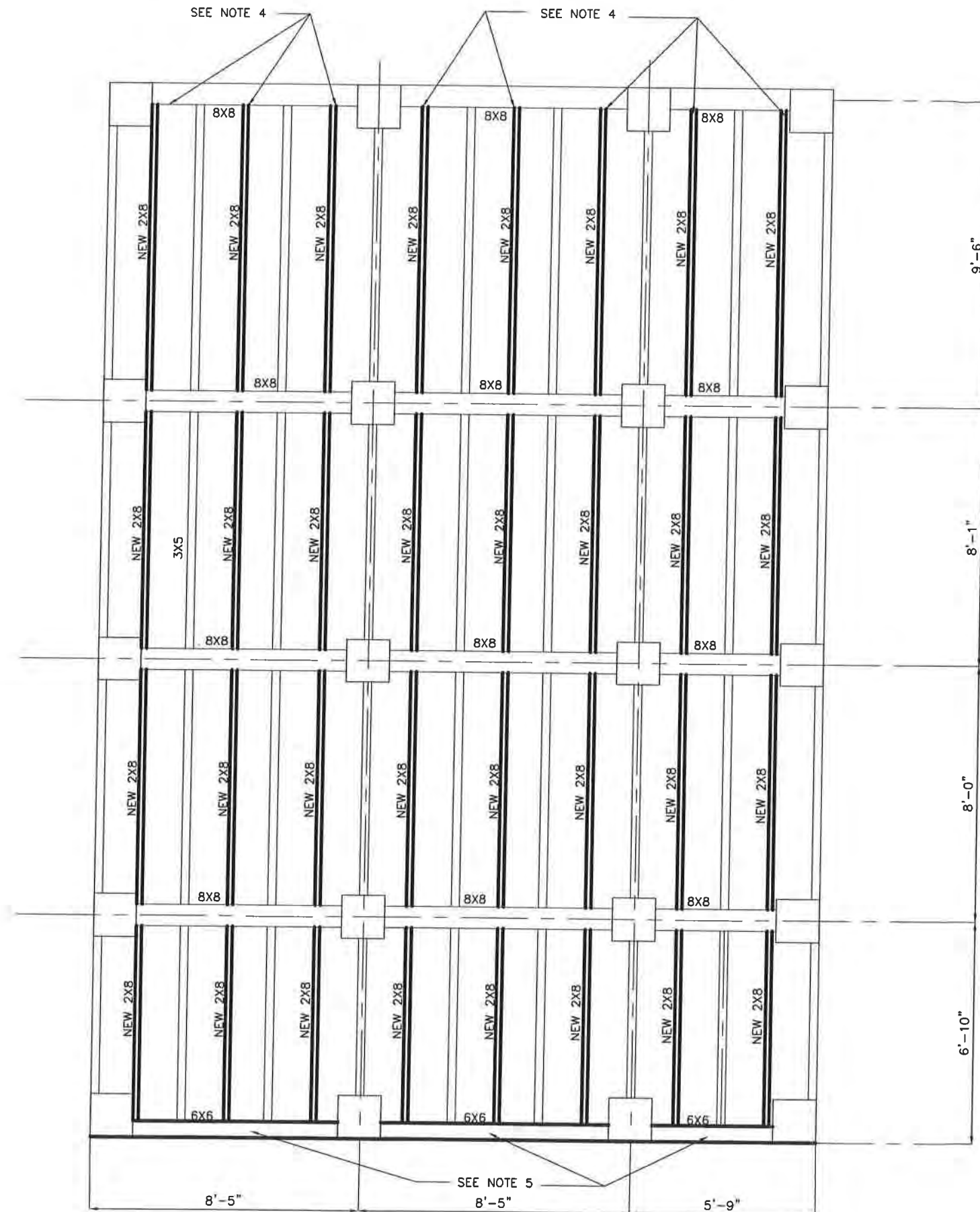
1 S2 FRAMING PLAN MODIFICATIONS
