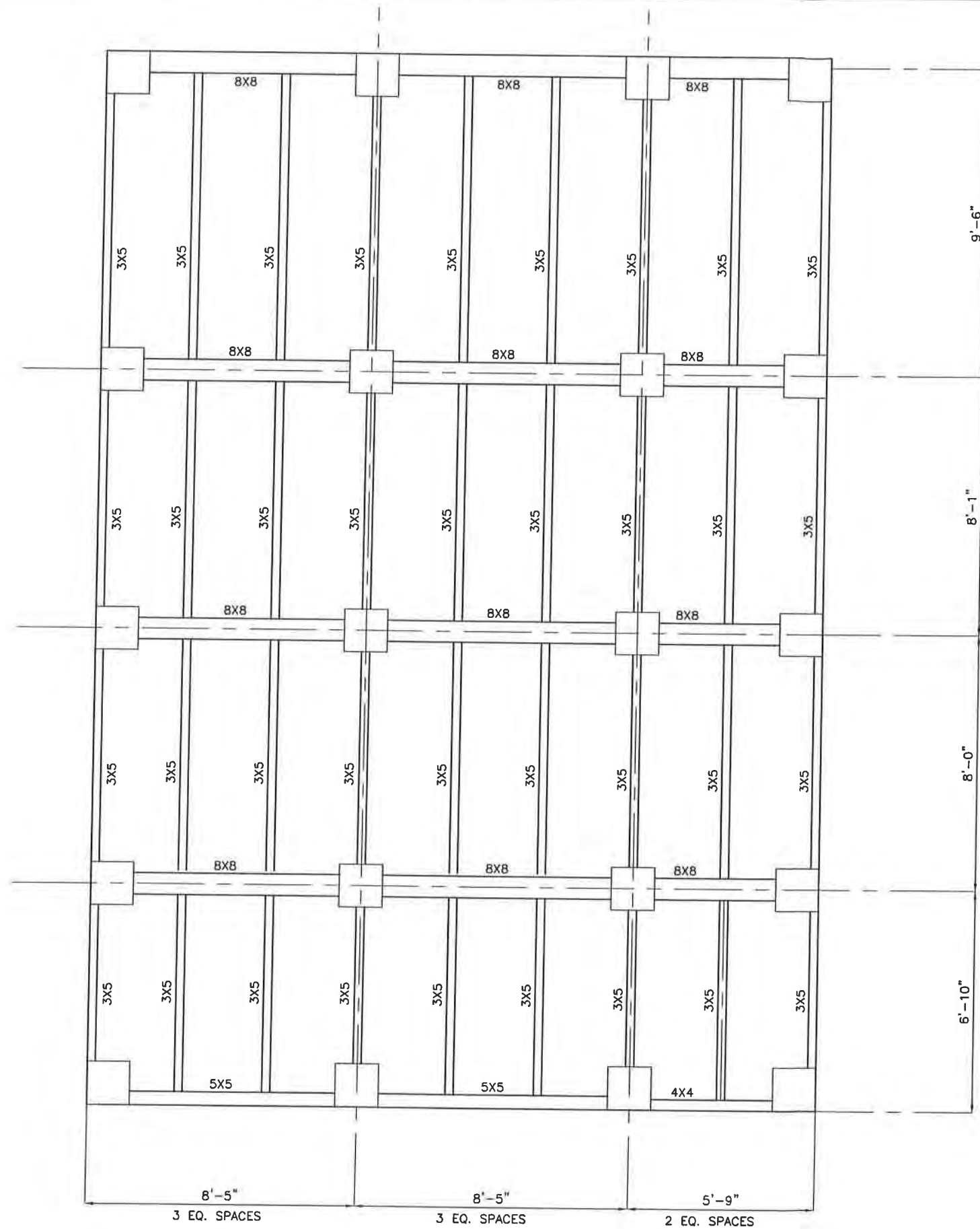
1 S1 EXISTING FRAMING PLAN
