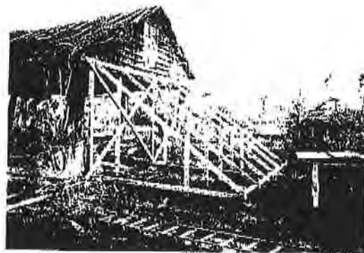
5-1. The Wagon Shed during structural stabilization work. Note diagonal cribbing.
