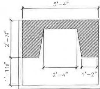
Plan of fireplace
