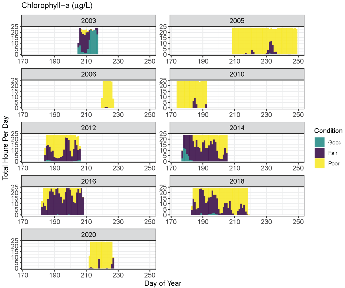
Figure 4-8. Total hours per day that surface chlorophyll-a concentration was observed within each condition category at the Gateway National Recreation Area logging station.
