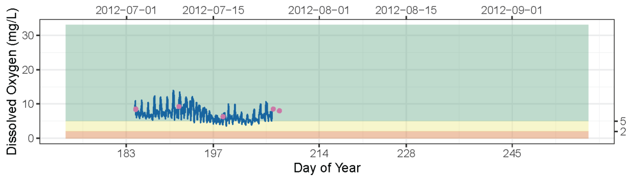
Figure 4-1. Continuous dissolved oxygen readings from sonde deployed at Gateway National Recreation Area logging station in 2012. Magenta points represent discrete grab samples collected every week for quality assurance. Estuarine quality category thresholds (Table 2-1) are delineated by the background color.
