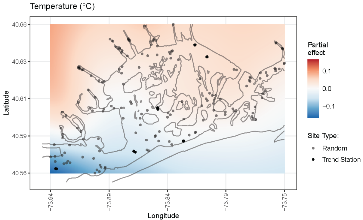
Figure 2-12. Mean surface for the generalized additive model latitude/longitude smooth of surface temperature within Gateway National Recreation Area during 2003-2018.
