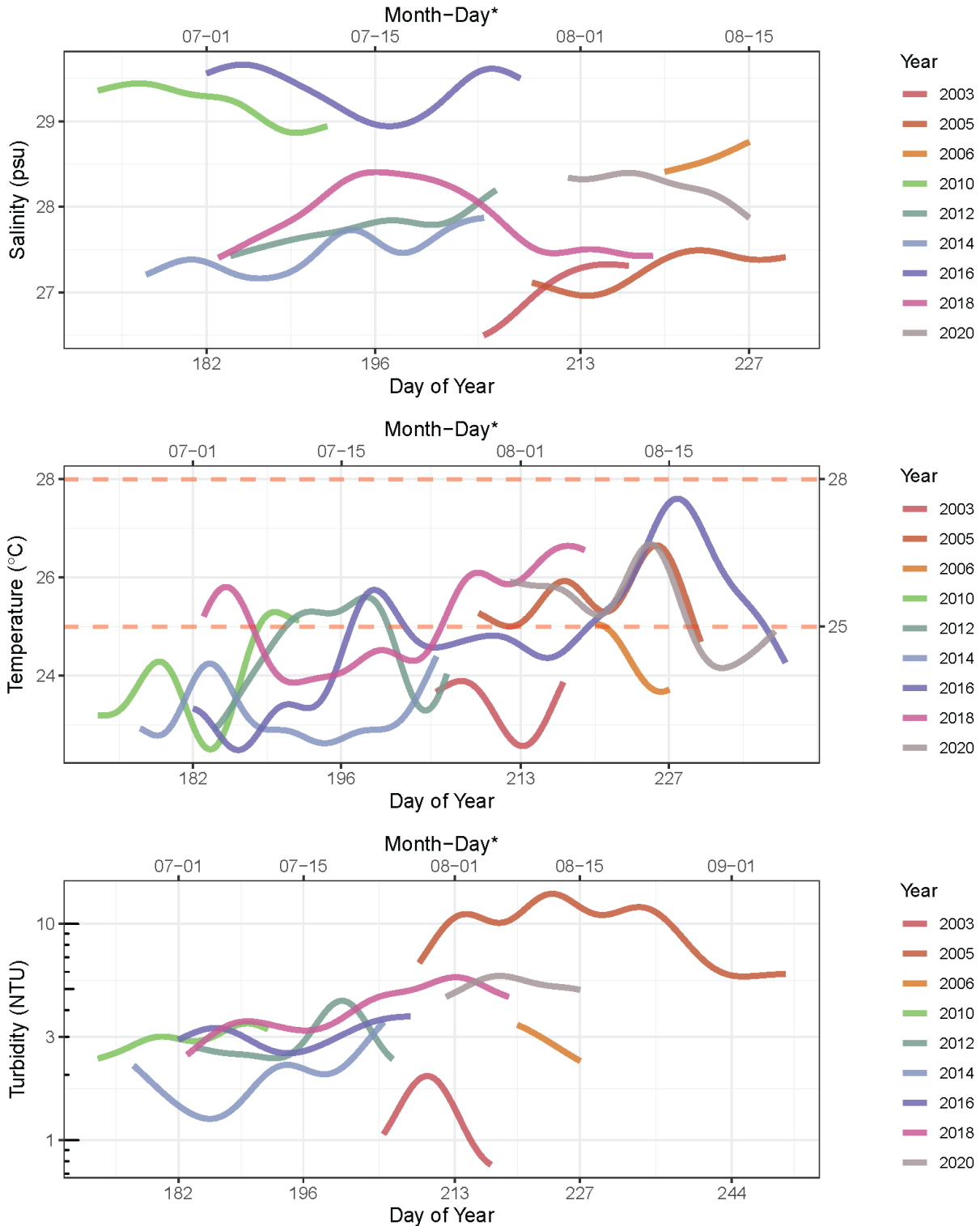
Figure 4-4. Intra-annual trends in surface salinity (top), surface temperature (middle), and surface turbidity (bottom) at the Gateway National Recreation Area logging station based on estimated generalized additive model smooths. Estuarine quality category thresholds (Table 2-1) plotted as red dashed lines. Note: the surface turbidity y-axis is transformed to the log 10 scale to better visualize the estimated trends.
