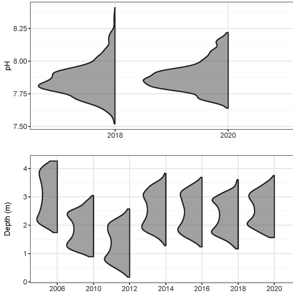
Figure 4-7. Distribution of index period time series values for pH (top) and depth (bottom) at the Gateway National Recreation Area logging station.
