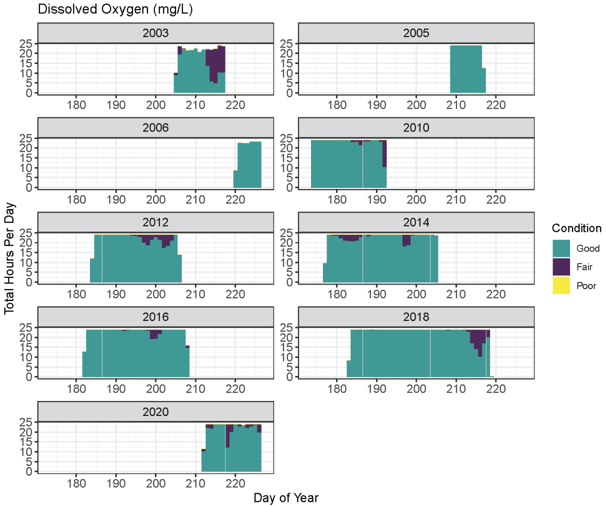
Figure 4-9. Total hours per day that bottom dissolved oxygen concentration was observed within each condition category at the Gateway National Recreation Area logging station.
