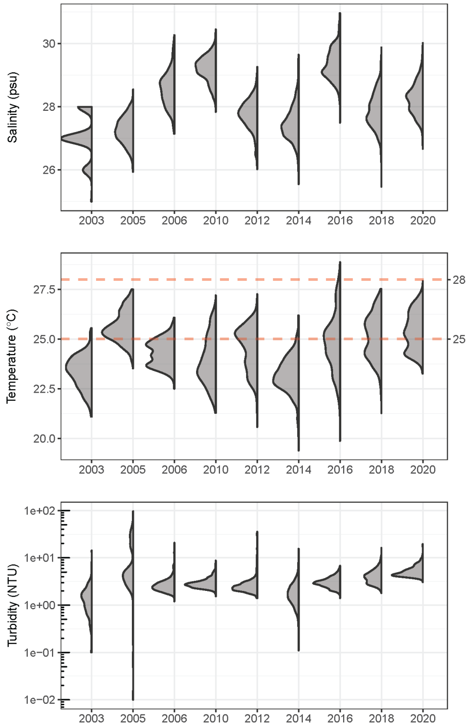
Figure 4-5. Distribution of index period time series values for surface salinity (top), surface temperature (middle), and surface turbidity (bottom) at the Gateway National Recreation Area logging station. Estuarine quality category thresholds (Table 2-1) plotted as red dashed lines. Note: the surface turbidity y-axis is transformed to the log 10 scale to better visualize the estimated distributions.
