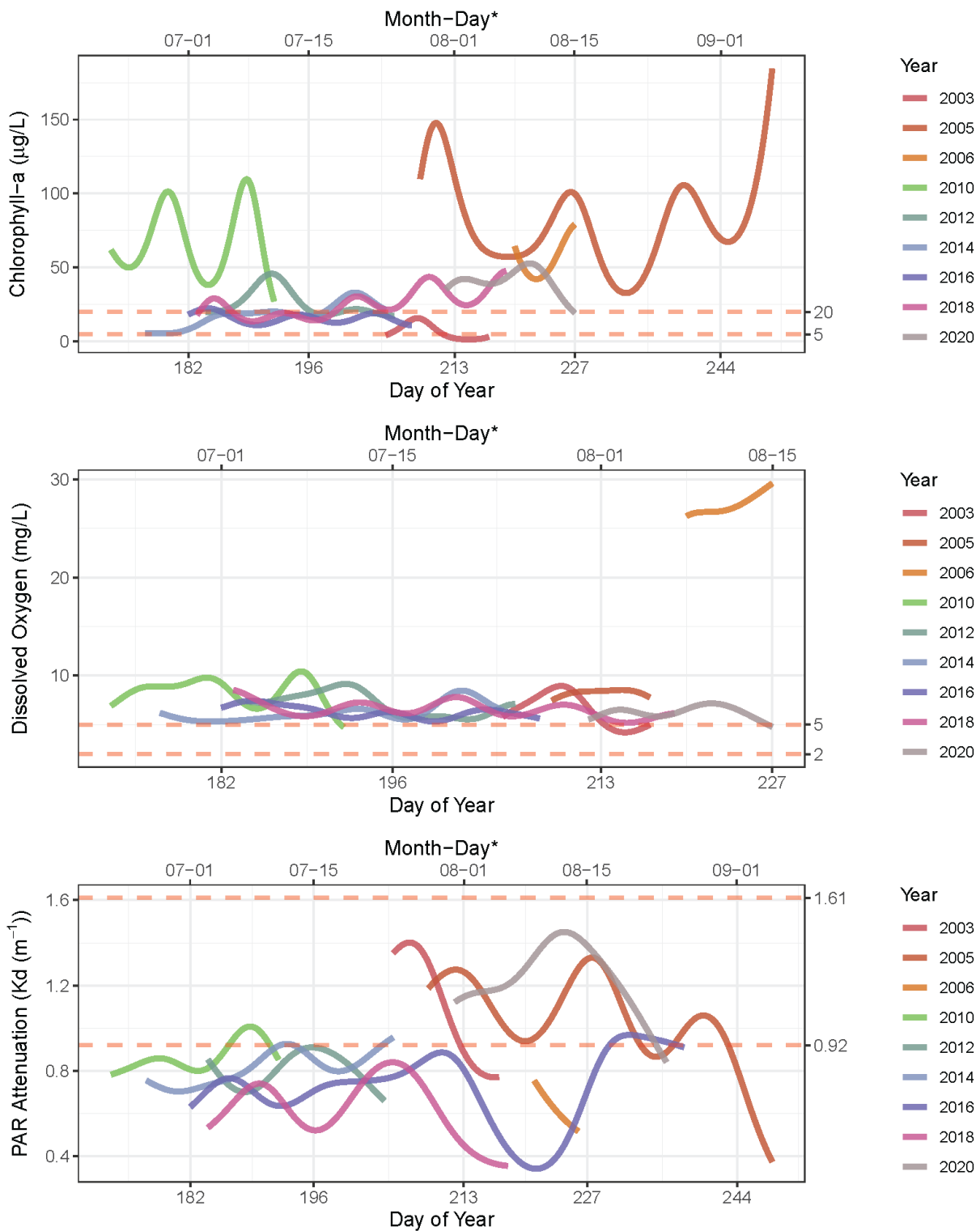
Figure 4-2. Intra-annual trends in surface chlorophyll- a concentration (top), bottom dissolved oxygen concentration (middle), and PAR attenuation (bottom) at the Gateway National Recreation Area logging station based on estimated generalized additive model smooths. Estuarine quality category thresholds (Table 2-1) plotted as red dashed lines.
