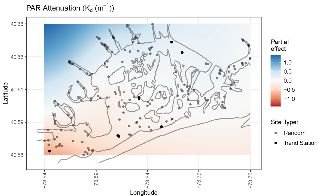
Figure 2-10. Mean surface for the generalized additive model latitude/longitude smooth of PAR attenuation within Gateway National Recreation Area during 2003-2018.
