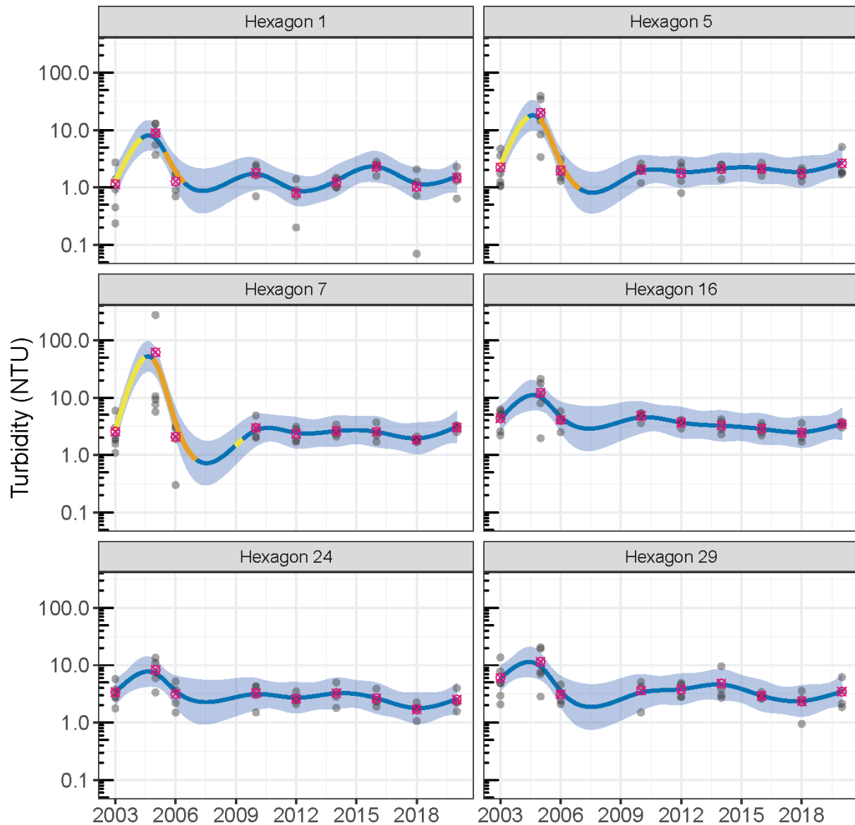
Figure 3-6. Mean surface turbidity (NTU) trend at each Gateway National Recreation Area trend station based on estimated generalized additive model smooths. The fitted smooth is plotted in dark blue with shaded 95% confidence interval. Periods of significant temporal change (increases/decreases), if present, are plotted in yellow/orange. Within each year, individual measurements and the average are plotted in gray and magenta, respectively. Note: the y-axis is transformed to the log 10 scale to better visualize the estimated trend.
