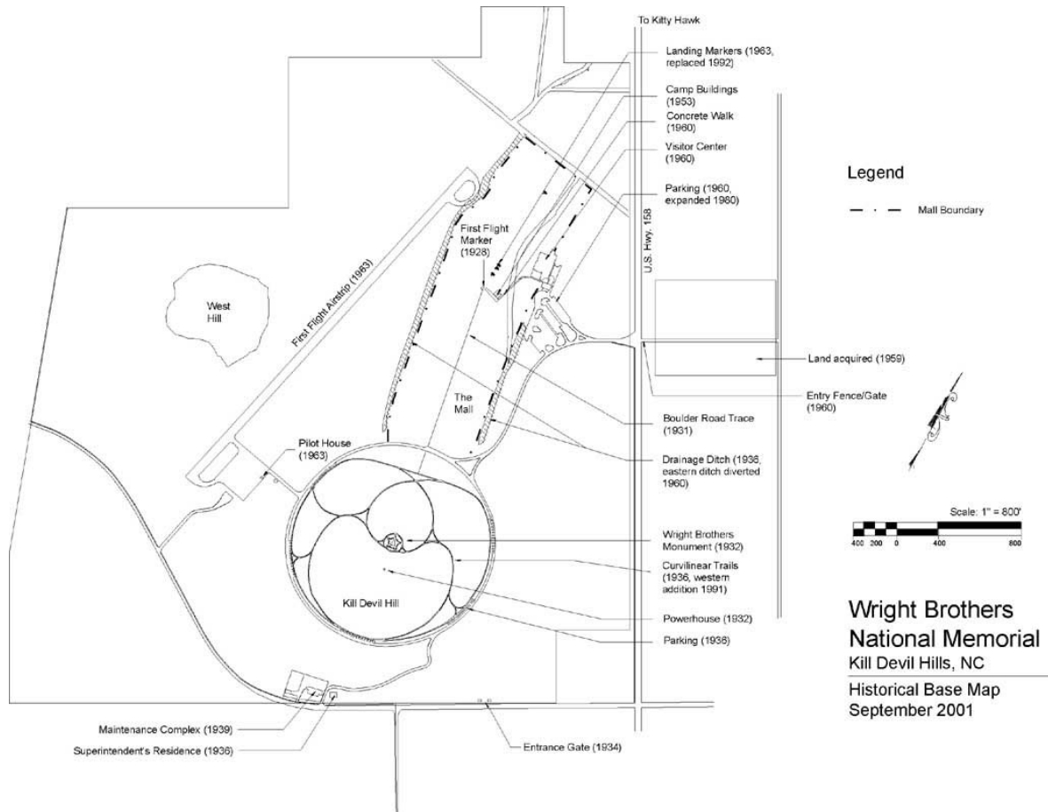
Fig 1. Site Plan 1 – Historical Base Map
