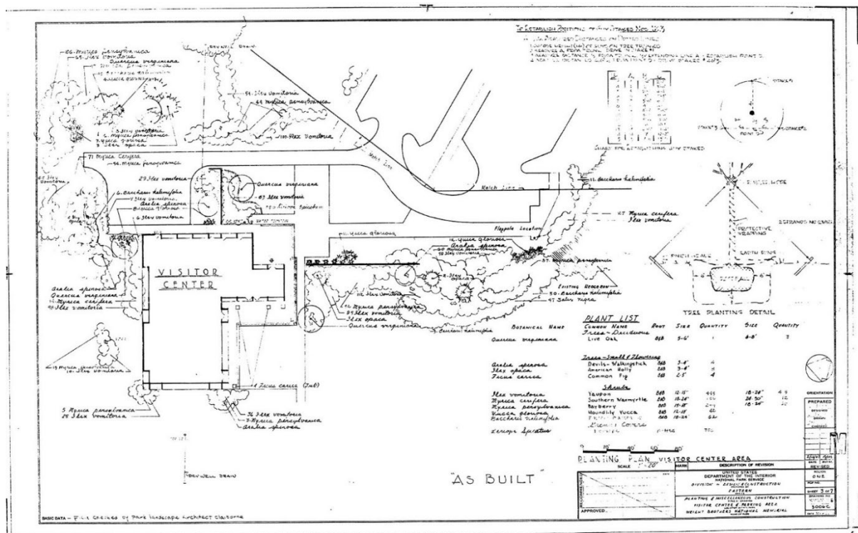
Fig 64. 1960 Planting Plan for Visitor Center Area
