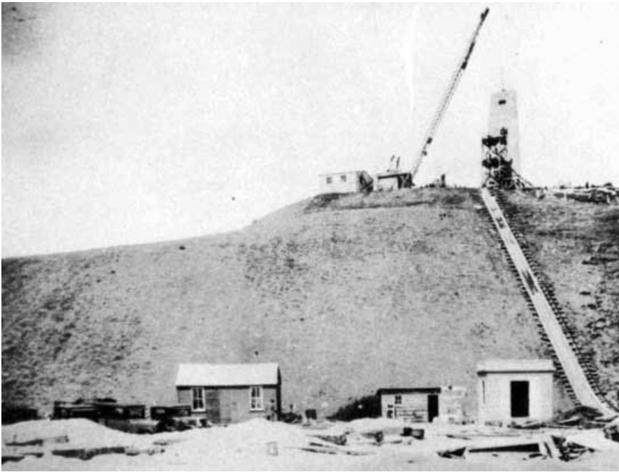
Fig 15. Monument and power house construction, 1932
