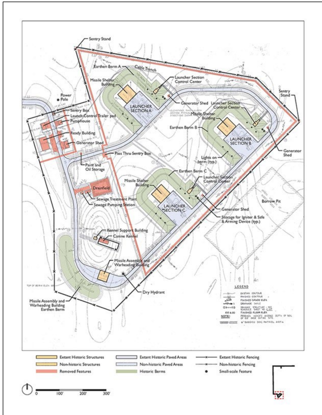
Fig 1. Launch Area site plan. Source: JMA, 2011; placed over 1964 as-built grading and drainage plan, NPS drawing 160 61071B, Sheet C-11.
