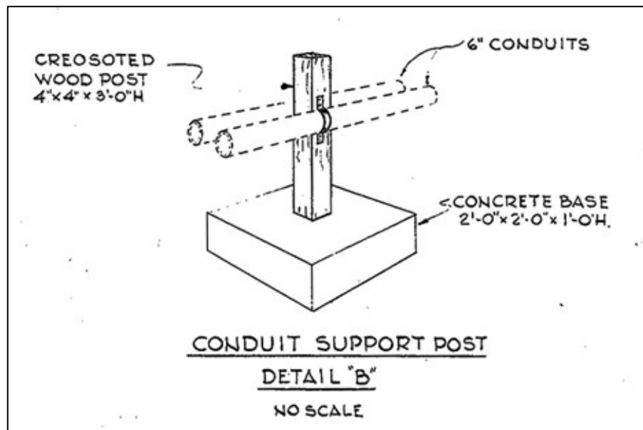
Fig 115. Creosoted wood post for conduit support, detail from the as-built construction document.
