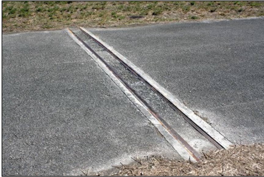
Fig 112. Cable trenches carried electrical cables beneath the roadway. The trenches were filled with concrete following the removal of the cable trays. Source: JMA, 2010
