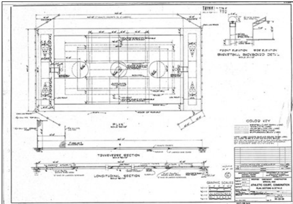
Fig 93. Construction plan for the athletic court, showing the layout of the lines, fencing, and backstops.
