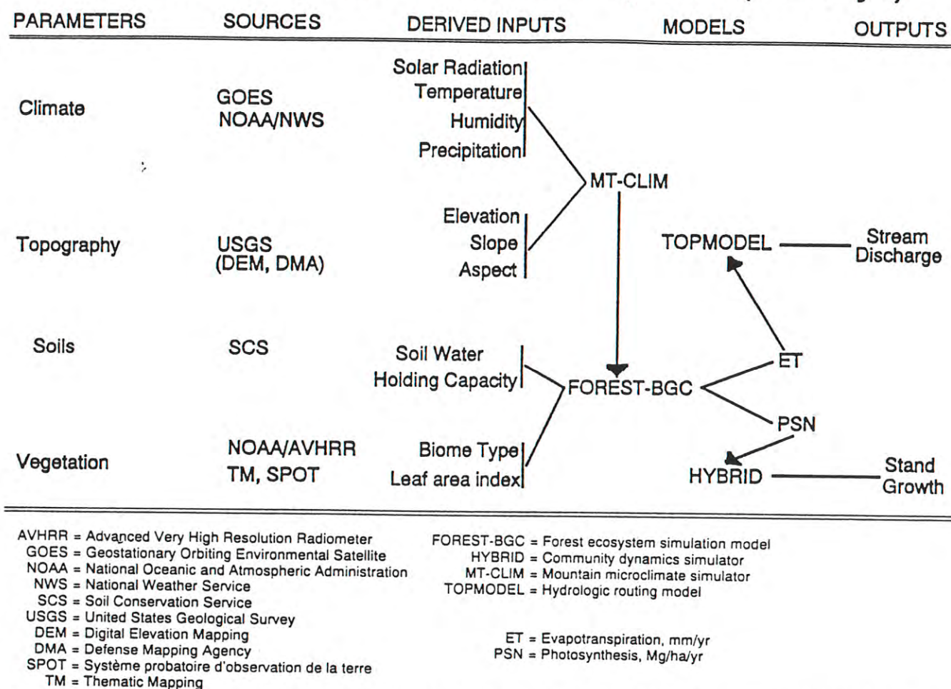
Figure 1. An organizational diagram for RESSys, showing the sources of raw climatic and biophysical data, the derived variables produced, and their incorporation into the topoclimate (MT-CLIM, Running et al., 1987) and ecosystem simulation (Forest-BGC, Running and Coughlan, 1988) models.
