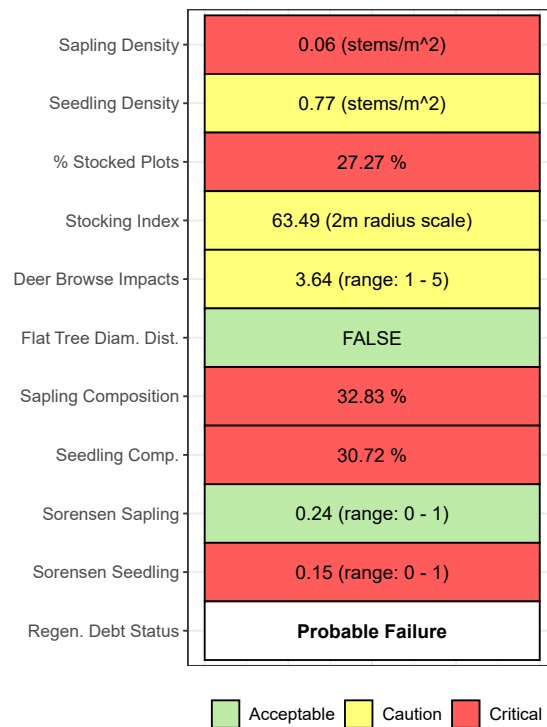
Figure 2. Regeneration Debt status for the most recent 4-year census (2019 – 2023) in Gettysburg National Military Park (GETT). Flat Tree Diam. Dist. stands for Flat Tree Diameter Distribution. If TRUE, the density of small trees is lower than expected due to chronic regeneration failure. Sapling/Seedling Composition is the % of total stems composed of native canopy-forming species. Sorensen is a measure of how closely the regen. layer matches canopy composition. For more details on metric calculations, thresholds and assessment of status, see Miller et al. 2023 ( https://esajournals.onlinelibrary.wiley.com/doi/full/10.1002/eap.2837 ).
