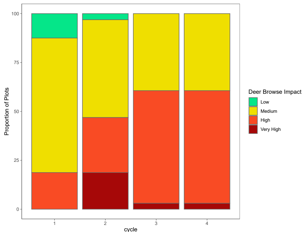
Figure 3. Deer browse impacts by cycle in Gettysburg National Military Park (GETT). Cycle 1: 2007 – 2010; Cycle 2: 2011 – 2014; Cycle 3: 2015 – 2018; Cycle 4: 2019 – 2023.
