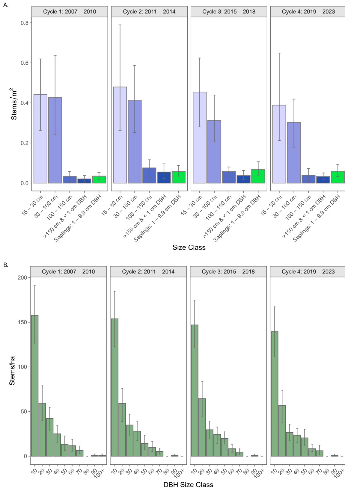
Figure 1. Stem density distributions by cycle in Gettysburg National Military Park (GETT). Cycle 1: 2007 – 2010; Cycle 2: 2011 – 2014; Cycle 3: 2015 – 2018; Cycle 4: 2019 – 2023. Figure A shows regeneration densities by size class. Figure B shows tree density by diameter at breast height (DBH) increments. Error bars are 95% bootstrapped confidence intervals to account for non-normal error. An asterisk denotes a linear DBH distribution that is indicative of long-term recruitment failure.
