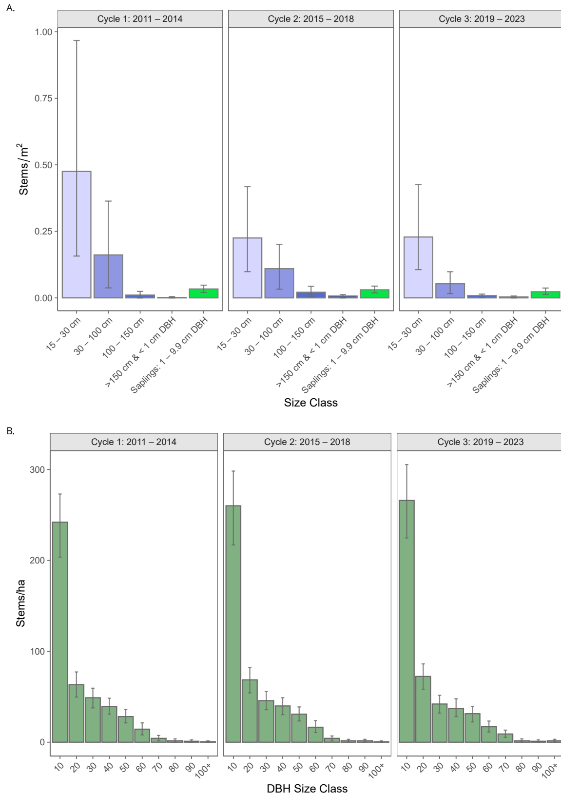
Figure 1. Stem density distributions by cycle in Colonial National Historical Park (COLO). Cycle 1: 2011 – 2014; Cycle 2: 2015 – 2018; Cycle 3: 2019 – 2023. Figure A shows regeneration densities by size class. Figure B shows tree density by diameter at breast height (DBH) increments. Error bars are 95% bootstrapped confidence intervals to account for non-normal error. An asterisk denotes a linear DBH distribution that is indicative of long-term recruitment failure.
