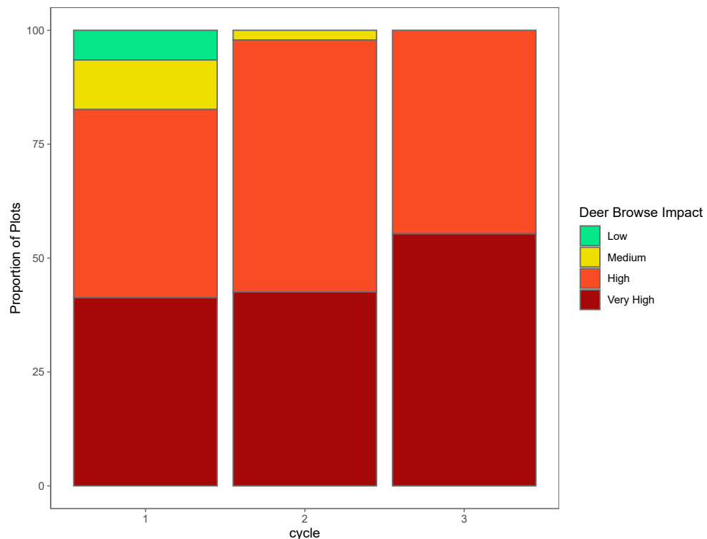
Figure 3. Deer browse impacts by cycle in Colonial National Historical Park (COLO). Cycle 1: 2011 – 2014; Cycle 2: 2015 – 2018; Cycle 3: 2019 – 2023.
