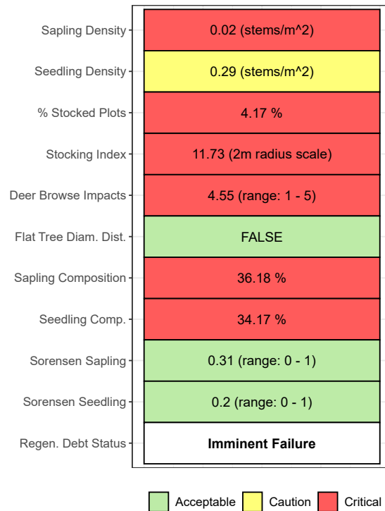
Figure 2. Regeneration Debt status for the most recent 4-year census (2019 – 2023) in Colonial National Historical Park (COLO). Flat Tree Diam. Dist. stands for Flat Tree Diameter Distribution. If TRUE, the density of small trees is lower than expected due to chronic regeneration failure. Sapling/Seedling Composition is the % of total stems composed of native canopy-forming species. Sorensen is a measure of how closely the regen. layer matches canopy composition. For more details on metric calculations, thresholds and assessment of status, see Miller et al. 2023 ( https://esajournals.onlinelibrary.wiley.com/doi/full/10.1002/eap.2837 ).
