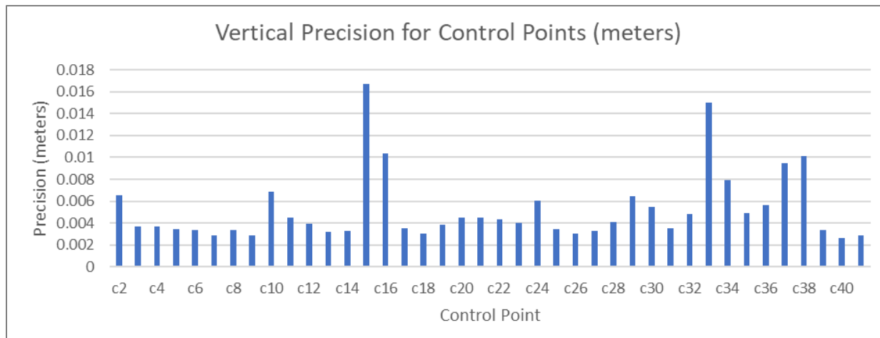
Figure 9. Graph comparing the vertical precision for control points set using the R12i GNSS receiver and the NTRIP base station.
