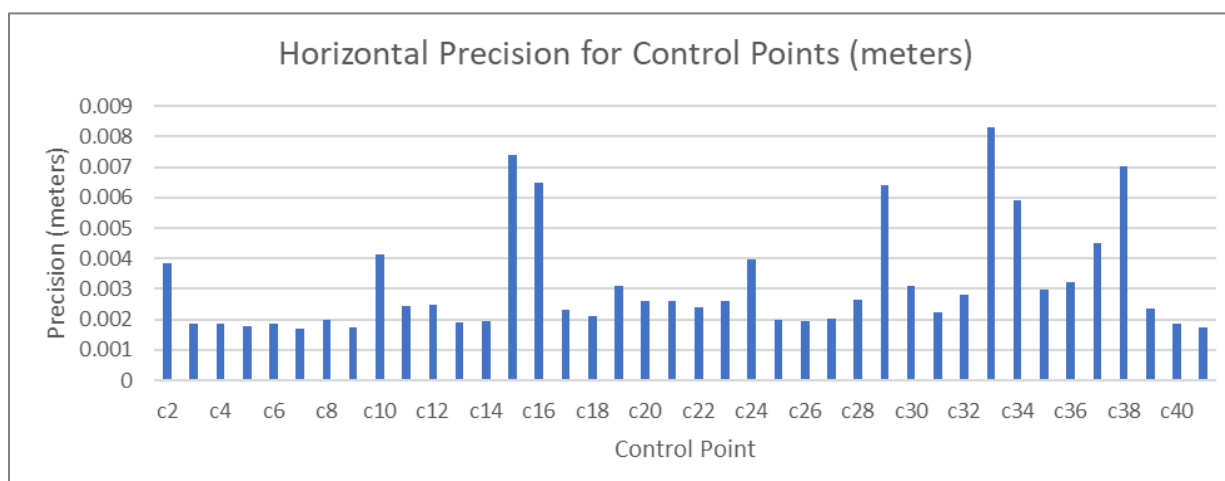
Figure 8. Graph comparing the horizontal precision for control points set using the R12i GNSS receiver and the NTRIP base station.
