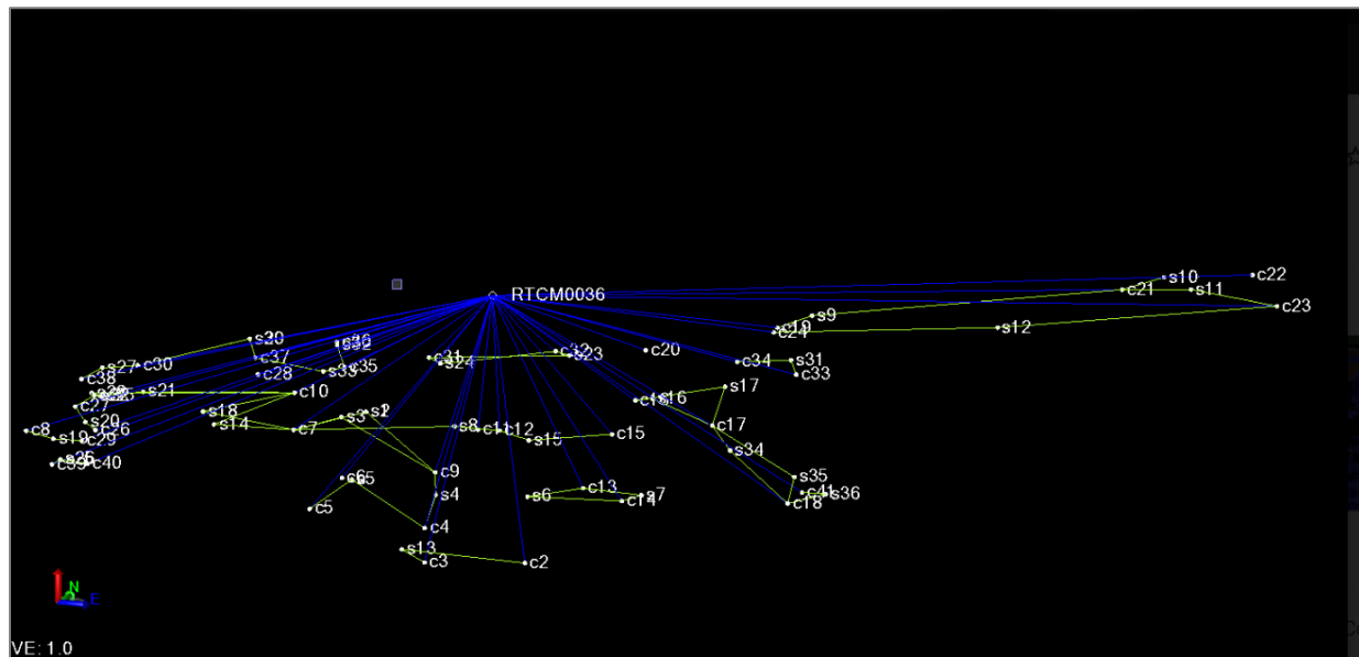
Figure 4. Two-dimensional view of each control point and scan at Charlestown Navy Yard, Boston National Historical Park. The blue lines represent the control points' connection to the NTRIP base station, and the green lines represent the resection for each scan, depicting which control points were used for a given scan.
