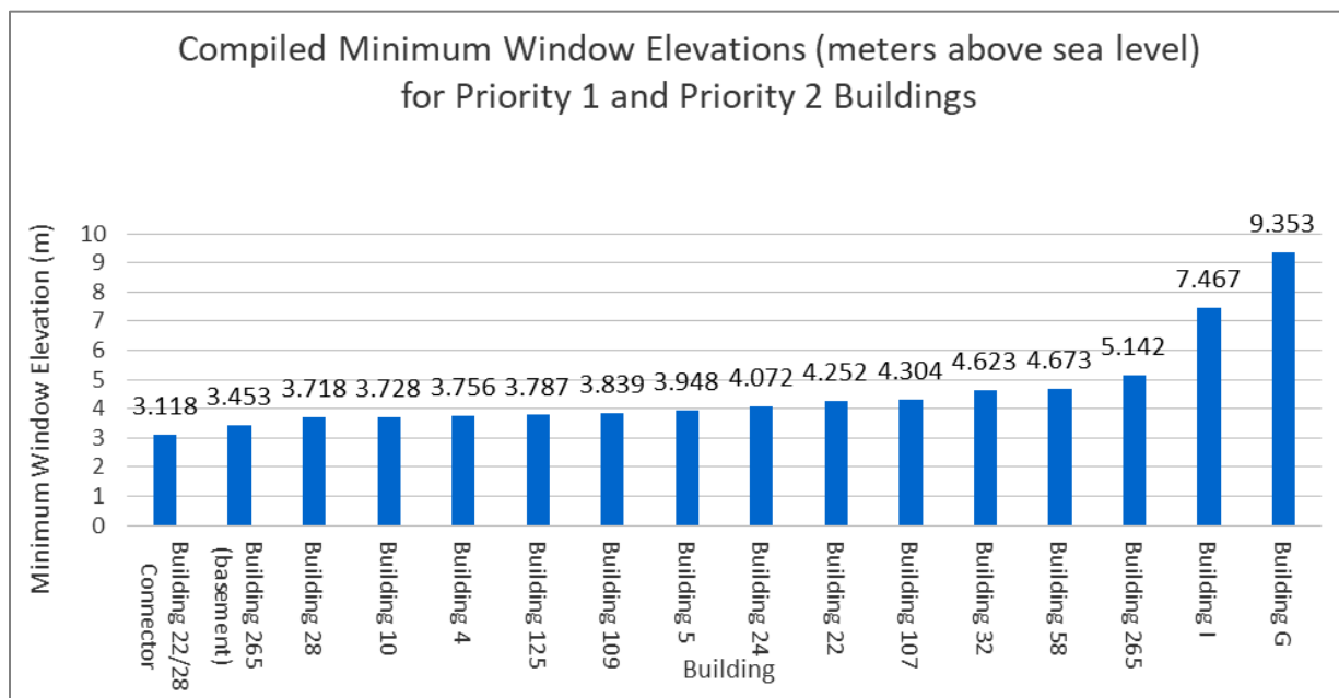
Figure 11. Graph showing the minimum window elevations for the fourteen Priority 1 and Priority 2 buildings with windows, the Building 22/28 connector, and the minimum basement window elevation for Building 265 at Charlestown Navy Yard, Boston National Historical Park.
