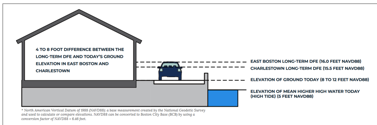
Figure 13. Diagram explaining the design flood elevation (DFE). Source: City of Boston (2022). CITY OF BOSTON
