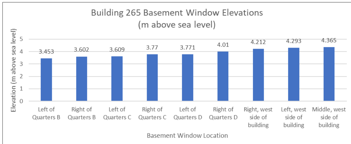
Figure 12. Graph depicting the elevations of the basement windows on Building 265 at Charlestown Navy Yard, Boston National Historical Park.
