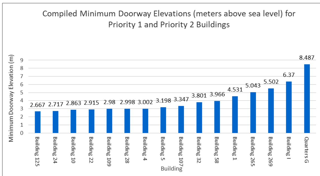
Figure 10. Graph showing the minimum doorway elevations for the sixteen Priority 1 and Priority 2 buildings at Charlestown Navy Yard, Boston National Historical Park.
