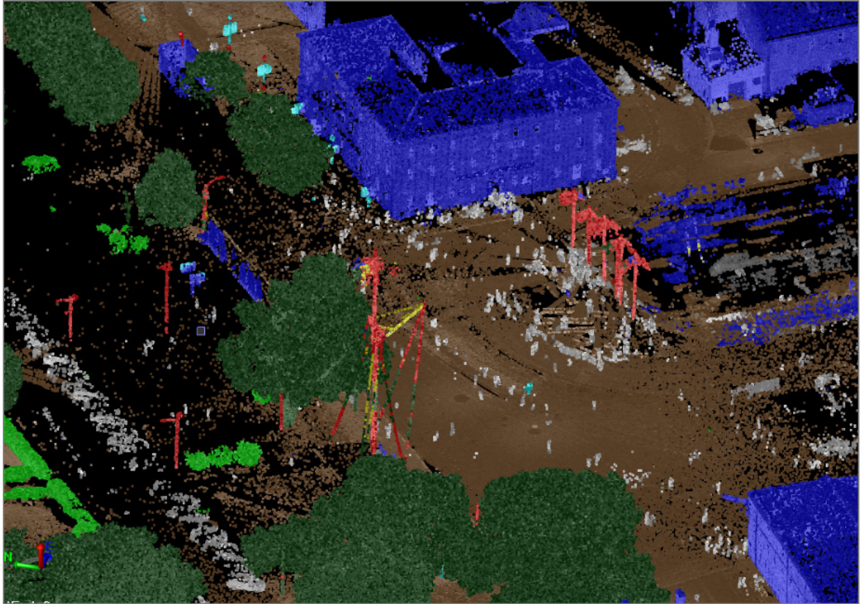
Figure 7. Point cloud view of the USS Constitution Museum and other features at the Charlestown Navy Yard, Boston National Historical Park. Blue points represent buildings, dark green points represent high vegetation, light green points represent low vegetation, red points represent poles, brown points represent the ground, and white points represent noise, which were typically people and cars in this setting.
