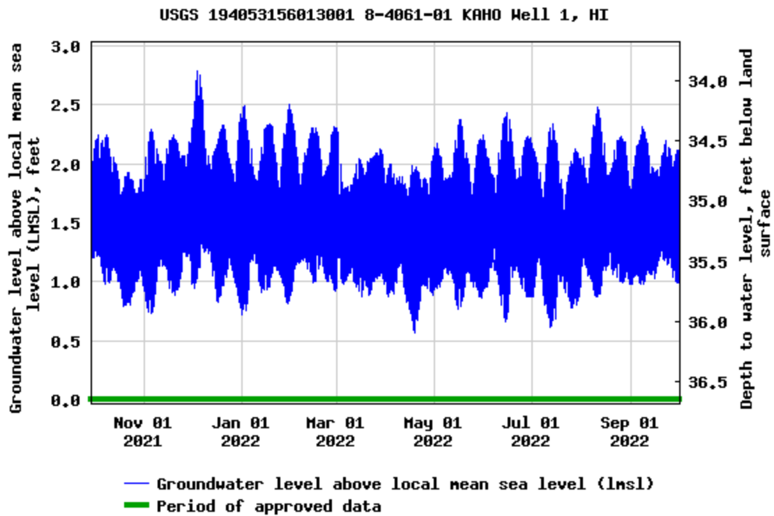
Figure 2. Water-level data for KAH0 Well 1, near the KAH0 Visitor Center, October 1, 2021–September 30, 2022.
