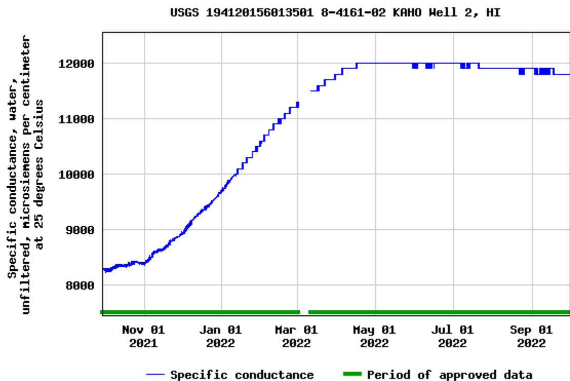
Figure 7. Specific-conductance data for KAH0 Well 2, the upper well, October 1, 2021–September 30, 2022.
