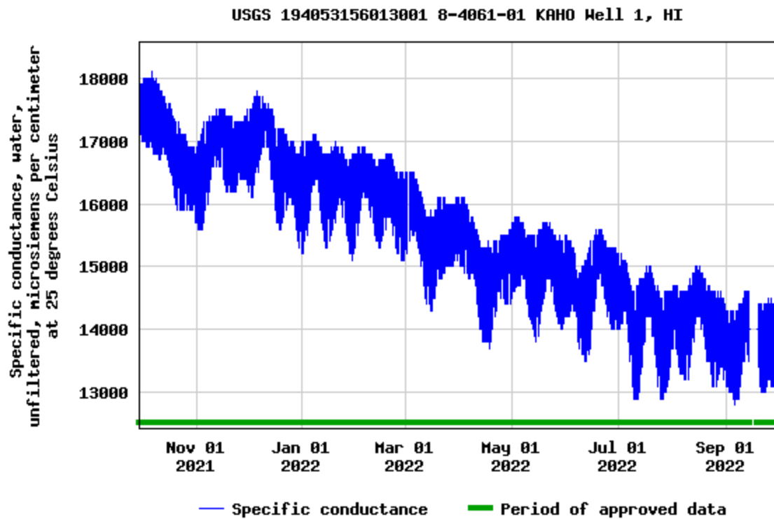
Figure 4. Specific-conductance data for KAHŌ Well 1, near the KAHŌ Visitor Center, October 1, 2021–September 30, 2022.
