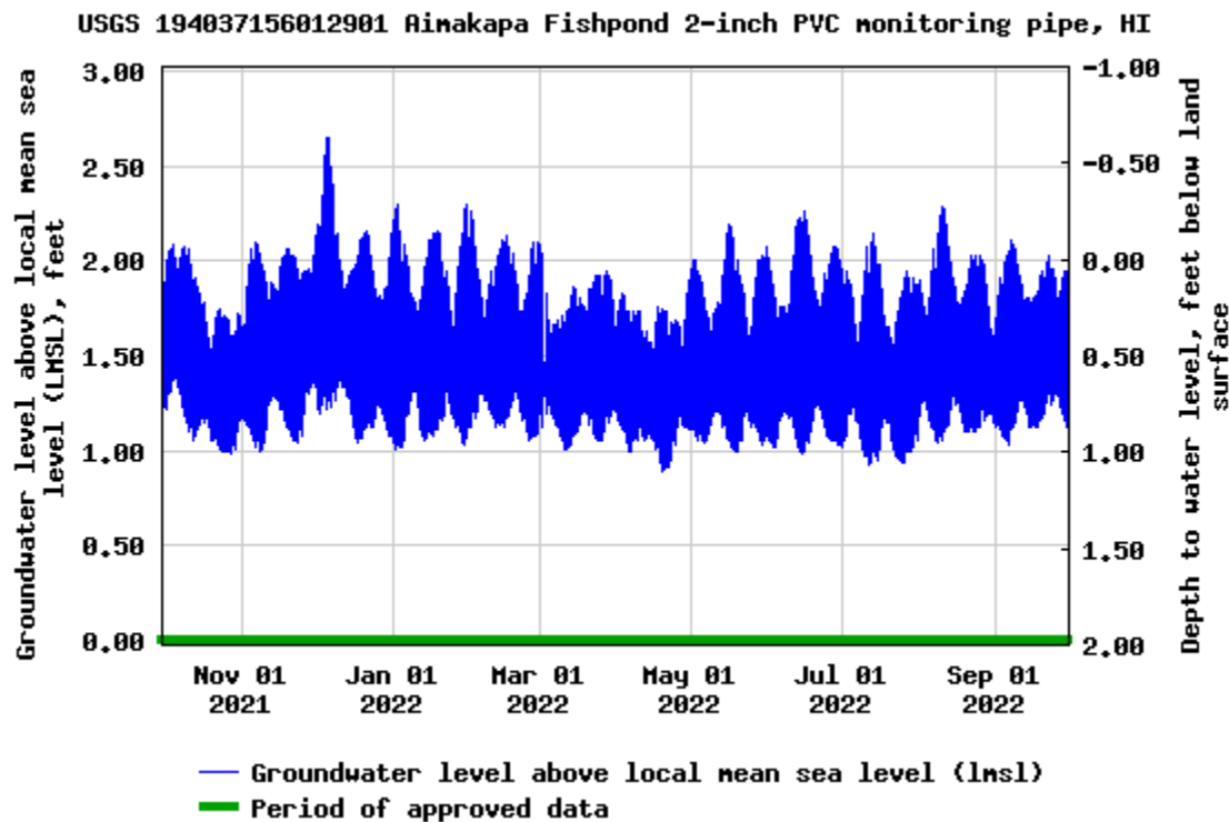
Figure 11. Water-level data for ‘Aimakapā Fishpond monitoring pipe, October 1, 2021–September 30, 2022.
