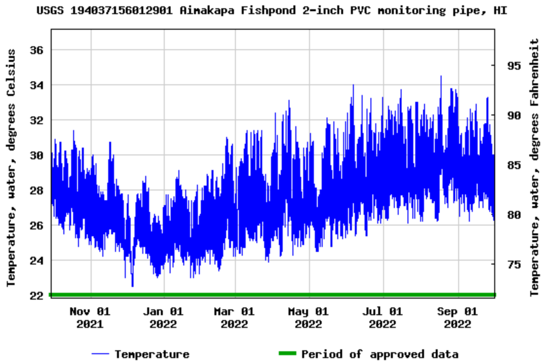
Figure 12. Temperature data for ‘Aimakapā Fishpond monitoring pipe, October 1, 2021–September 30, 2022.
