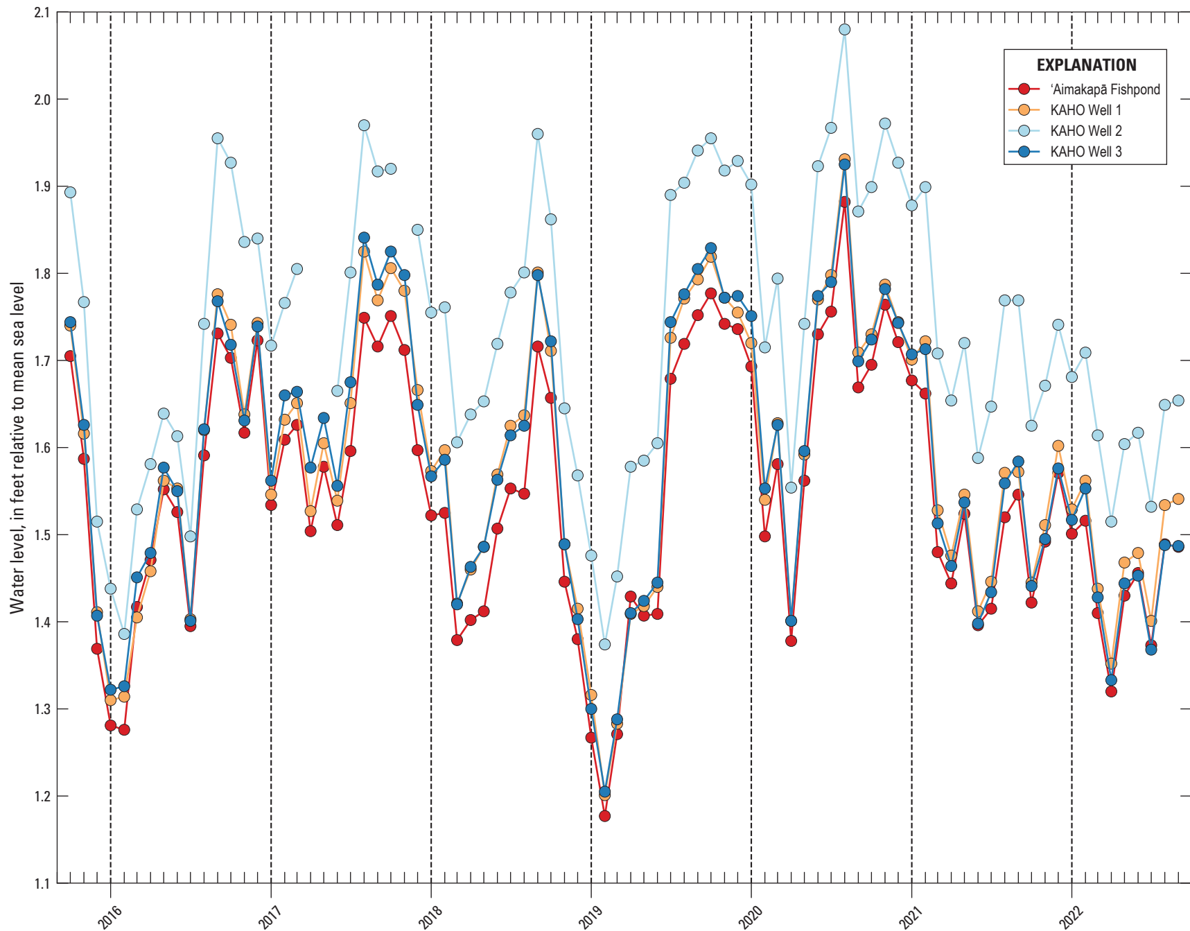
Figure 14. Monthly mean water level at four monitoring sites in Kaloko-Honokōhau (KAHO) National Historical Park, Island of Hawai'i, October 2015–September 2022, including months with incomplete data.
