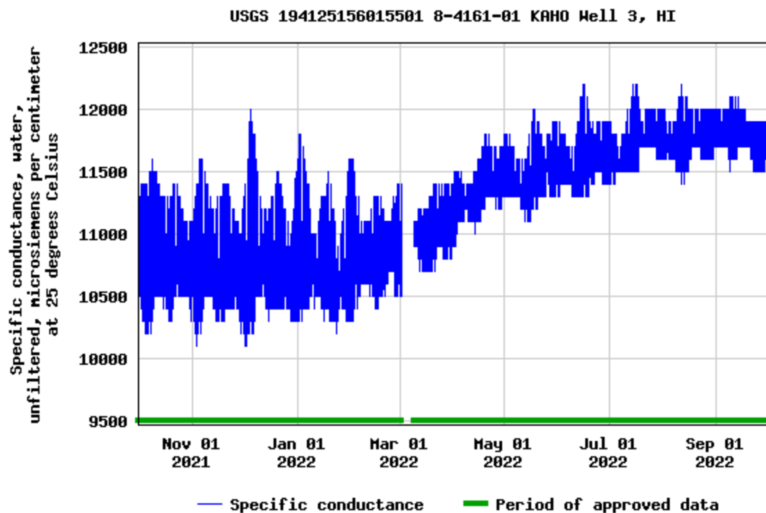
Figure 10. Specific-conductance data for KAH0 Well 3, the lower well, October 1, 2021–September 30, 2022.
