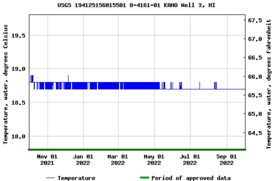
Figure 9. Temperature data for KAH0 Well 3, the lower well, October 1, 2021–September 30, 2022.
