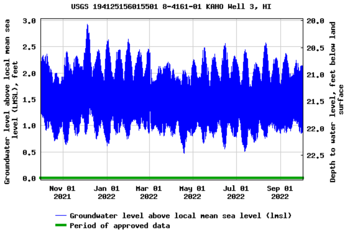
Figure 8. Water-level data for KAH0 Well 3, the lower well, October 1, 2021–September 30, 2022.
