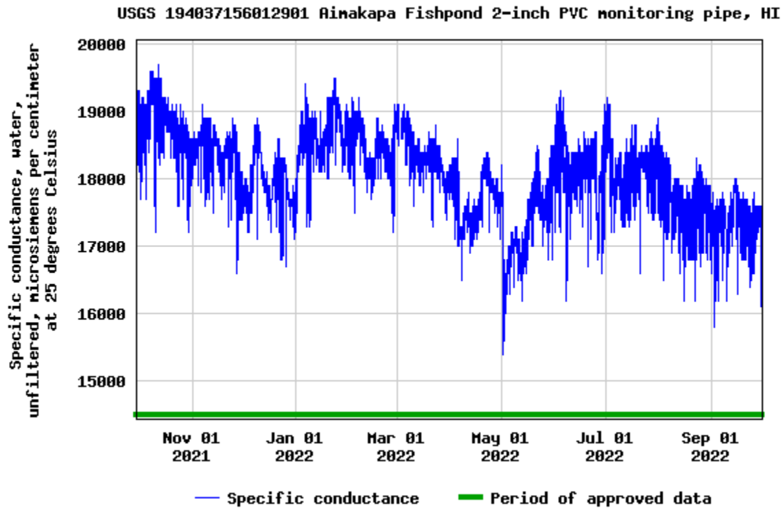
Figure 13. Specific-conductance data for ‘Aimakapā Fishpond monitoring pipe, October 1, 2021–September 30, 2022.
