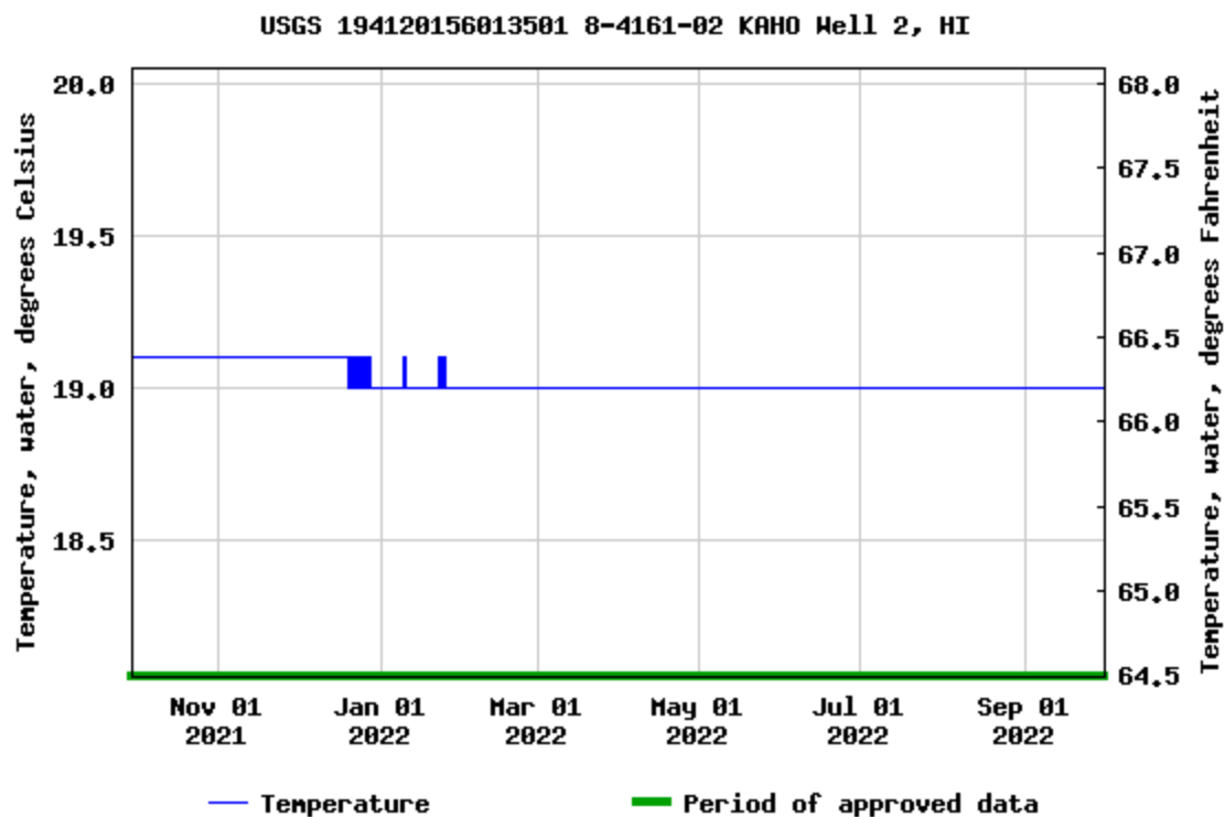
Figure 6. Temperature data for KAH0 Well 2, the upper well, October 1, 2021–September 30, 2022.
