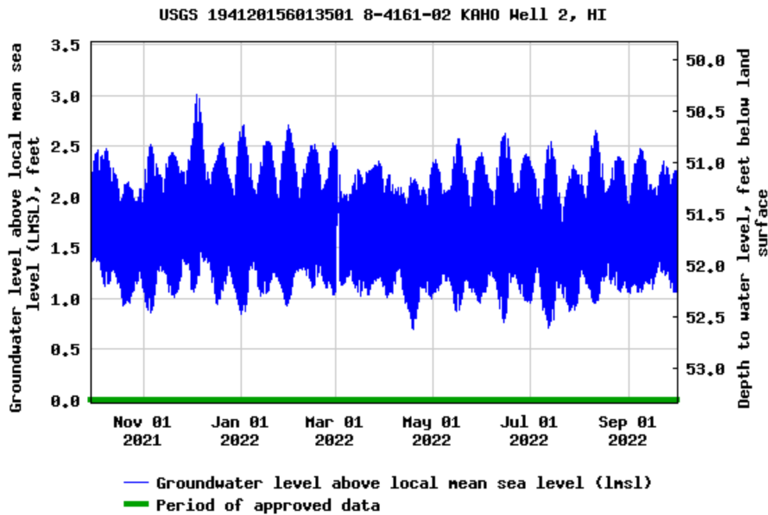
Figure 5. Water-level data for KAHŌ Well 2, the upper well, October 1, 2021–September 30, 2022.
