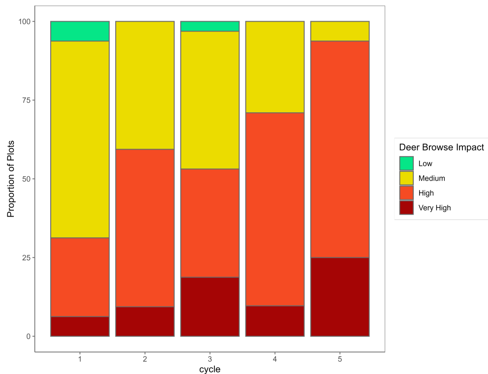
Figure 2. Deer browse impacts by cycle in Richmond National Battlefield Park (RICH). Cycle 1: 2007 – 2010; Cycle 2: 2011 – 2014; Cycle 3: 2015 – 2018; Cycle 4: 2019 – 2022; Cycle 5: 2023 – 2024. Note that Cycle 5 is only partially complete.
