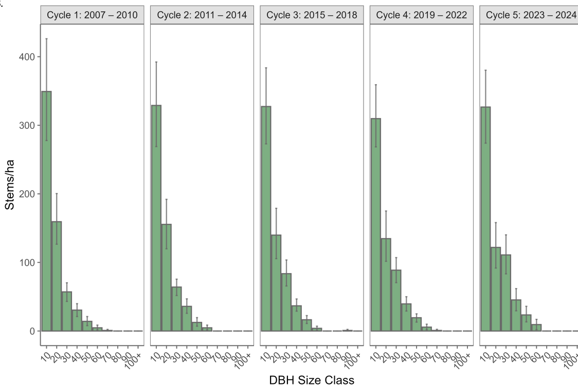
Figure 3. Stem density distributions by cycle in Richmond National Battlefield Park (RICH). Cycle 1: 2007 – 2010; Cycle 2: 2011 – 2014; Cycle 3: 2015 – 2018; Cycle 4: 2019 – 2022; Cycle 5: 2023 – 2024. Note that Cycle 5 is only partially complete. Figure A shows regeneration densities by size class. Figure B shows tree density by diameter at breast height (DBH) increments. Error bars are 95% bootstrapped confidence intervals to account for non-normal error. An asterisk denotes a linear DBH distribution that is indicative of long-term recruitment failure.
