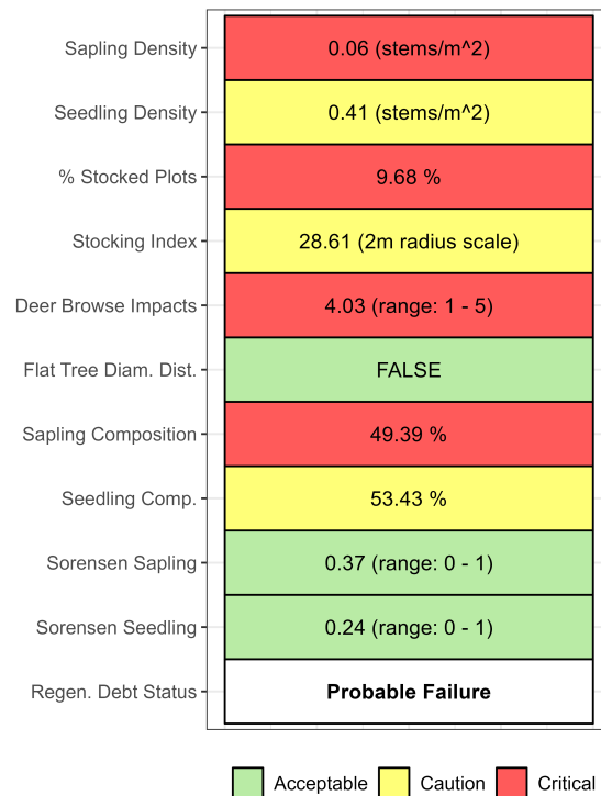
Figure 1. Regeneration Debt status for the most recent 4-year census (2021 – 2024) in Richmond National Battlefield Park (RICH). Flat Tree Diam. Dist. stands for Flat Tree Diameter Distribution. If TRUE, the density of small trees is lower than expected due to chronic regeneration failure. Sapling/Seedling Composition is the % of total stems composed of native canopy-forming species. Sorensen is a measure of how closely the regen. layer matches canopy composition. For more details on metric calculations, thresholds and assessment of status, see Miller et al. 2023 ( https://esajournals.onlinelibrary.wiley.com/doi/full/10.1002/eap.2837 ).
