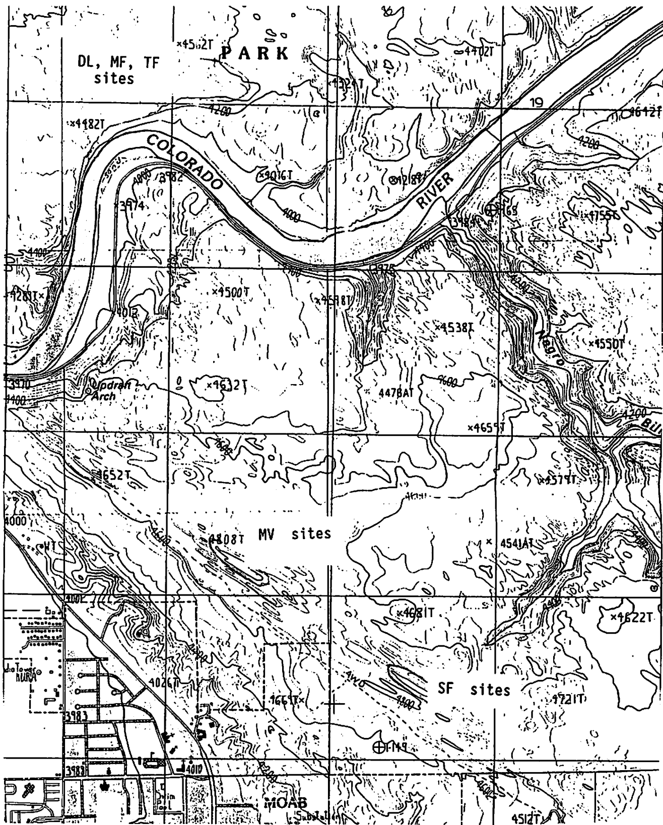
Figure 2. Sampling sites in Arches National Park and adjoining BLM land.
