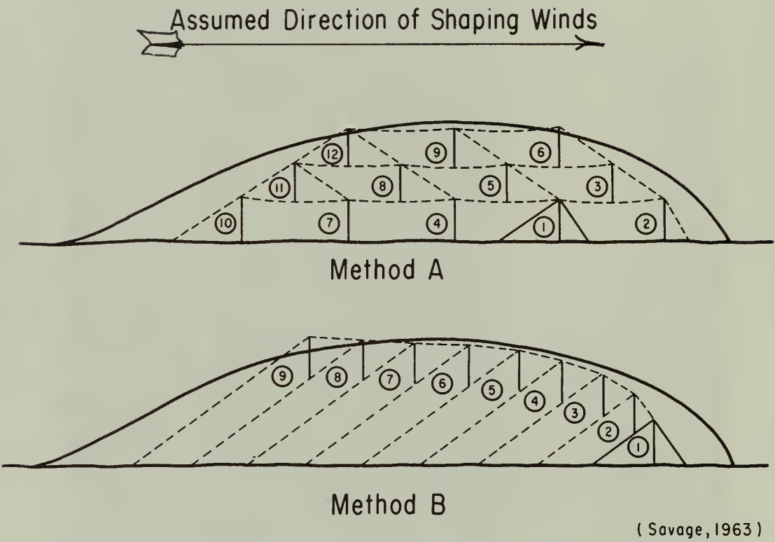
FIGURE 5. PROPOSED PROGRAMS FOR BUILDING A BARRIER DUNE
