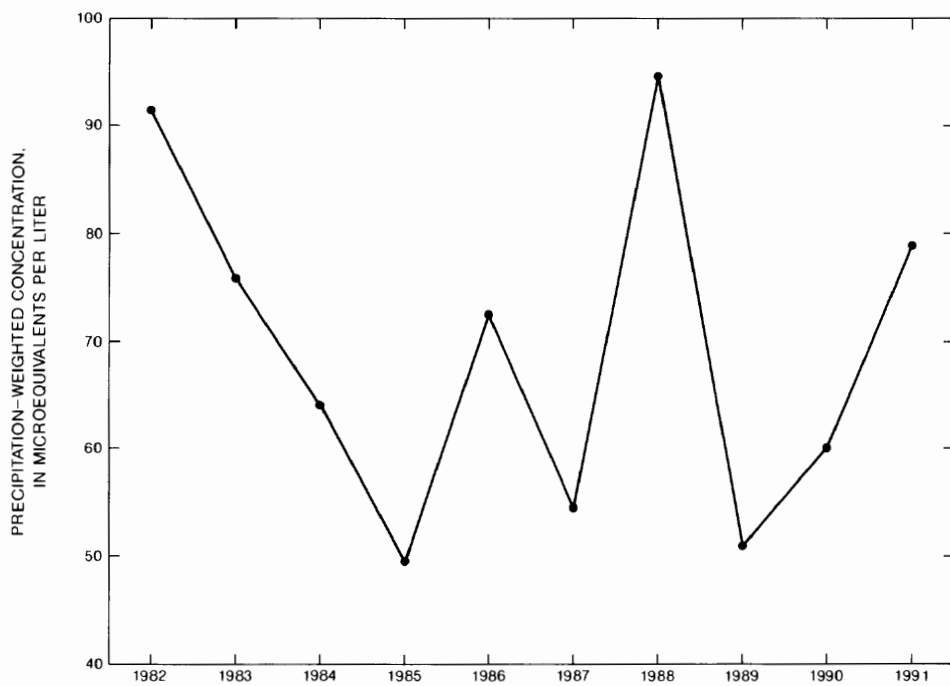
Figure 2. Annual precipitation-weighted mean field hydrogen-ion concentrations.
