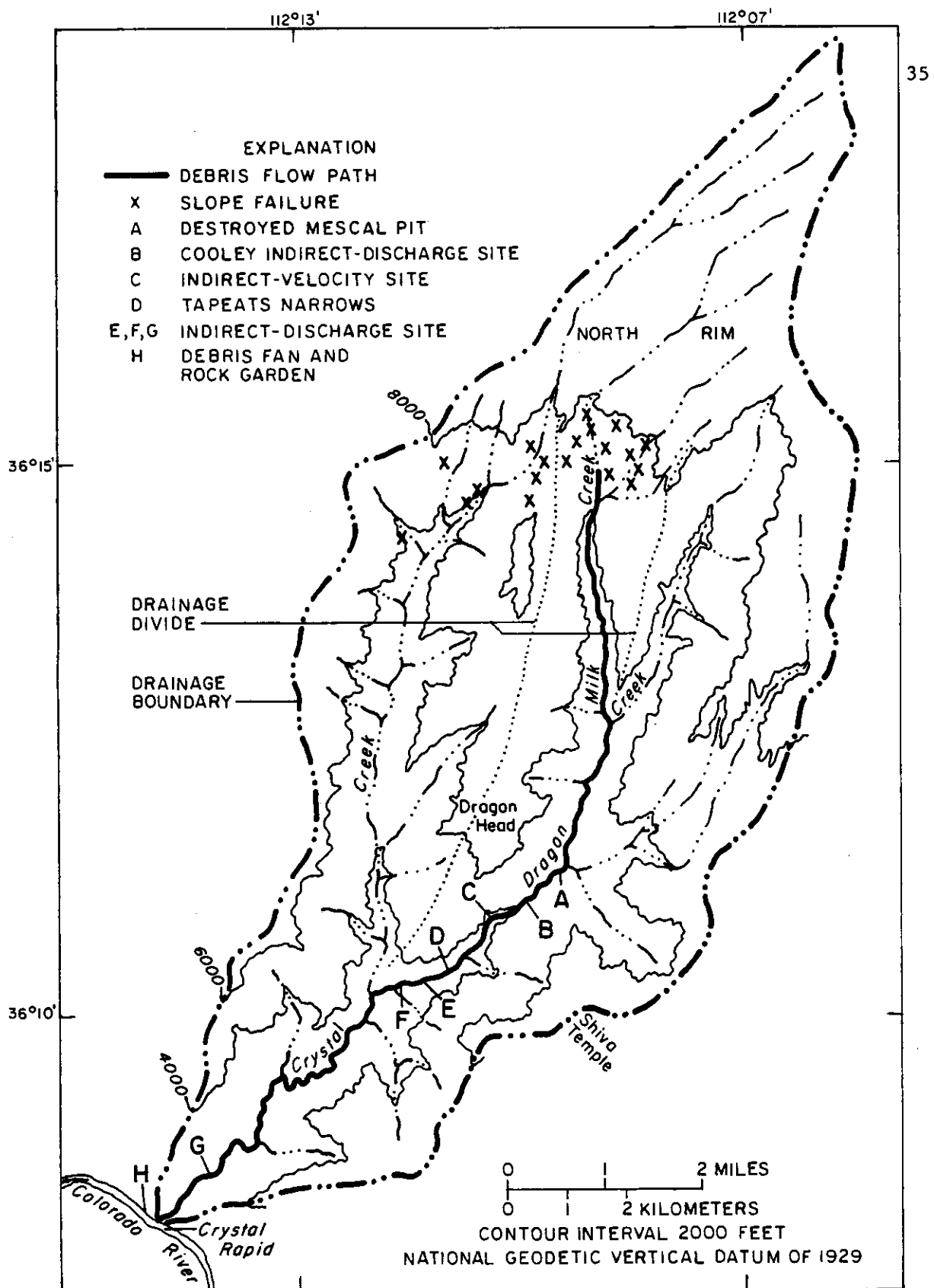
Figure 13.--The Crystal Creek drainage at mile 98.2 on the Colorado River.
