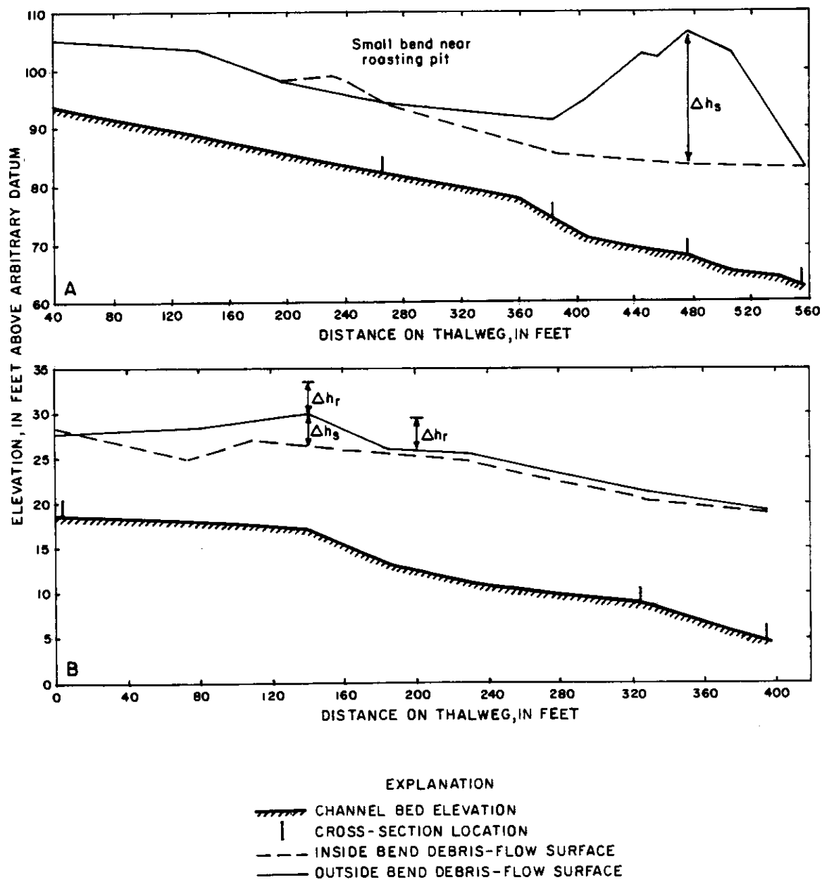
Figure 18.--Longitudinal profiles for indirect-discharge sites in the Crystal Creek drainage. A, Site G, 4.8 miles upstream from the Colorado River. B, Site 1, 0.9 mile upstream from the Colorado River.
