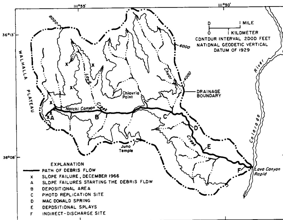
Figure 2.--The Lava-Chuar Creek drainage at mile 65.5 on the Colorado River.
