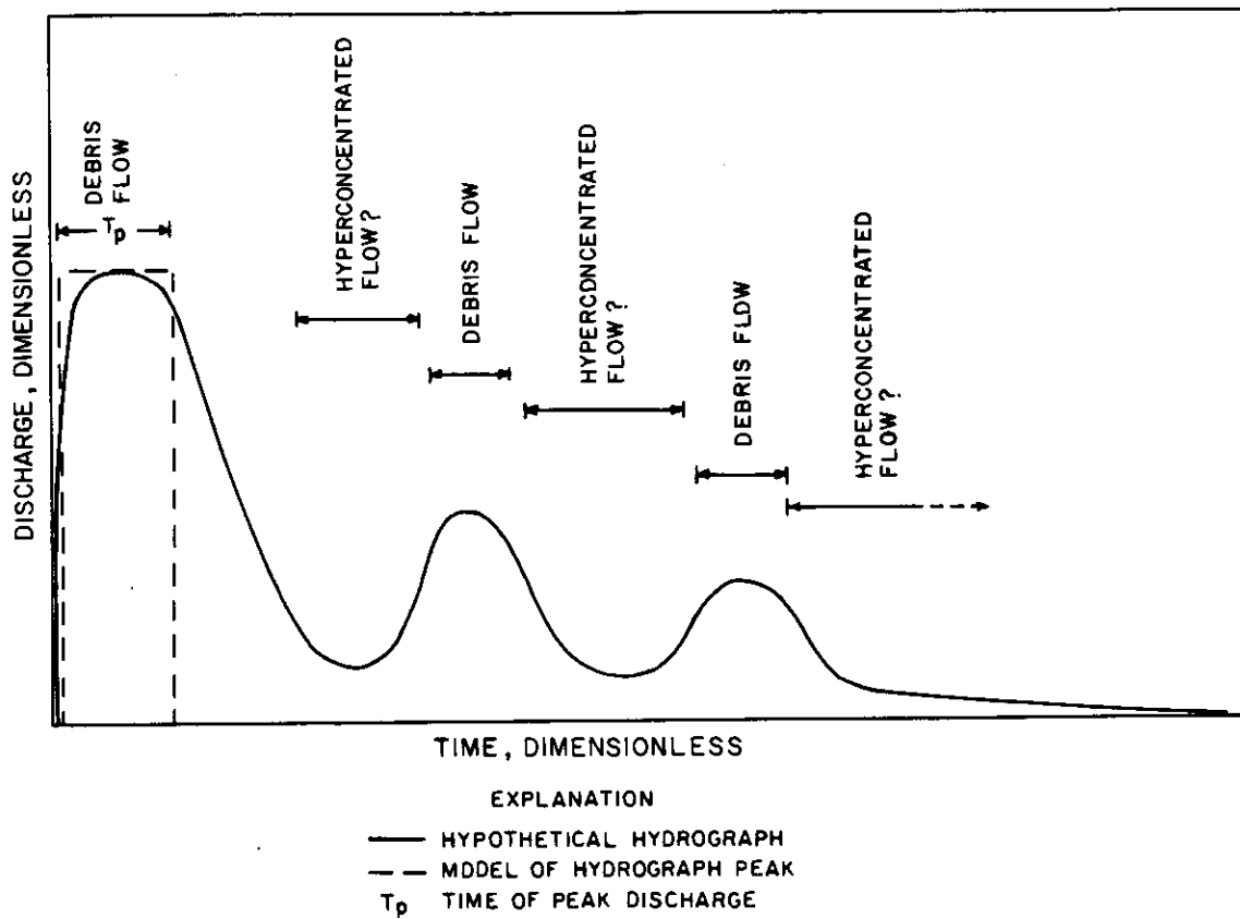
Figure 12.--Hypothetical hydrograph of the debris flow of 1984 in Monument Creek as suggested by stratigraphic evidence.
