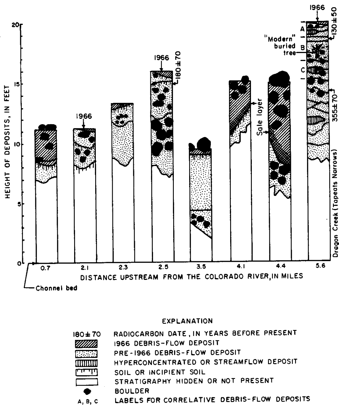
Figure 14.--Stratigraphy of debris-flow deposits in the Crystal Creek drainage.
