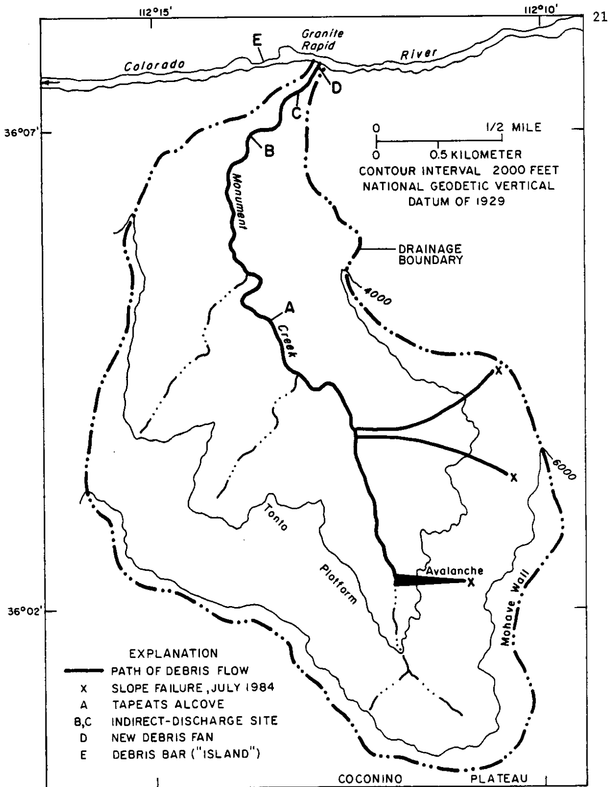
Figure 7.--The Monument Creek drainage at mile 93.5 on the Colorado River.
