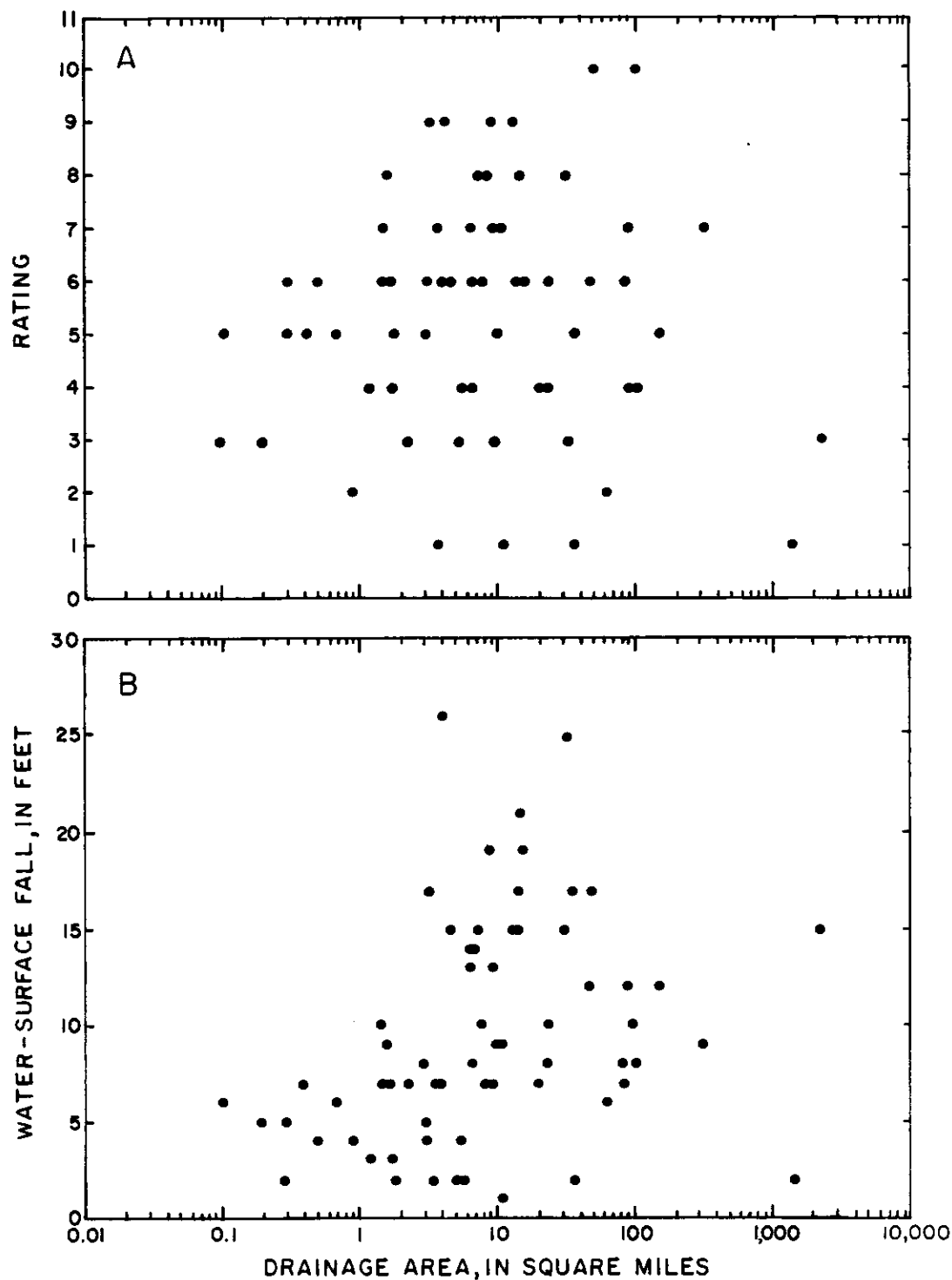
Figure 19.--Relation of characteristics of rapids and the contributing drainage area of the tributaries. A , Using the "rapid rating" (scale of 1 to 10; Stevens, 1983) for a discharge of 10,000 cubic feet per second in the Colorado River. B , Using the water-surface fall surveyed in 1921 and adjusted to 10,000 cubic feet per second. This fall may have significantly changed as a result of historic debris flows, especially at Crystal Rapid.
