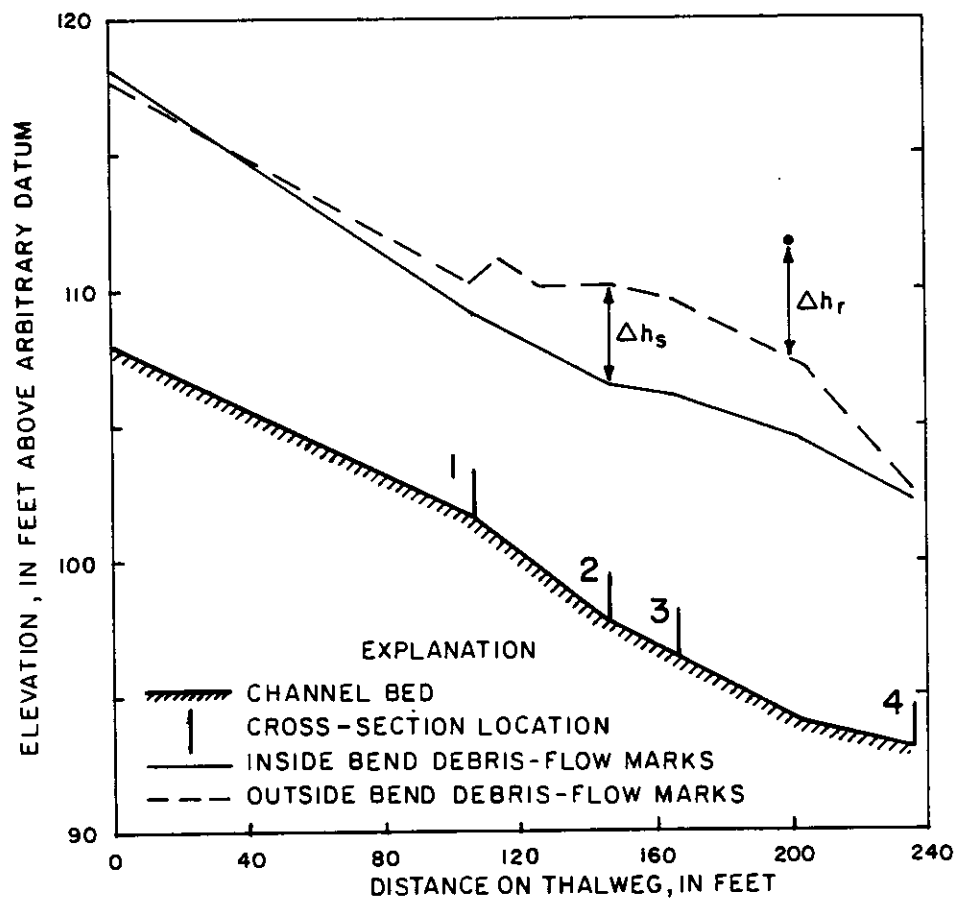
Figure 11.--Plan map and longitudinal profile for indirect-discharge site B in Monument Creek, 0.5 mile upstream from the Colorado River.
