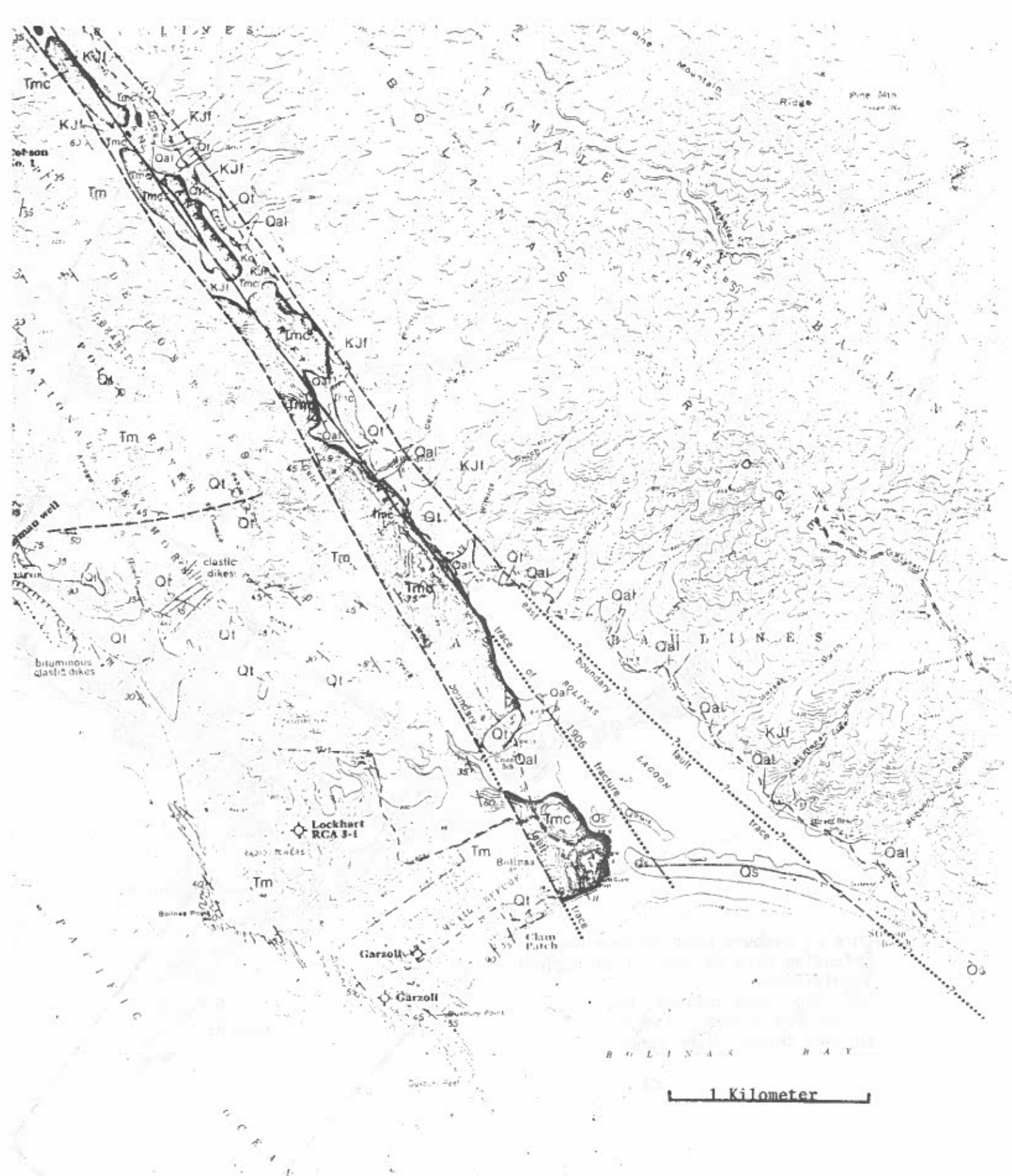
Figure 2. Map showing relationship of Duxbury Reef, Bolinas Lagoon, and the San Andreas Fault. (From Calloway, 1976).
