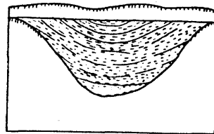
POORLY SORTED SAND, SILT AND CLAY, TRUNCATED BY WINDBLOWN MATERIAL, ALL DERIVED LOCALLY
