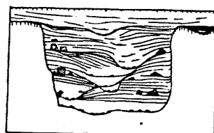
AGGRADING CHANNEL WITH BANK BUILD-UP
