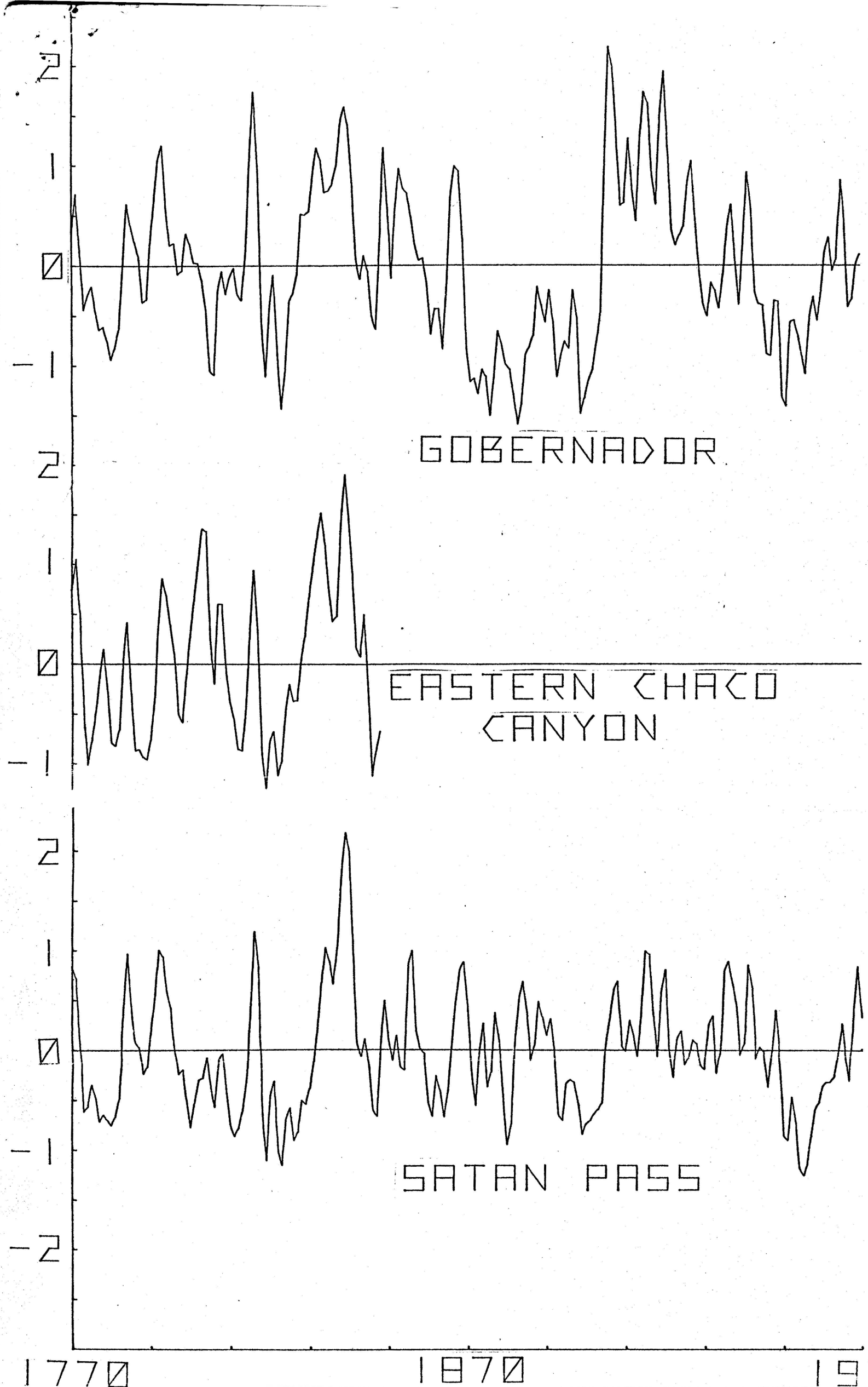
Plot of standardized three-year running weighted averages of tree ring indices from eastern Chaco Canyon, Gobernador (80 kilometers north of Chaco Canyon) and Satan Pass (60 kilometers south of Chaco Canyon) from A.D. 1770 to 1970. All three show moisture peak around 1840, a likely time to initiate downcutting of an arroyo in Chaco Canyon. Climatically sensitive
