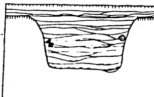
AGGRADING BRAIDED SANDY CHANNEL
