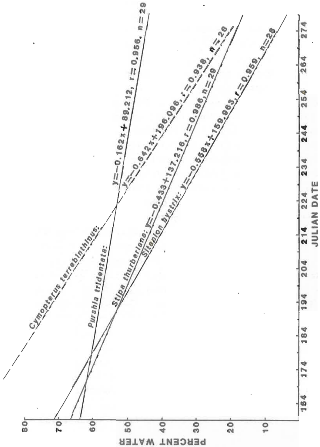
Figure 5.1.2 Percent water in forage, Craters of the Moon National Monument, Idaho.
