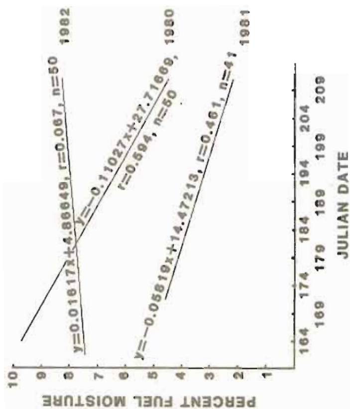
Figure 2.5.1 Percent fuel moisture, 1980-1982, Craters of the Moon National Monument, Idaho.
