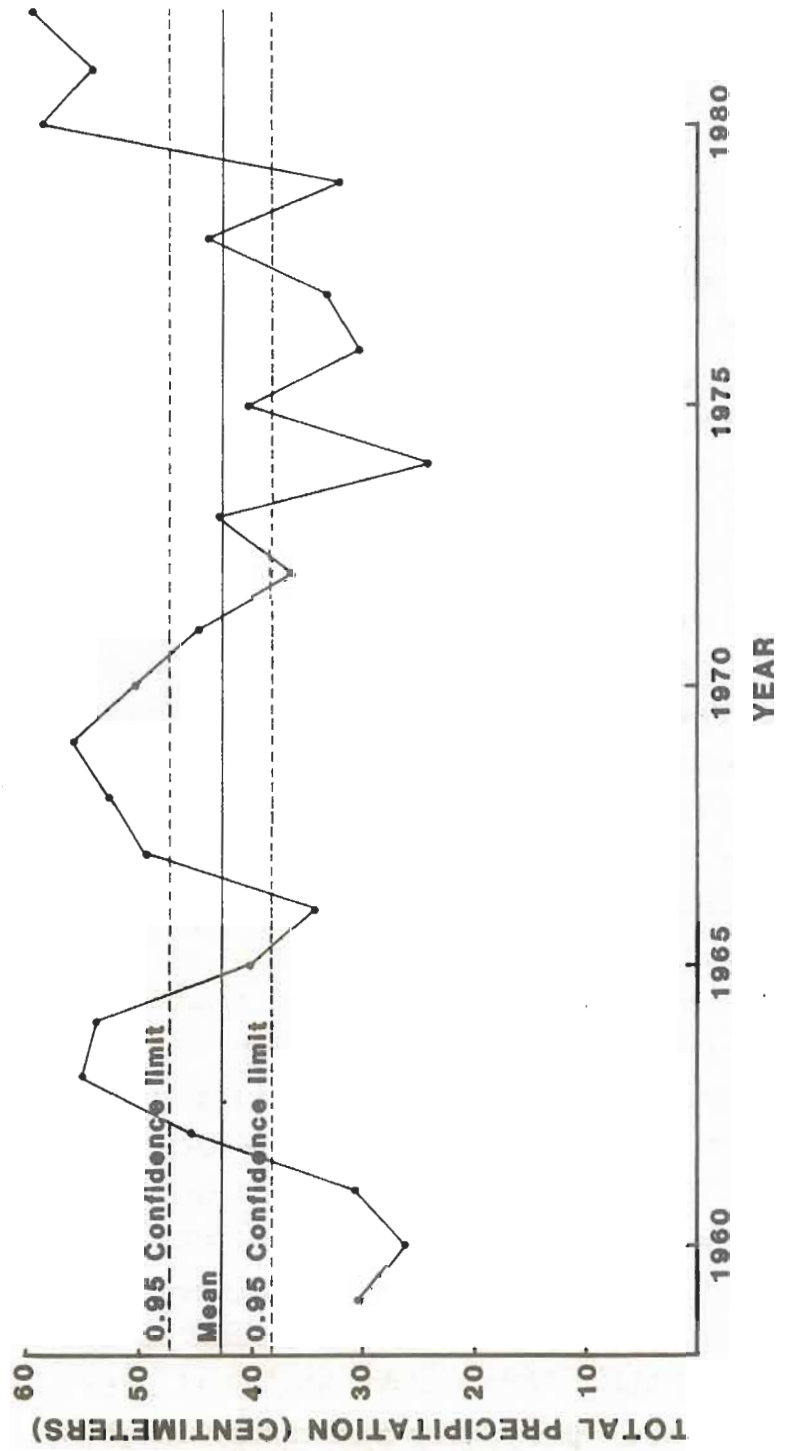
Figure 5.2.1 Total yearly precipitation, 1959-1982, Craters of the Moon National Monument, Idaho.
