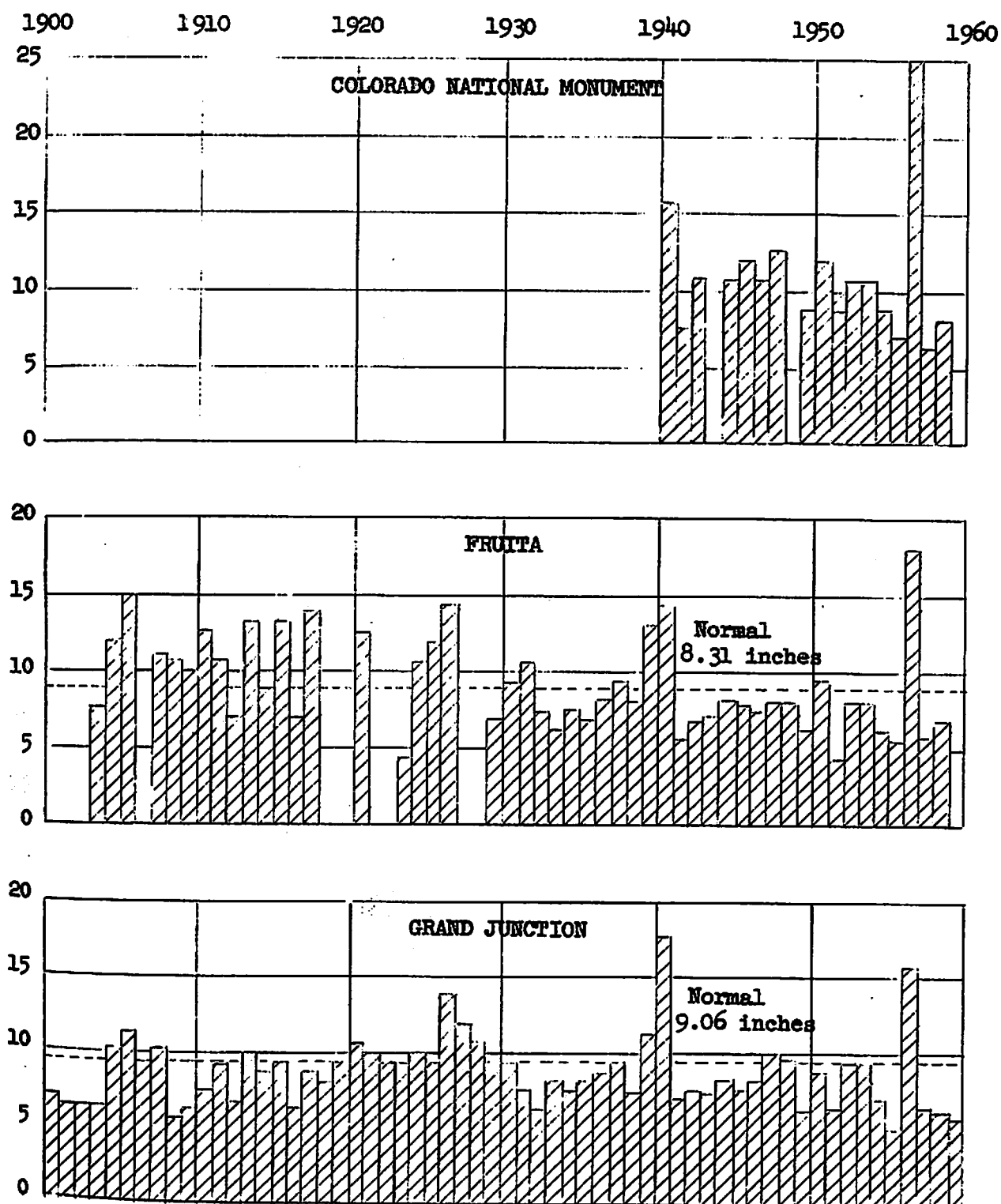
Fig. 3. Precipitation, in inches. From U. S. Weather Bureau Records
