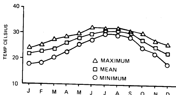
Figure 8. Monthly minimum, mean, and maximum seawater temperature at Sand Key, 1878-1890 (Vaughan 1918).
