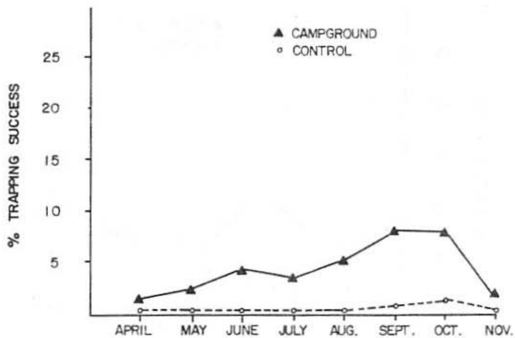
Figure 9. Trapping success for Neotoma spp., Squaw Flat Campground, Canyonlands National Park, Utah (1975).
