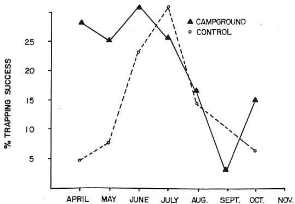
Figure 4. Trapping success for Peromyscus spp., Devil's Garden Campground, Arches National Park, Utah (1975).
