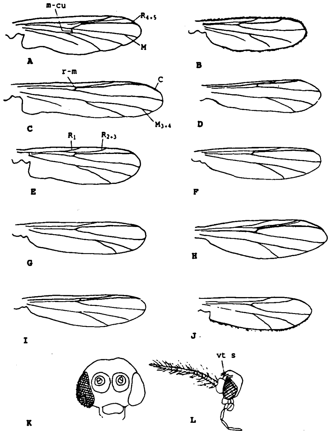
Figure 2.4. Wings and details of male chironomid heads; wing of (A) Diamesa sp.; (B) Eukiefferiella claripennis ; (C) Metriocnemus sp.; (D) Paraphaenocladus exagitans ; (E) Orthocladus rivicola ; (F) Parakiefferiella sp.; (G) Pseudosmittia sp.; (H) Chironomus sp.; (I) Micropsectra sp.; (J) Polypedilum obelos ; (K) anterior view of head with flagellum removed; (L) lateral view of head (A,G,I,K,L) redrawn from McAlpine et al. (1981).
