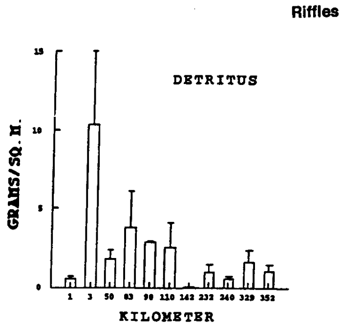
Figure 3.11. Annual summary of spatial variation in detritus ( \text{gm/m}^2 , SE) in pools and riffles in the Colorado River, Arizona during 1991. Note difference in scale between pools and riffles.
