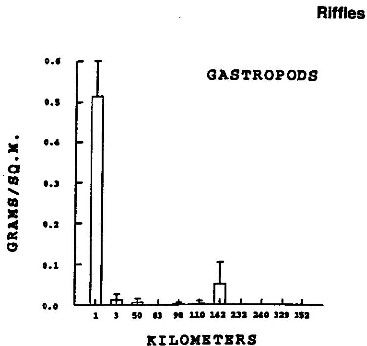
Figure 3.16. Annual summary of spatial variation in gastropod biomass (gm/m 2 , SE) in pools and riffles in the Colorado River, Arizona during 1991.
