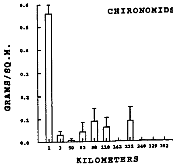
Figure 3.14. Annual summary of spatial variation in chironomid biomass (gm/m 2 , SE) in pools and riffles in the Colorado River, Arizona during 1991.
