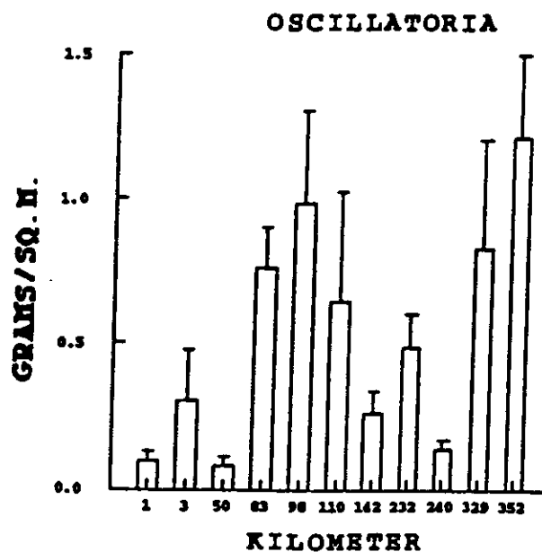
Figure 3.10. Annual summary of spatial variation in Oscillatoria spp. biomass (gm/m 2 , SE) in pools and riffles in the Colorado River, Arizona during 1991. Note difference in scale between pools and riffles.
