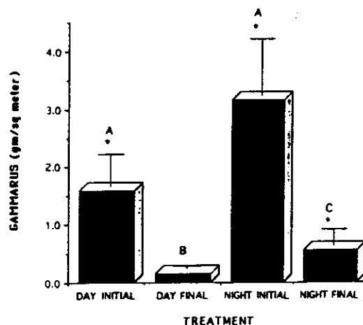
Figure 5.1 Initial and final average dry weight biomass (gm/2; SE) for Cladophora glomerata , chironomids, and Gammarus lacustris after repeated day and night 12-hr experimental exposures for 5 days at Lees Ferry, Arizona, during June 1-5, 1991 (Experiment I). Letters above histograms are significantly different at <0.05 (*) and <0.01 (**) for univariate contrasts.
