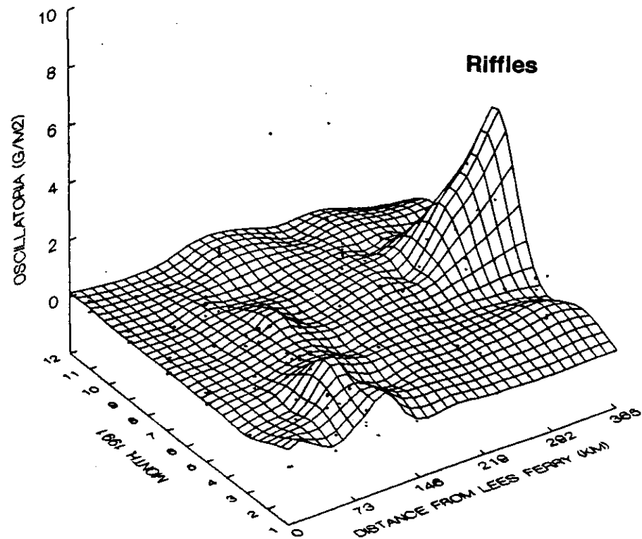
Figure 3.7. Temporal and spatial variation in Oscillatoria spp. biomass (gm/m 2 ) in pools and riffles in the Colorado River, Arizona during 1991. Note difference in scale between pools and riffles.
