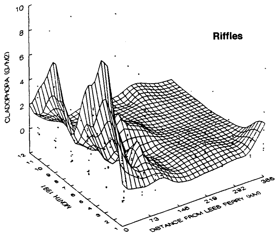
Figure 3.6. Temporal and spatial variation in Cladophora glomerata biomass ( \text{gm}/\text{m}^2 ) in pools and riffles in the Colorado River, Arizona during 1991.
