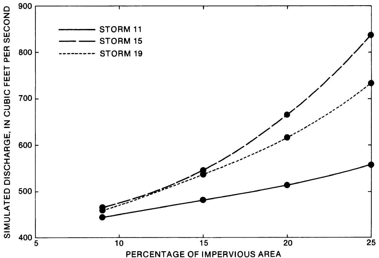
Figure 17.--Simulated peak discharge of Valley Creek at the Pennsylvania Turnpike bridge for storms 11, 15, and 19 with increased impervious area in the Valley Creek basin.
