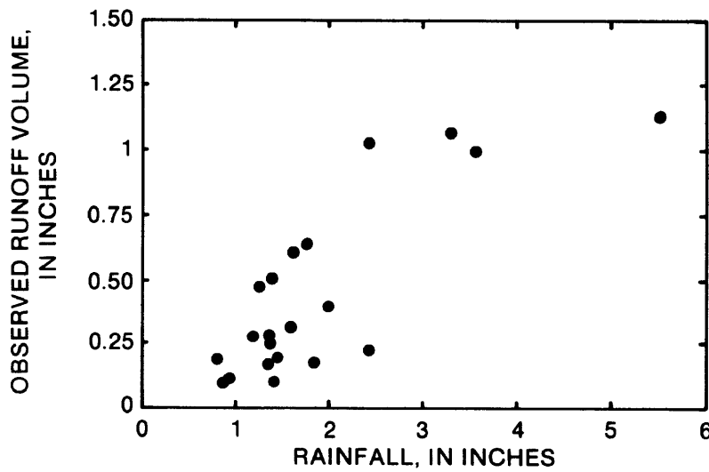
Figure 6.-- Relation between rainfall and observed runoff volume.
