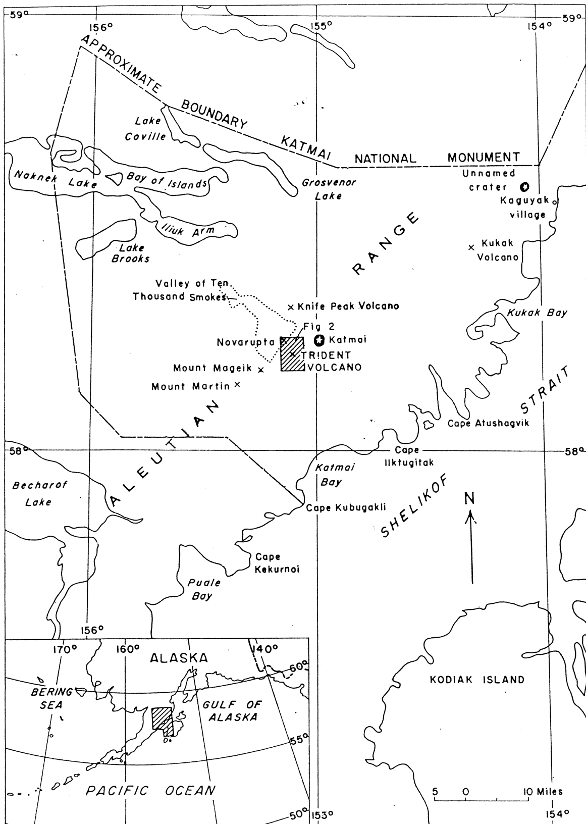
Figure 1. —Location map of Trident Volcano in Katmai National Monument, Alaska.
