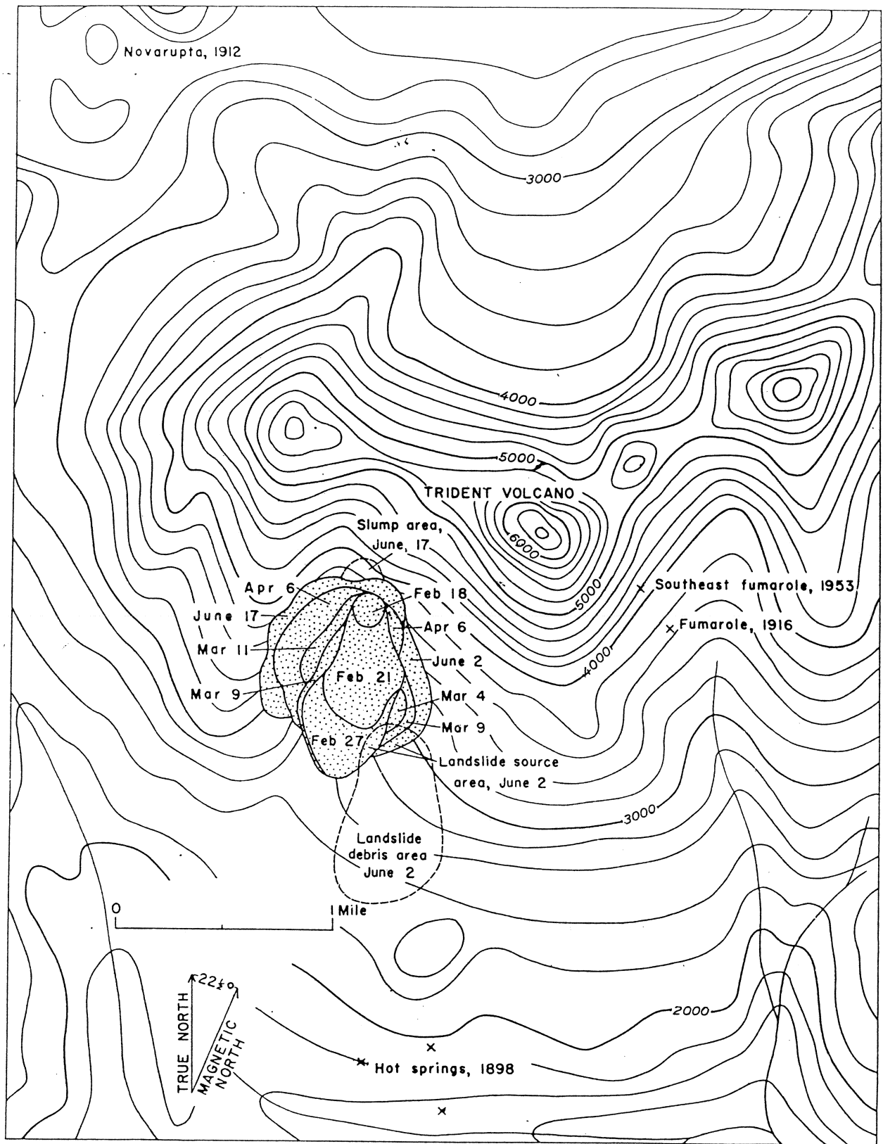
Figure 2. —Sketch map of lava flow from Trident Volcano, February-June, 1953.
